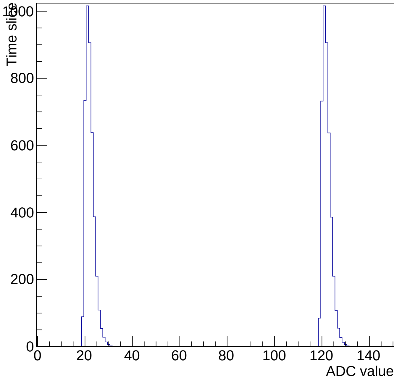
Evt 10 Time mcm 2002 chip 2 chan 2 pulser-10V-wire20-135
