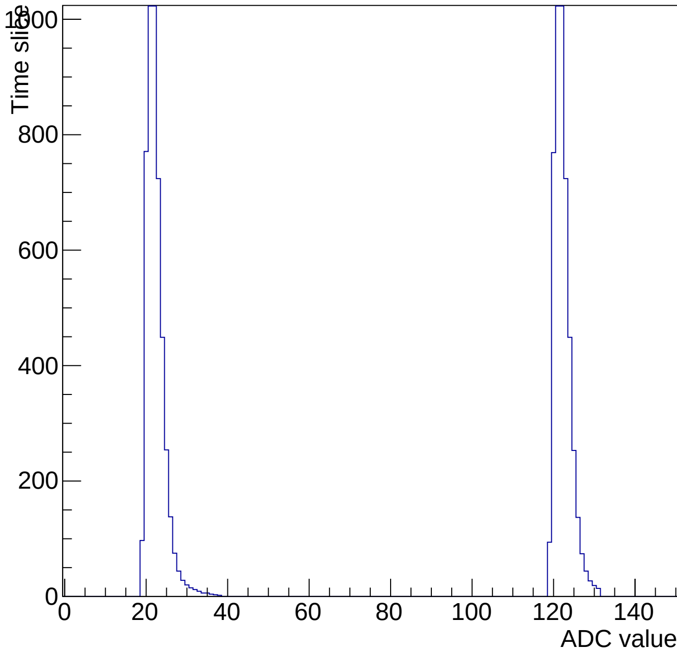
Evt 10 Time mcm 2002 chip 2 chan 1 pulser-10V-wire20-135
