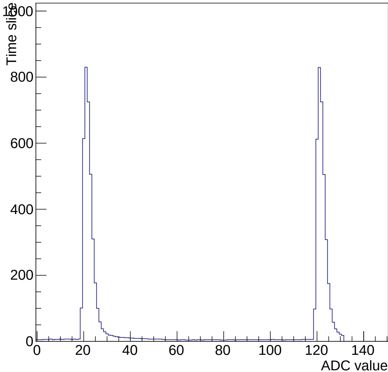
Evt 10 Time mcm 2002 chip 2 chan 5 pulser-10V-wire20-135
