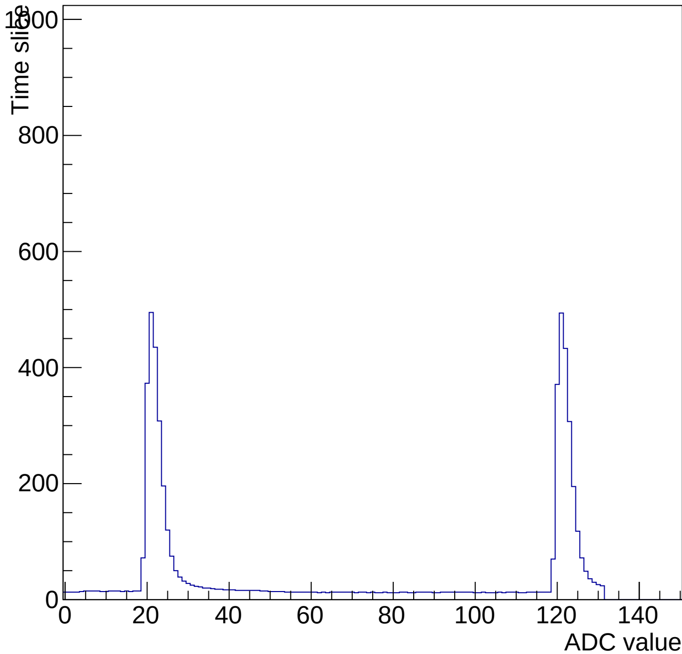
Evt 10 Time mcm 2002 chip 2 chan 11 pulser-10V-wire20-135
