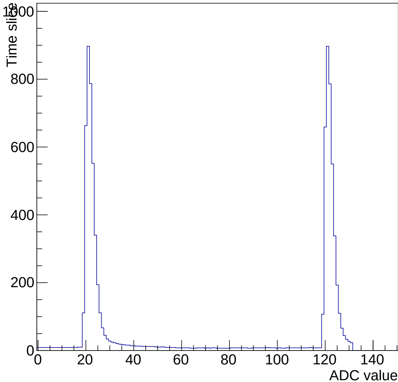
Evt 10 Time mcm 2002 chip 2 chan 4 pulser-10V-wire20-135
