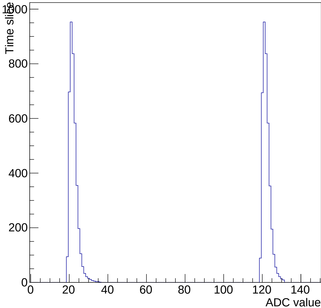
Evt 10 Time mcm 2002 chip 2 chan 3 pulser-10V-wire20-135
