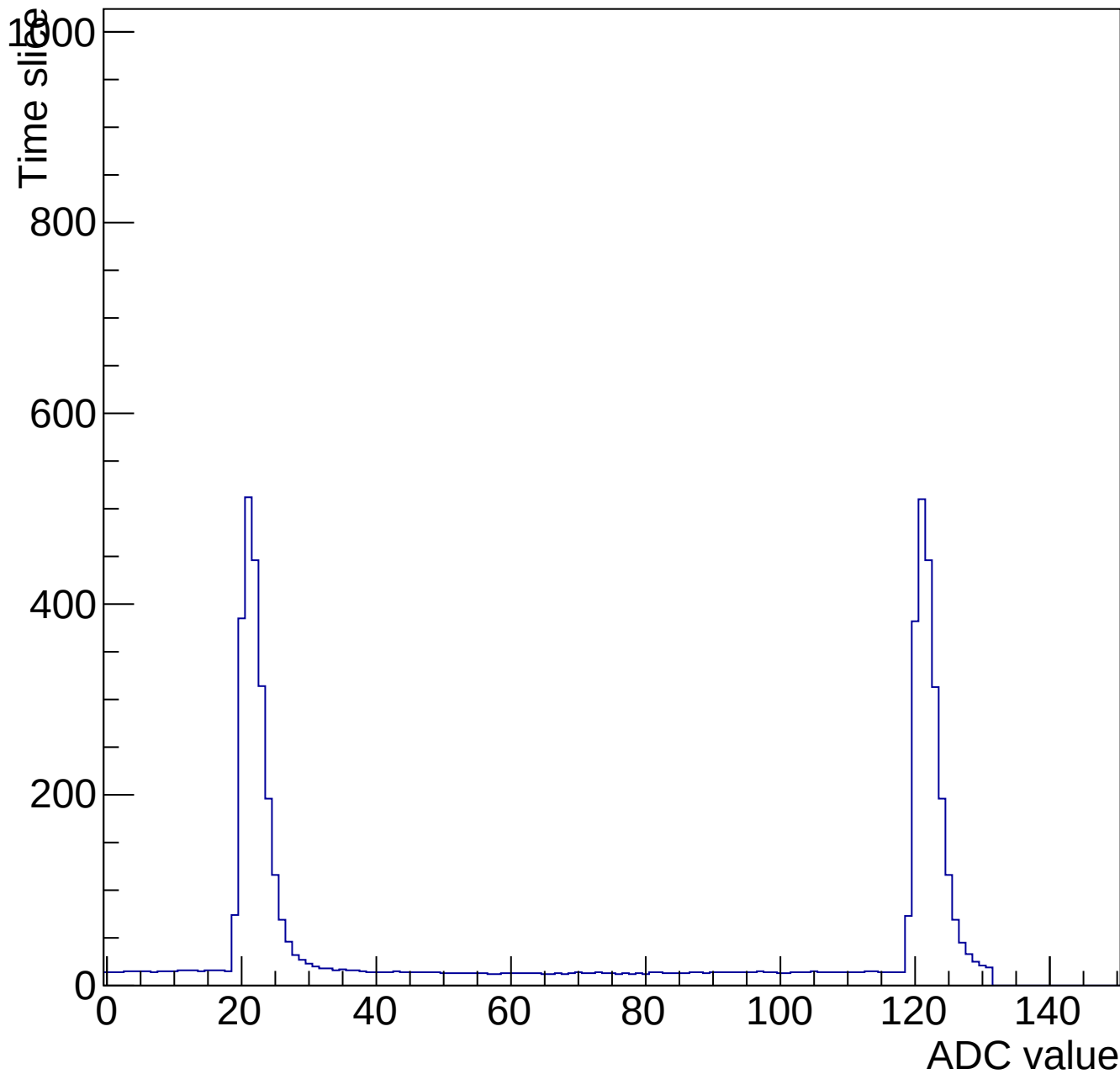
Evt 10 Time mcm 2002 chip 2 chan 10 pulser-10V-wire20-135
