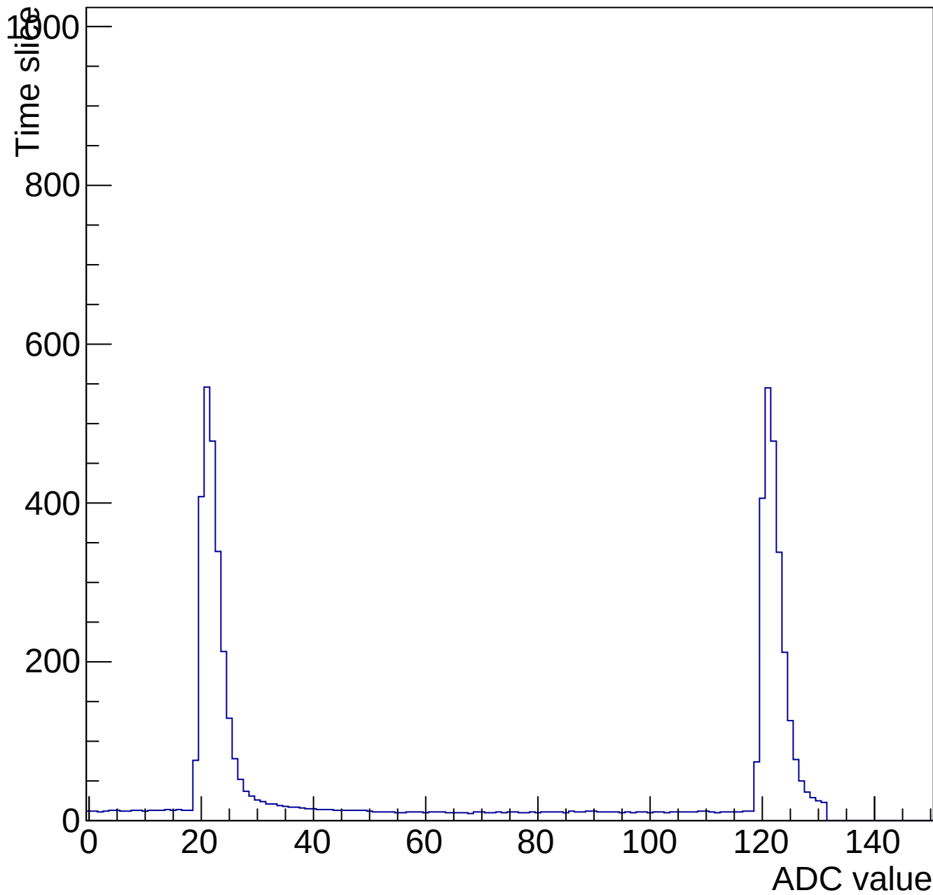
Evt 10 Time mcm 2002 chip 2 chan 9 pulser-10V-wire20-135
