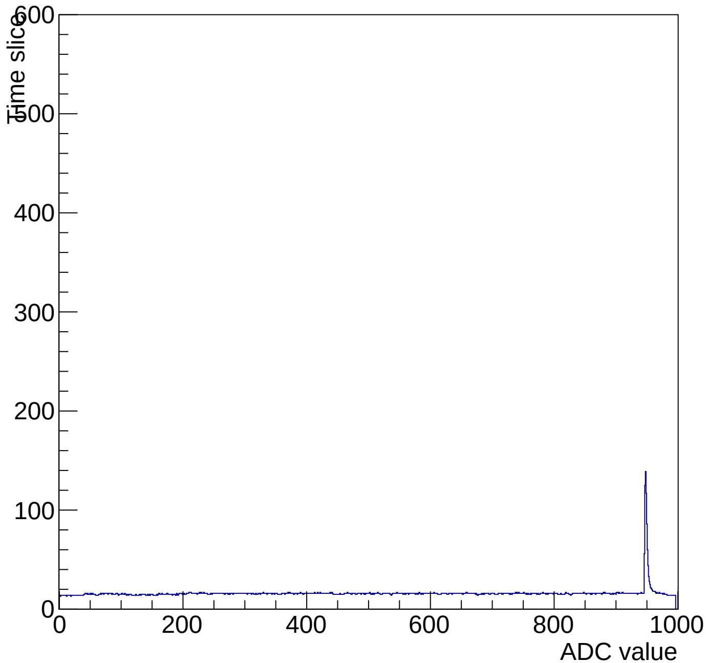
Evt 10 Time mcm 2002 chip 2 chan 15 pulser-10V-wire20
