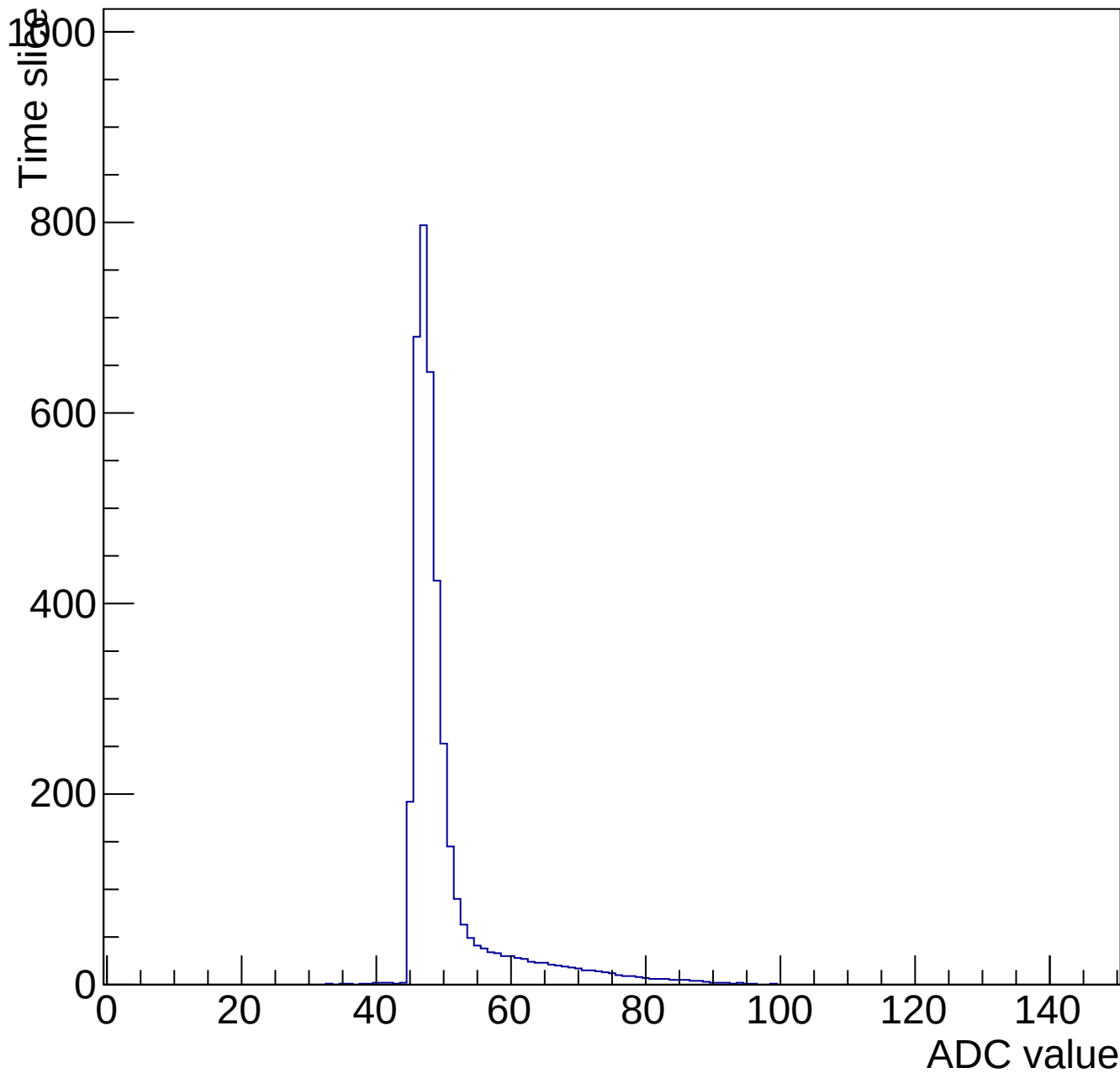
Evt 10 Time mcm 2003 chip 3 chan 10 pulser-10V-wire20-135
