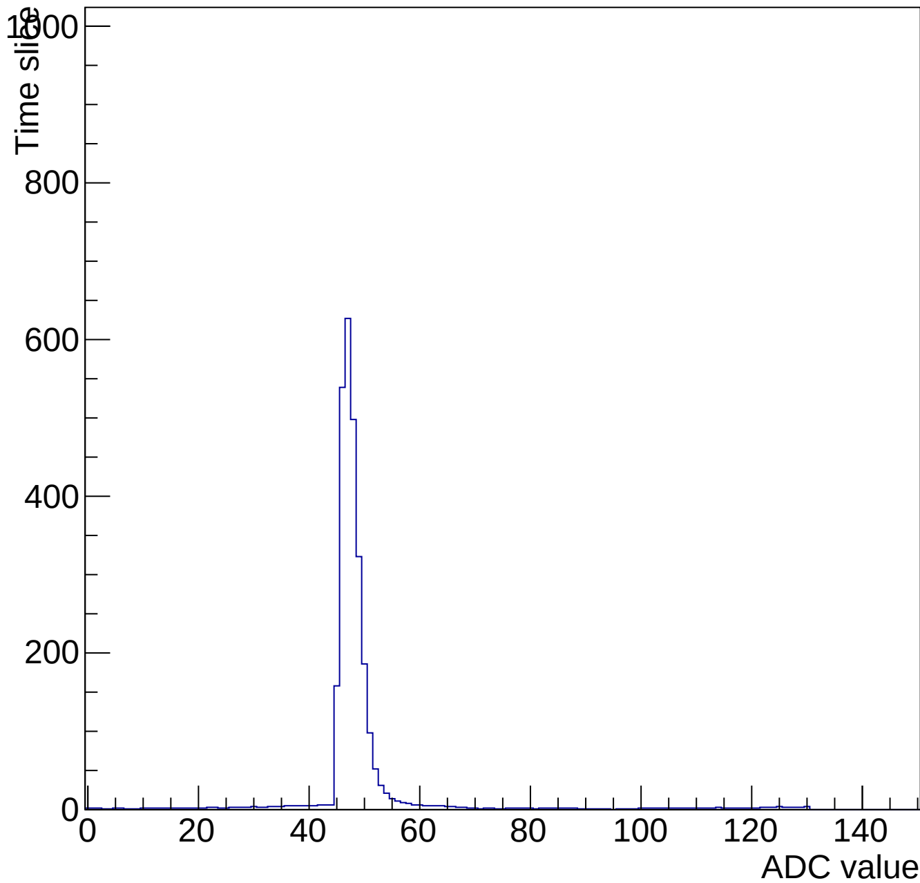
Evt 10 Time mcm 2003 chip 3 chan 15 pulser-10V-wire20-135
