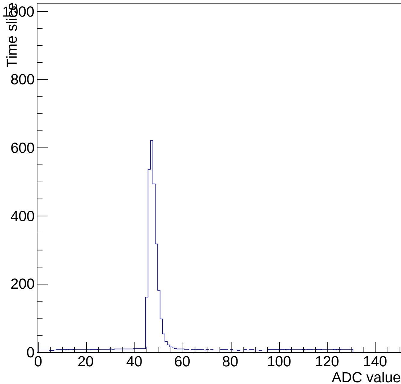
Evt 10 Time mcm 2003 chip 3 chan 11 pulser-10V-wire20-135
