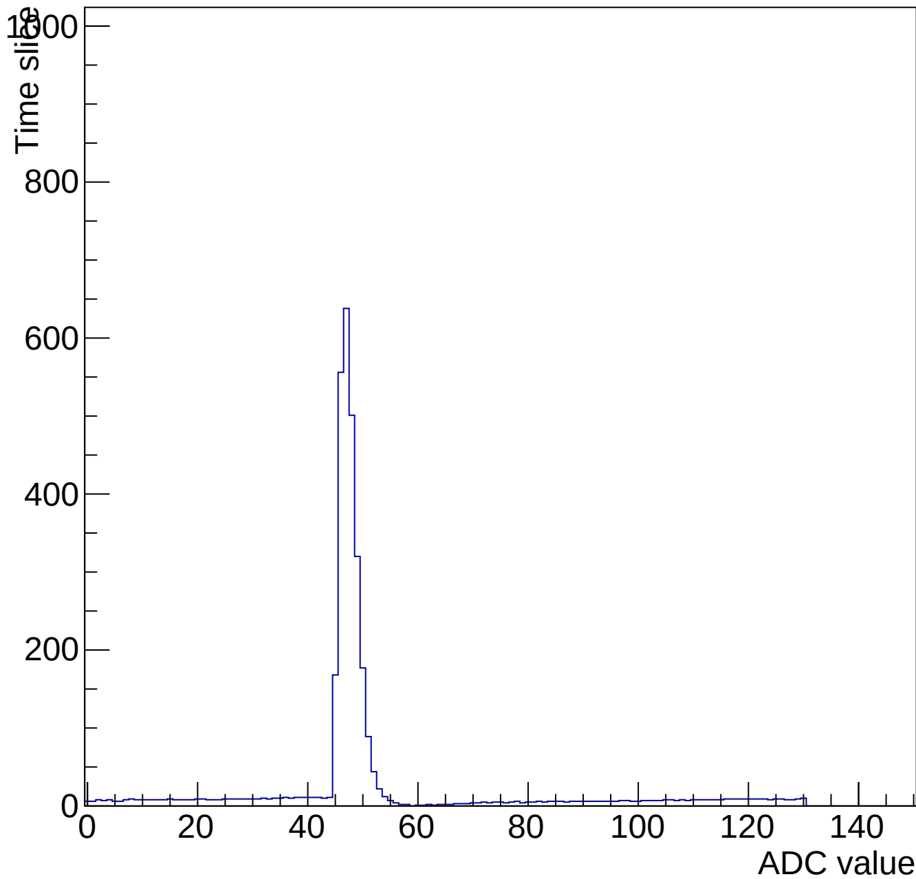
Evt 10 Time mcm 2003 chip 3 chan 13 pulser-10V-wire20-135
