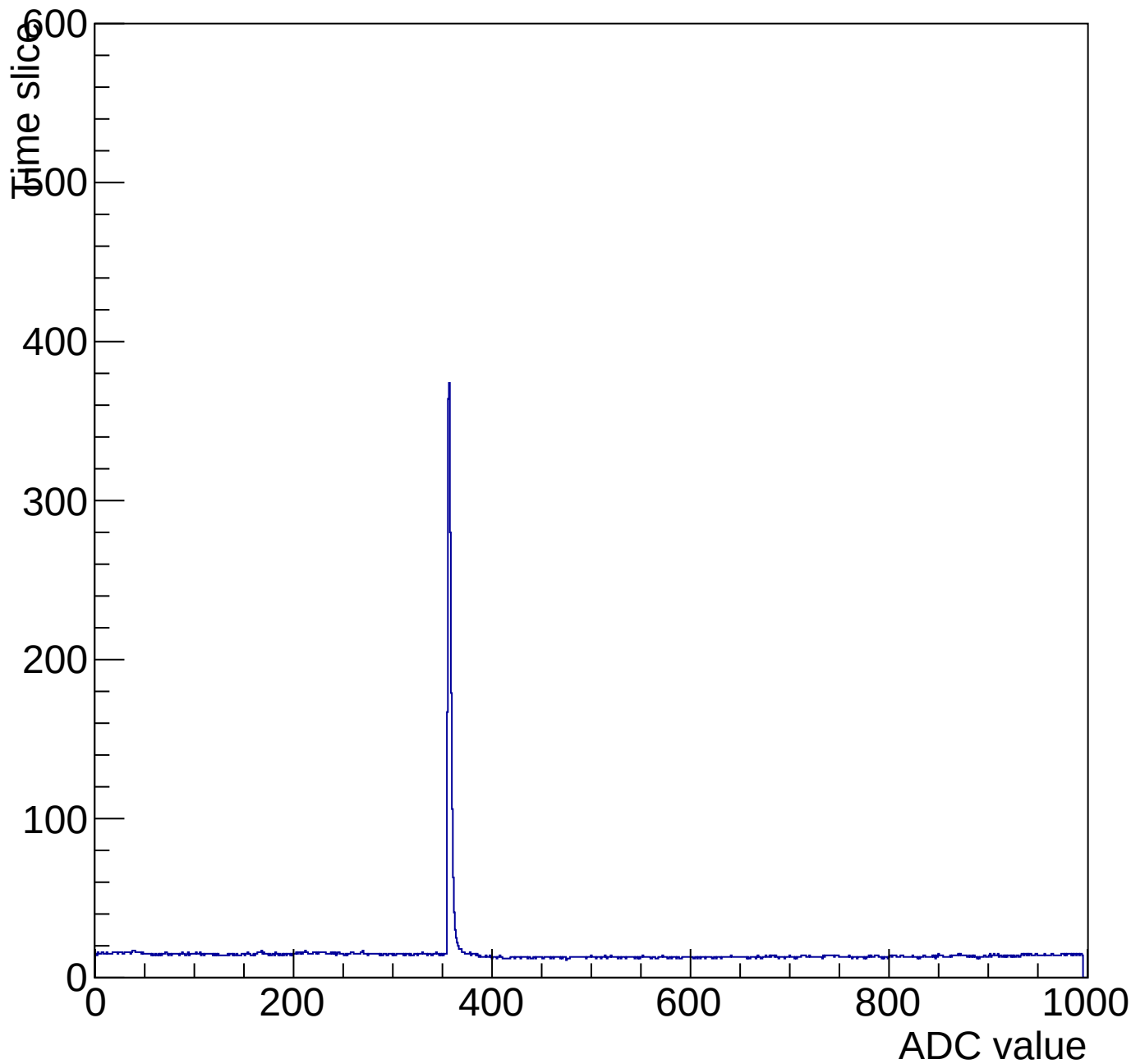
Evt 10 Time mcm 2003 chip 3 chan 3 pulser-6V-wire20
