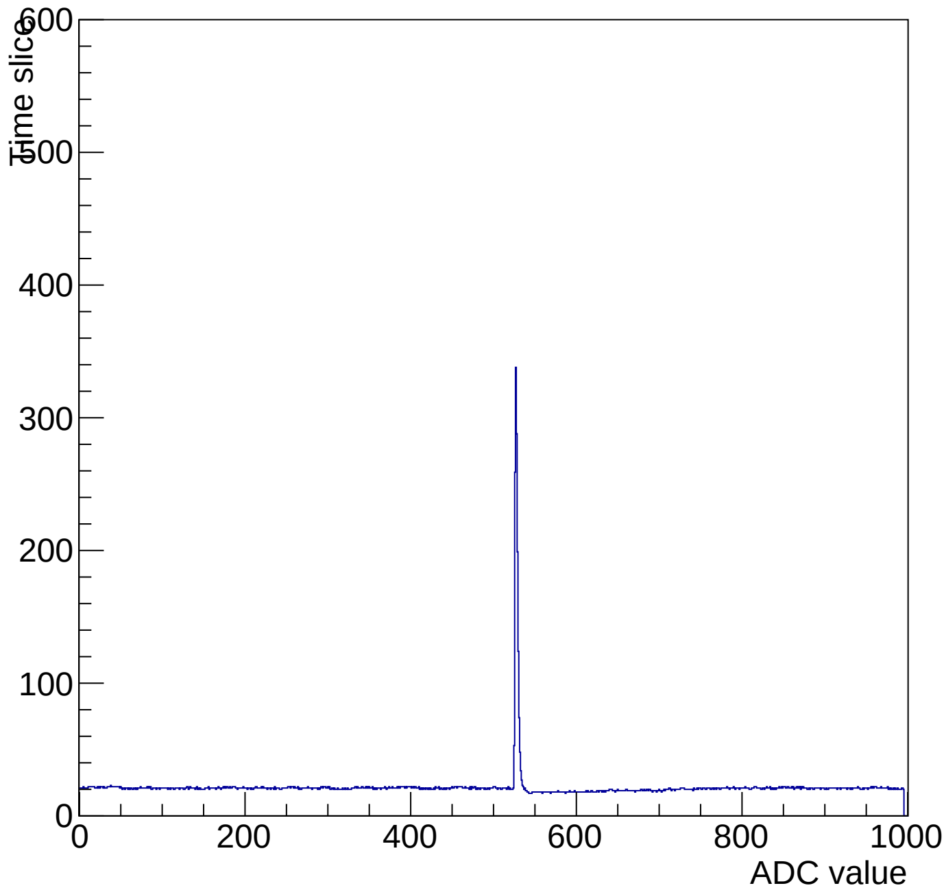
Evt 10 Time mcm 2003 chip 3 chan 11 pulser-6V-wire20
