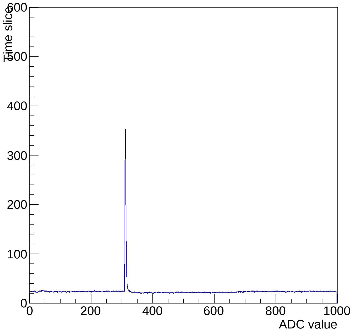
Evt 10 Time mcm 2003 chip 3 chan 5 pulser-6V-wire20
