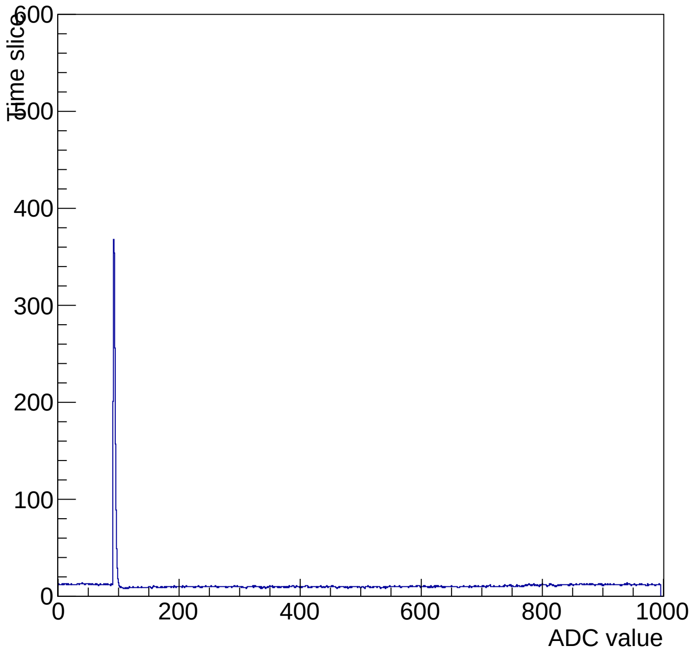
Evt 10 Time mcm 2003 chip 3 chan 12 pulser-6V-wire20
