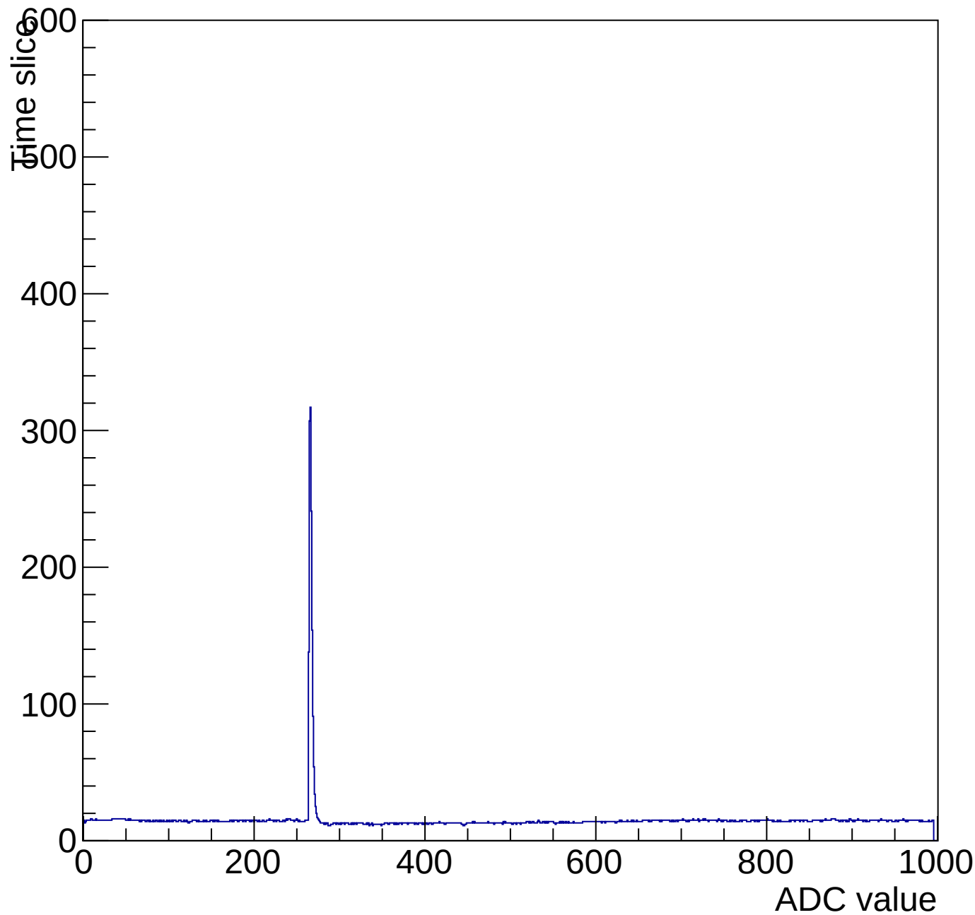
Evt 10 Time mcm 2003 chip 3 chan 7 pulser-6V-wire20
