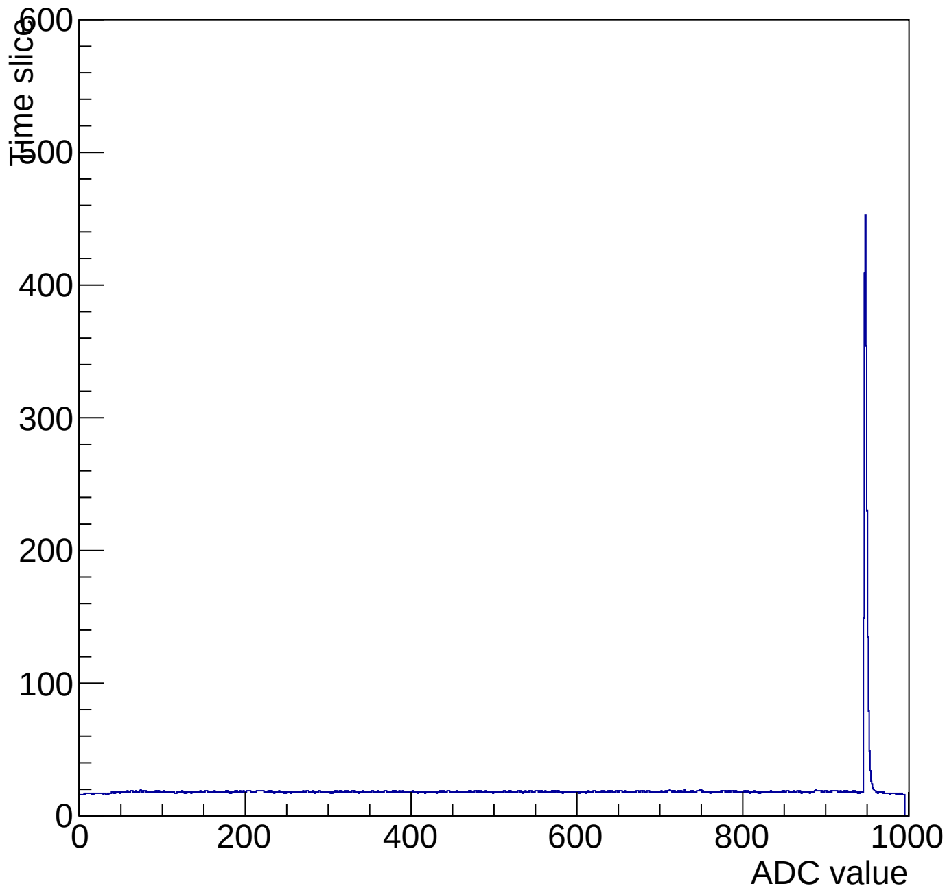
Evt 10 Time mcm 2003 chip 3 chan 8 pulser-6V-wire20
