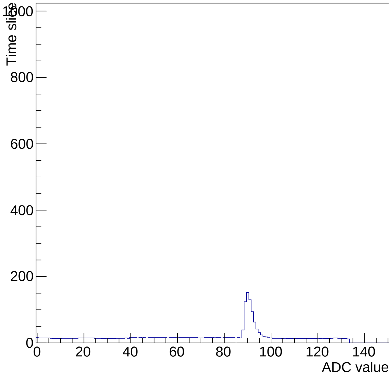
Evt 10 Time mcm 2004 chip 4 chan 10 pulser-10V-wire64-135
