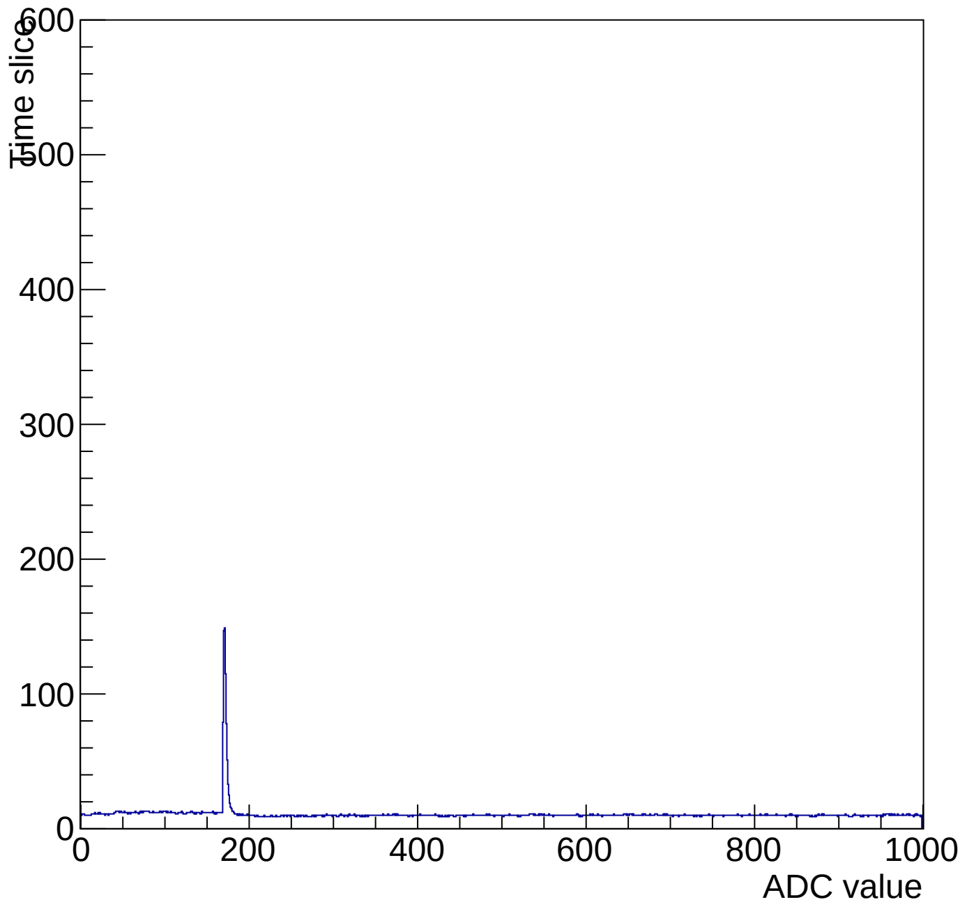
Evt 10 Time mcm 2004 chip 4 chan 15 pulser-10V-wire64
