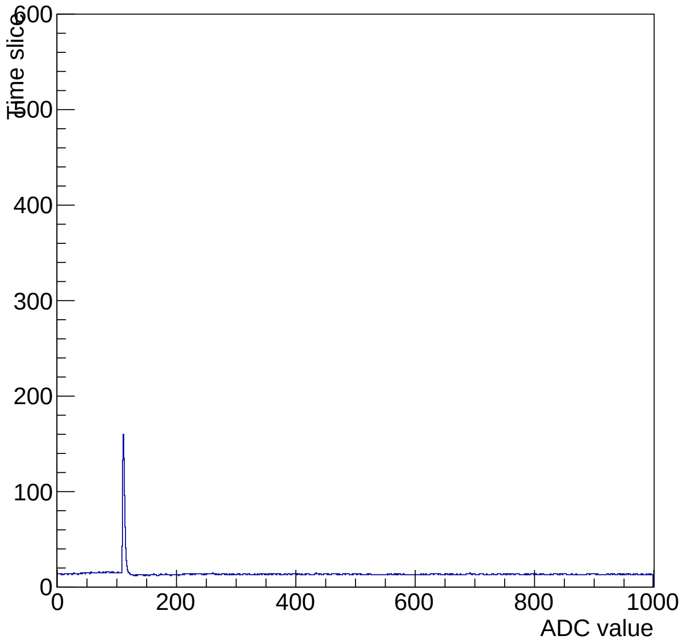
Evt 10 Time mcm 2004 chip 4 chan 13 pulser-10V-wire64
