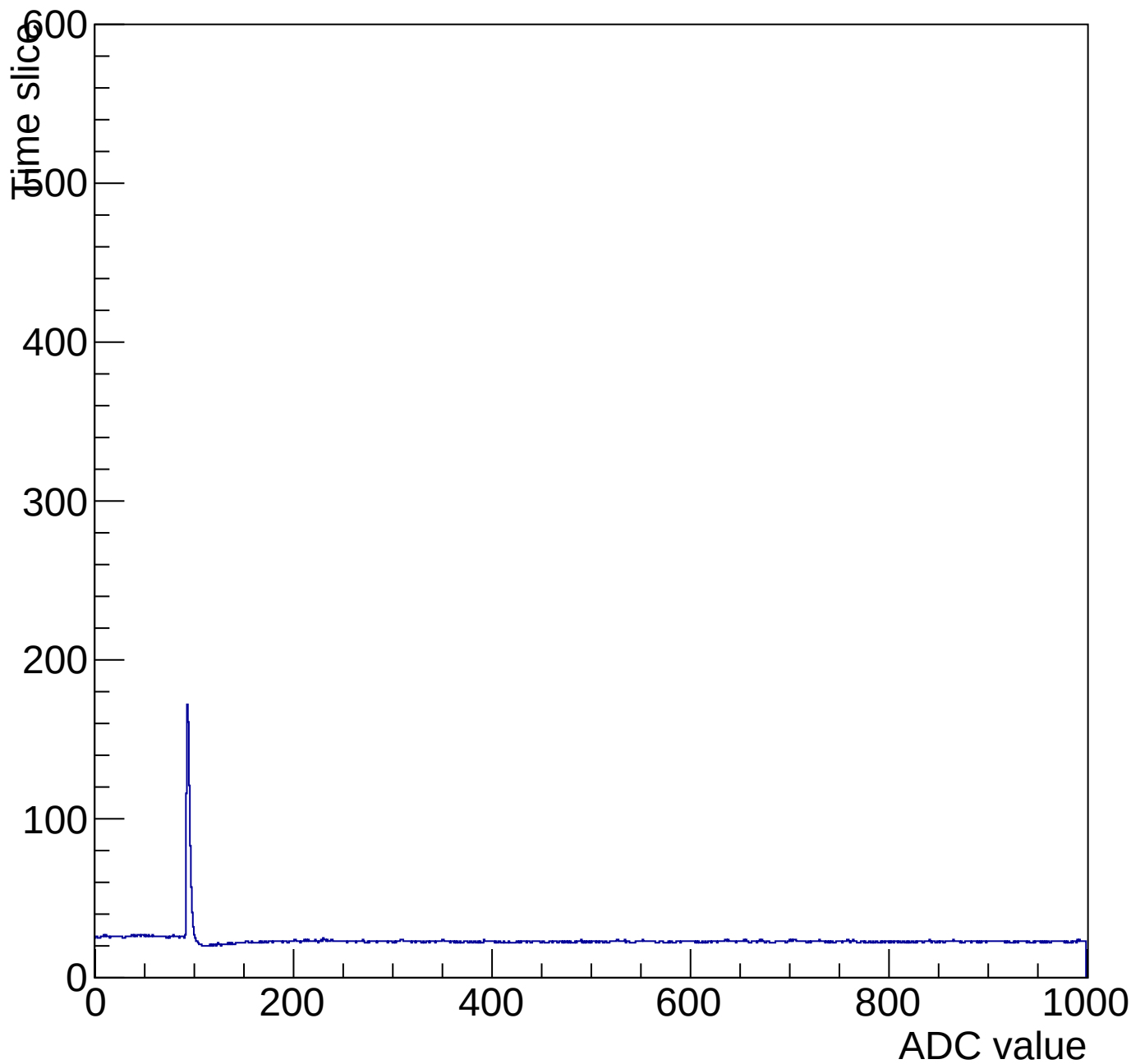
Evt 10 Time mcm 2004 chip 4 chan 11 pulser-10V-wire64
