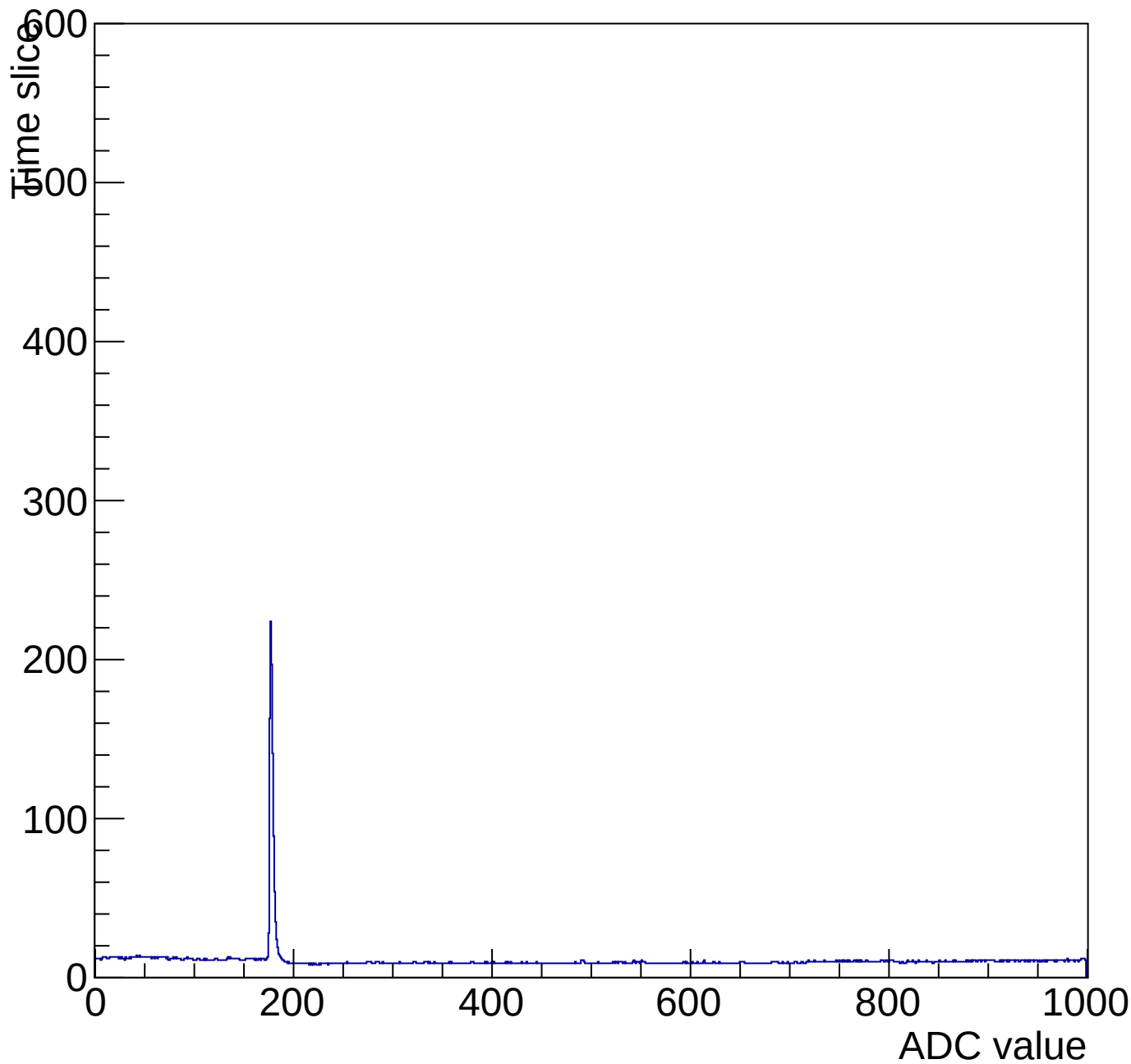
Evt 10 Time mcm 2004 chip 4 chan 1 pulser-10V-wire64
