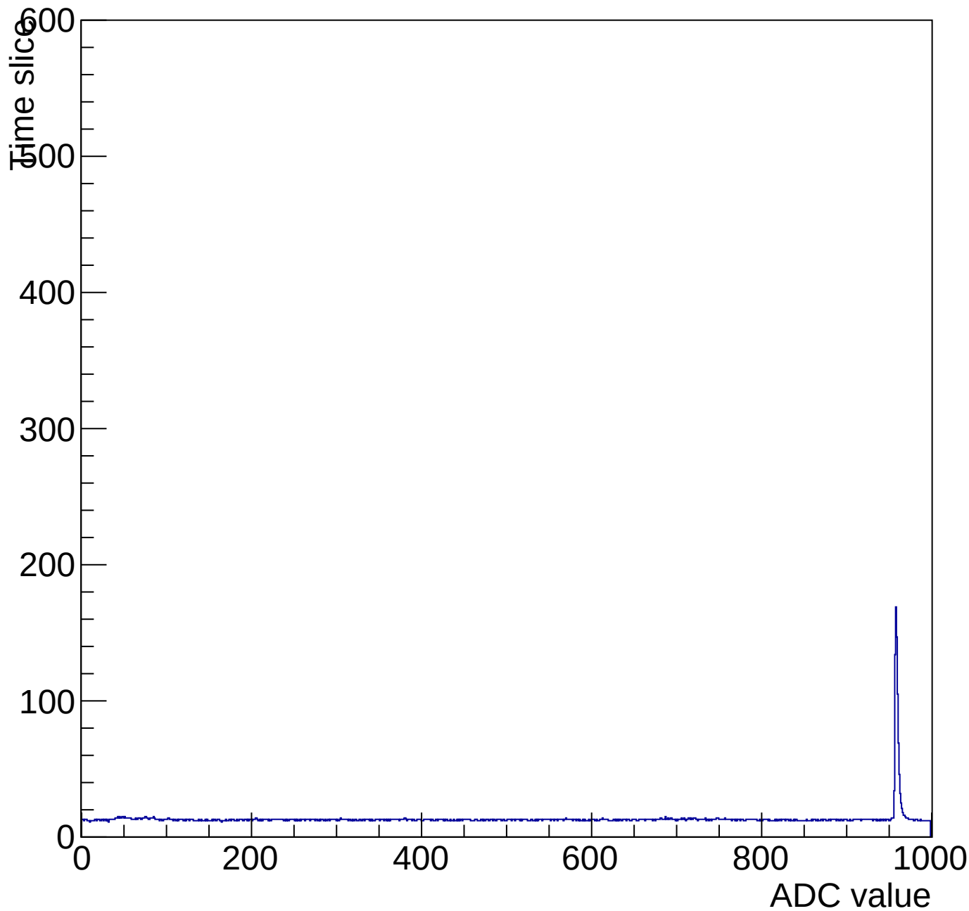
Evt 10 Time mcm 2004 chip 4 chan 8 pulser-10V-wire64
