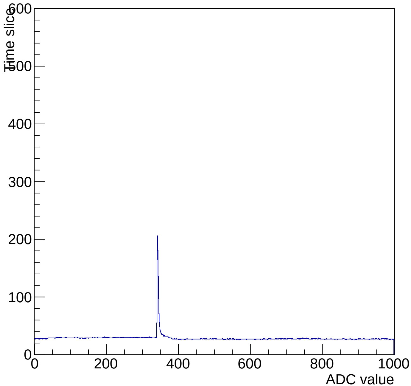
Evt 10 Time mcm 2004 chip 4 chan 7 pulser-10V-wire64
