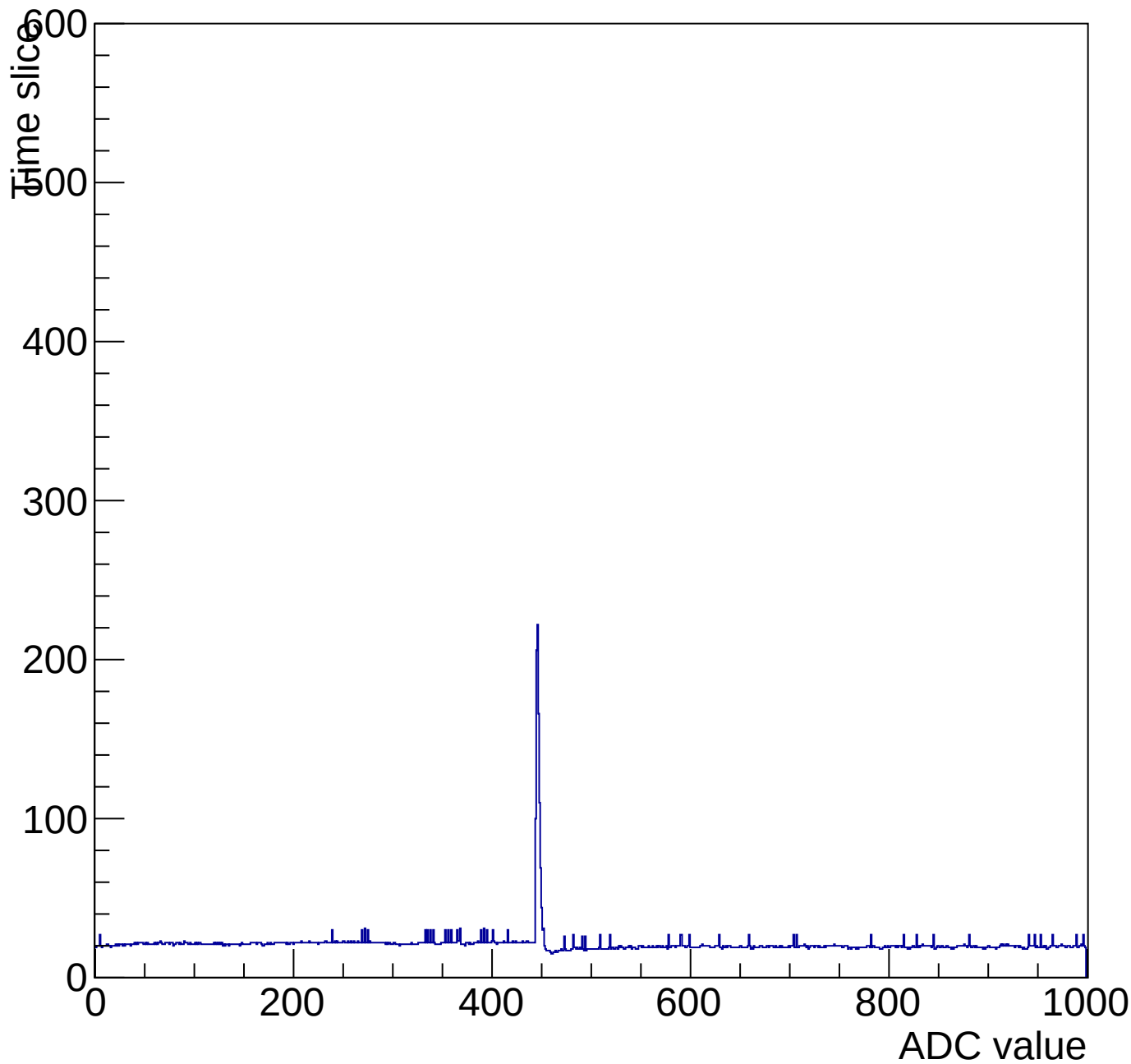
Evt 10 Time mcm 2004 chip 4 chan 2 pulser-10V-wire64
