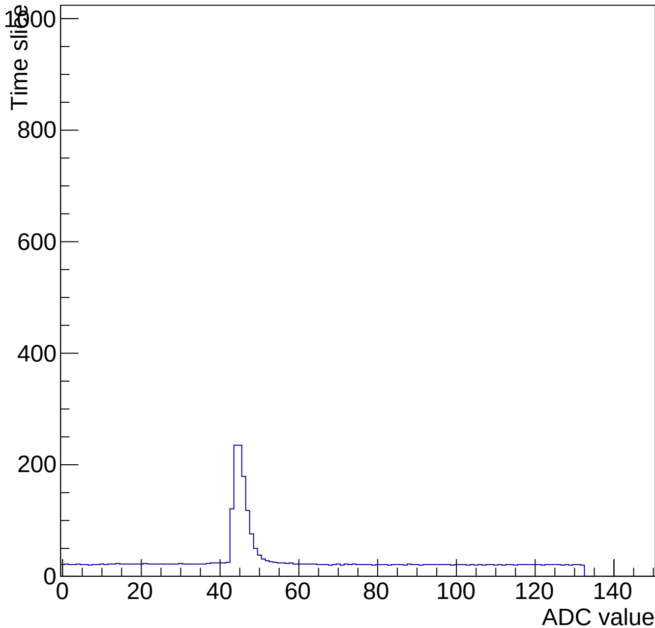
Evt 10 Time mcm 2005 chip 5 chan 1 pulser-10V-wire64-135
