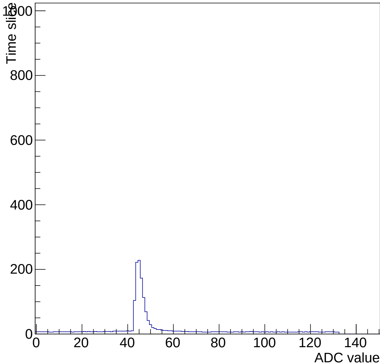
Evt 10 Time mcm 2005 chip 5 chan 13 pulser-10V-wire64-135
