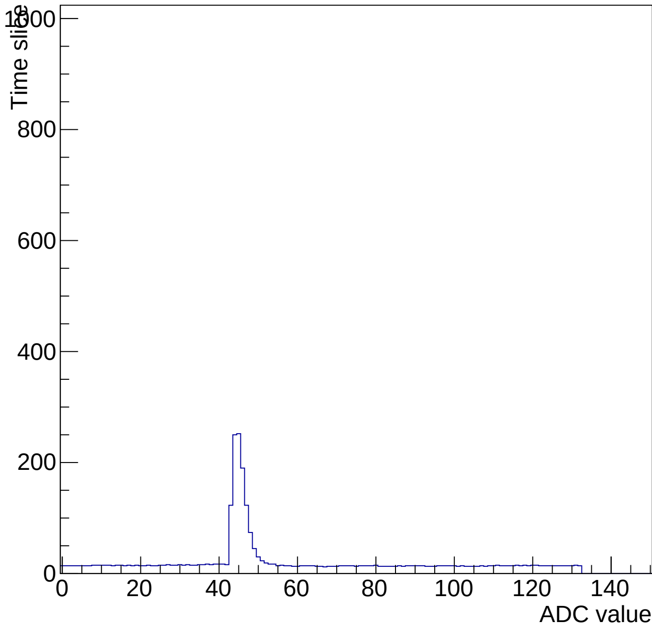
Evt 10 Time mcm 2005 chip 5 chan 10 pulser-10V-wire64-135
