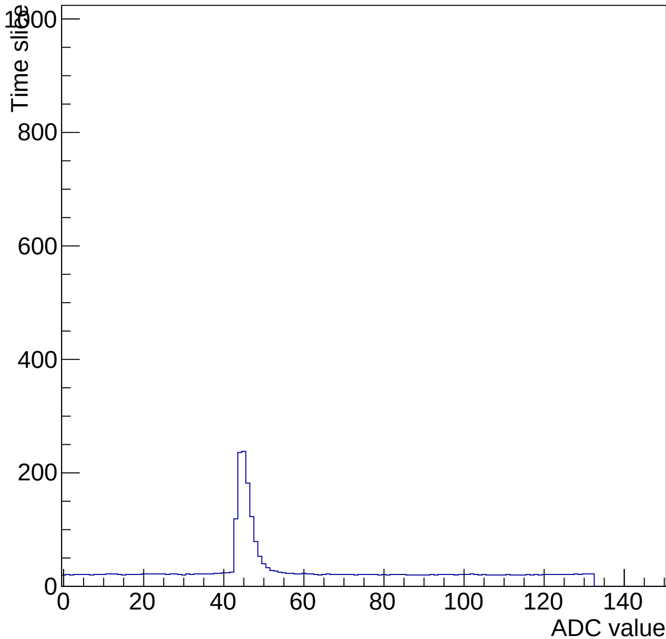
Evt 10 Time mcm 2005 chip 5 chan 6 pulser-10V-wire64-135
