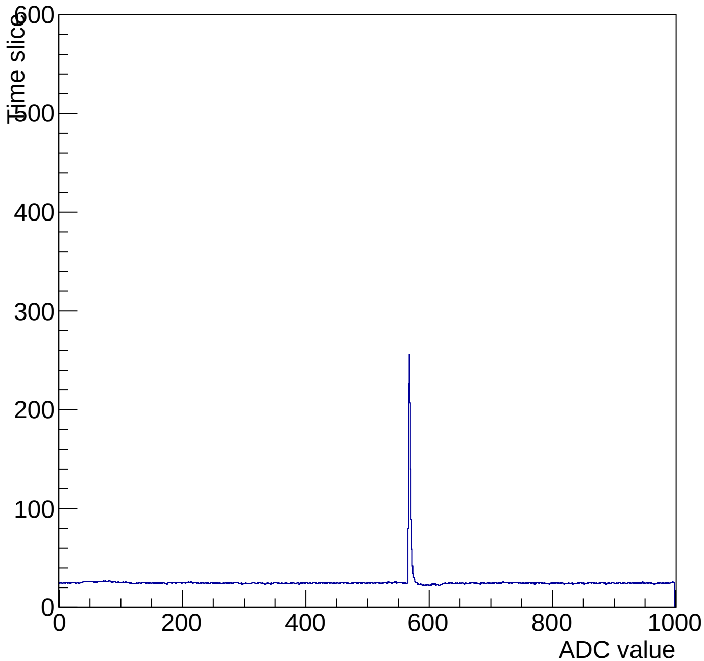
Evt 10 Time mcm 2005 chip 5 chan 1 pulser-10V-wire64
