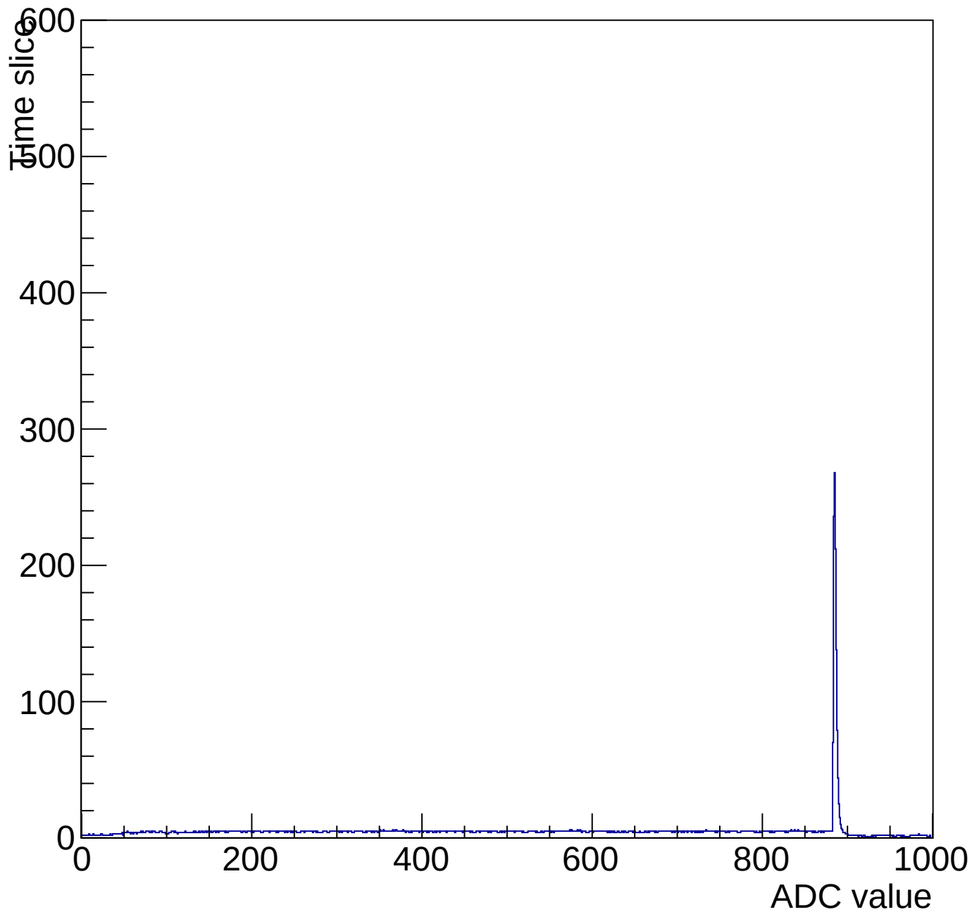
Evt 10 Time mcm 2005 chip 5 chan 12 pulser-10V-wire64
