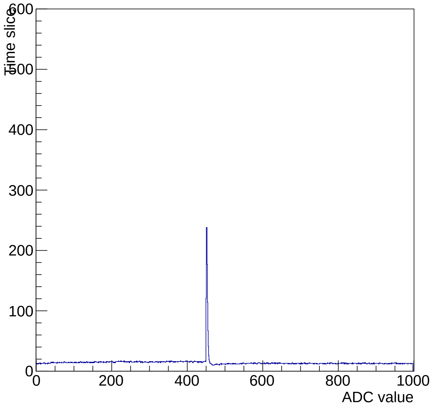
Evt 10 Time mcm 2005 chip 5 chan 15 pulser-10V-wire64
