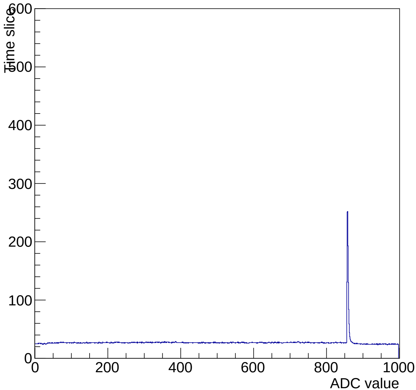
Evt 10 Time mcm 2005 chip 5 chan 6 pulser-10V-wire64
