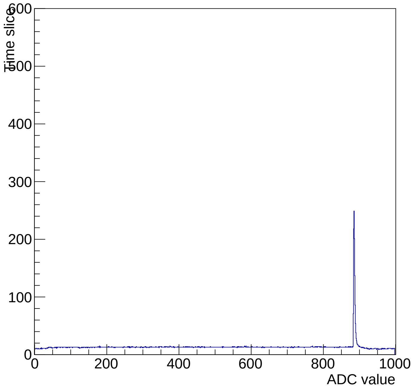
Evt 10 Time mcm 2005 chip 5 chan 13 pulser-10V-wire64
