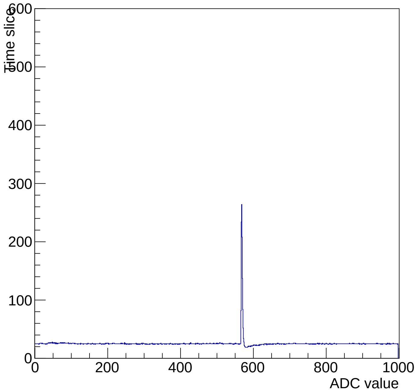
Evt 10 Time mcm 2005 chip 5 chan 0 pulser-10V-wire64
