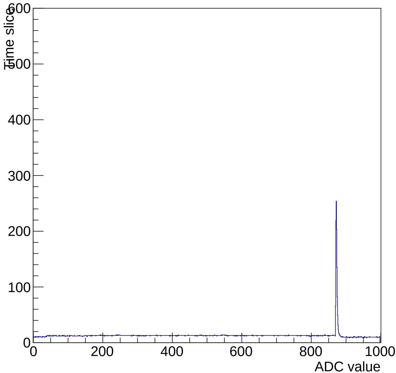
Evt 10 Time mcm 2005 chip 5 chan 4 pulser-10V-wire64
