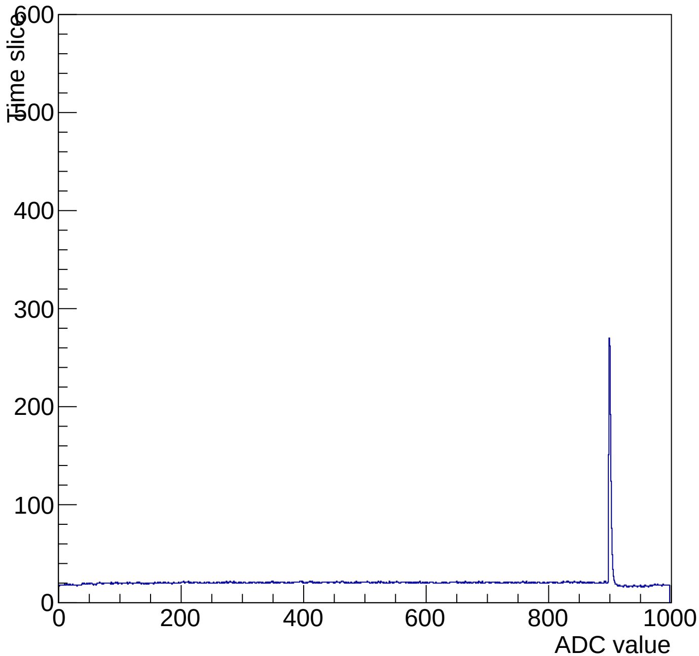
Evt 10 Time mcm 2005 chip 5 chan 10 pulser-10V-wire64
