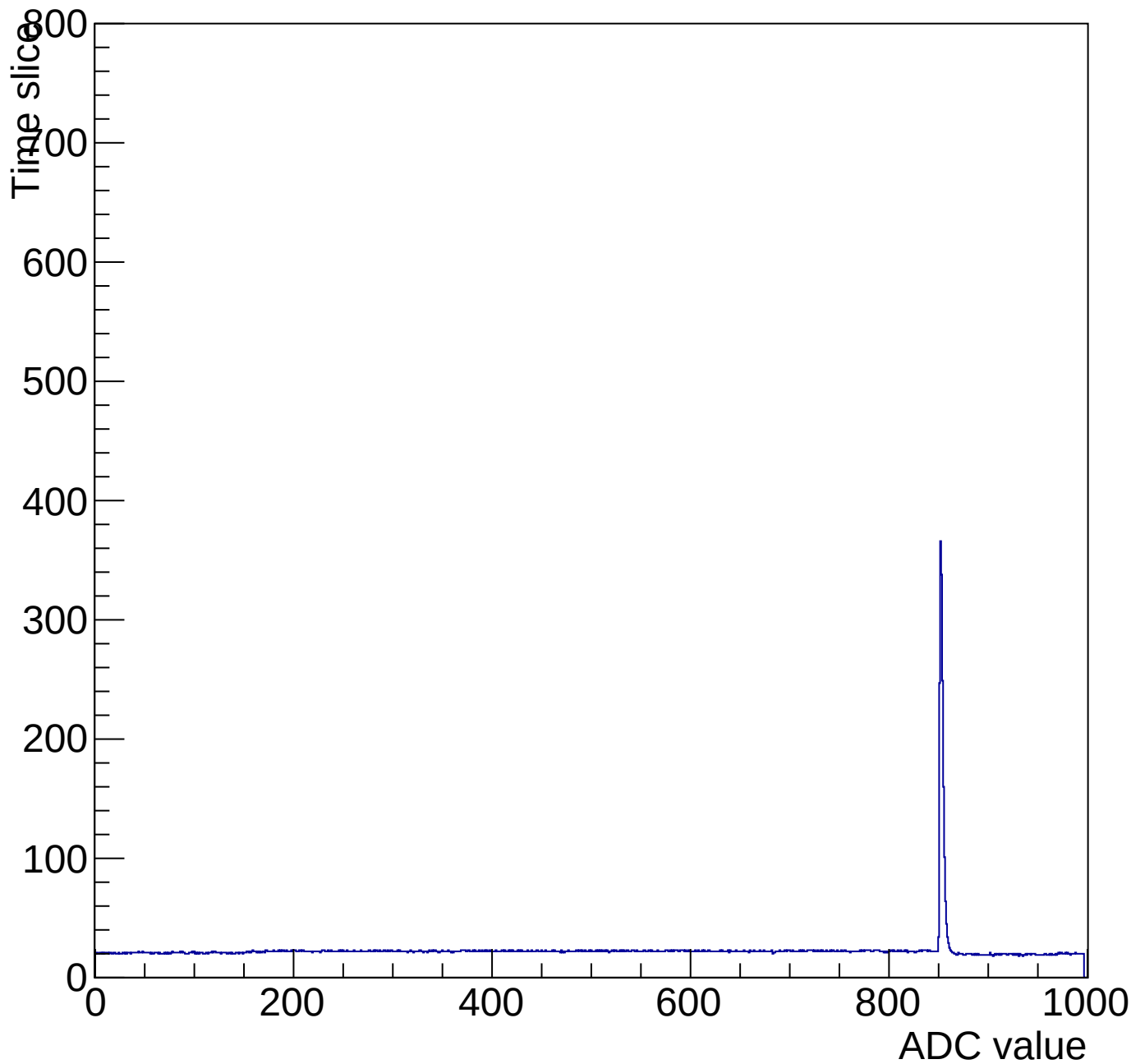
Evt 10 Time mcm 2006 chip 6 chan 13 pulser-10V-wire64
