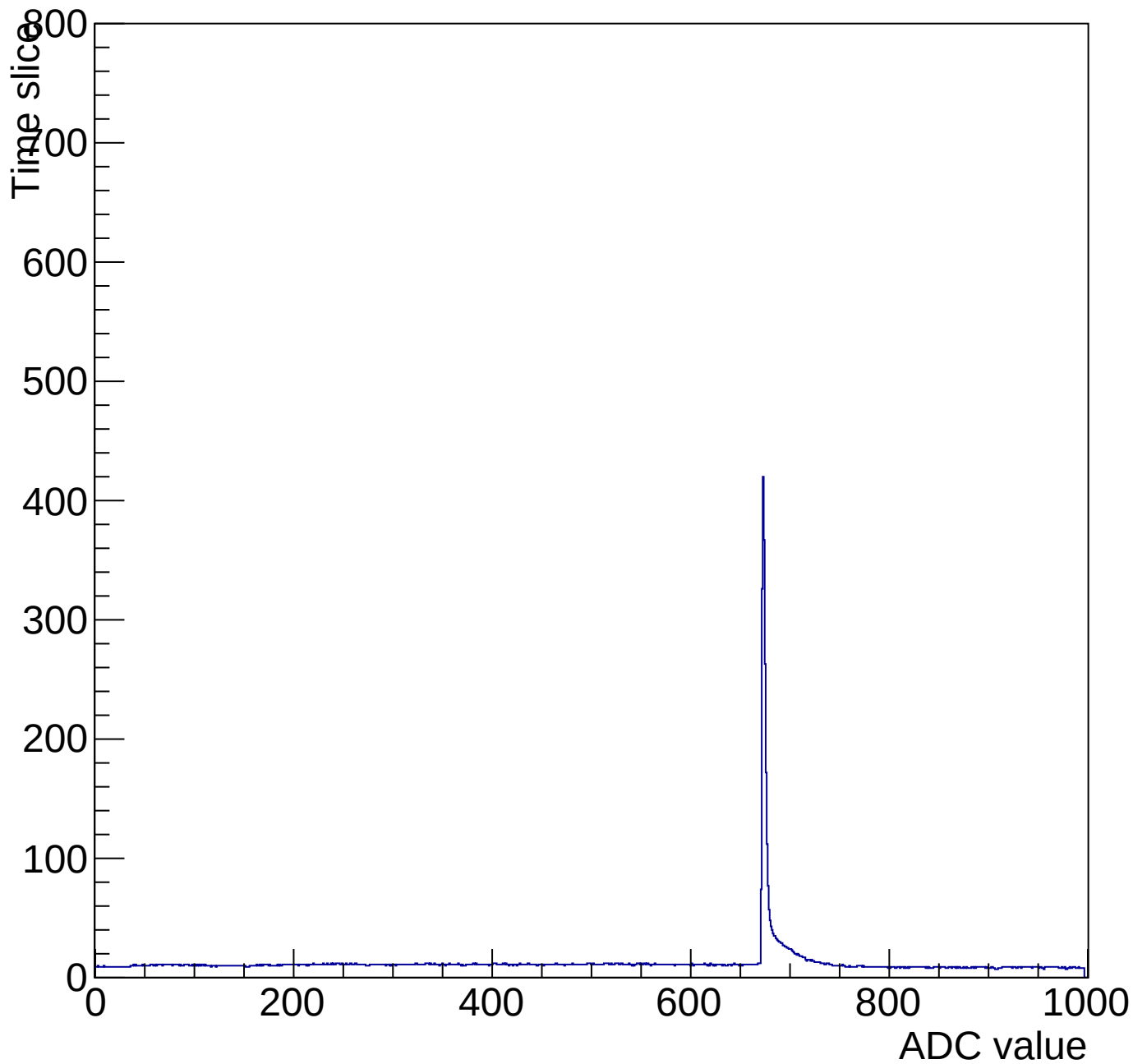
Evt 10 Time mcm 2006 chip 6 chan 6 pulser-10V-wire64
