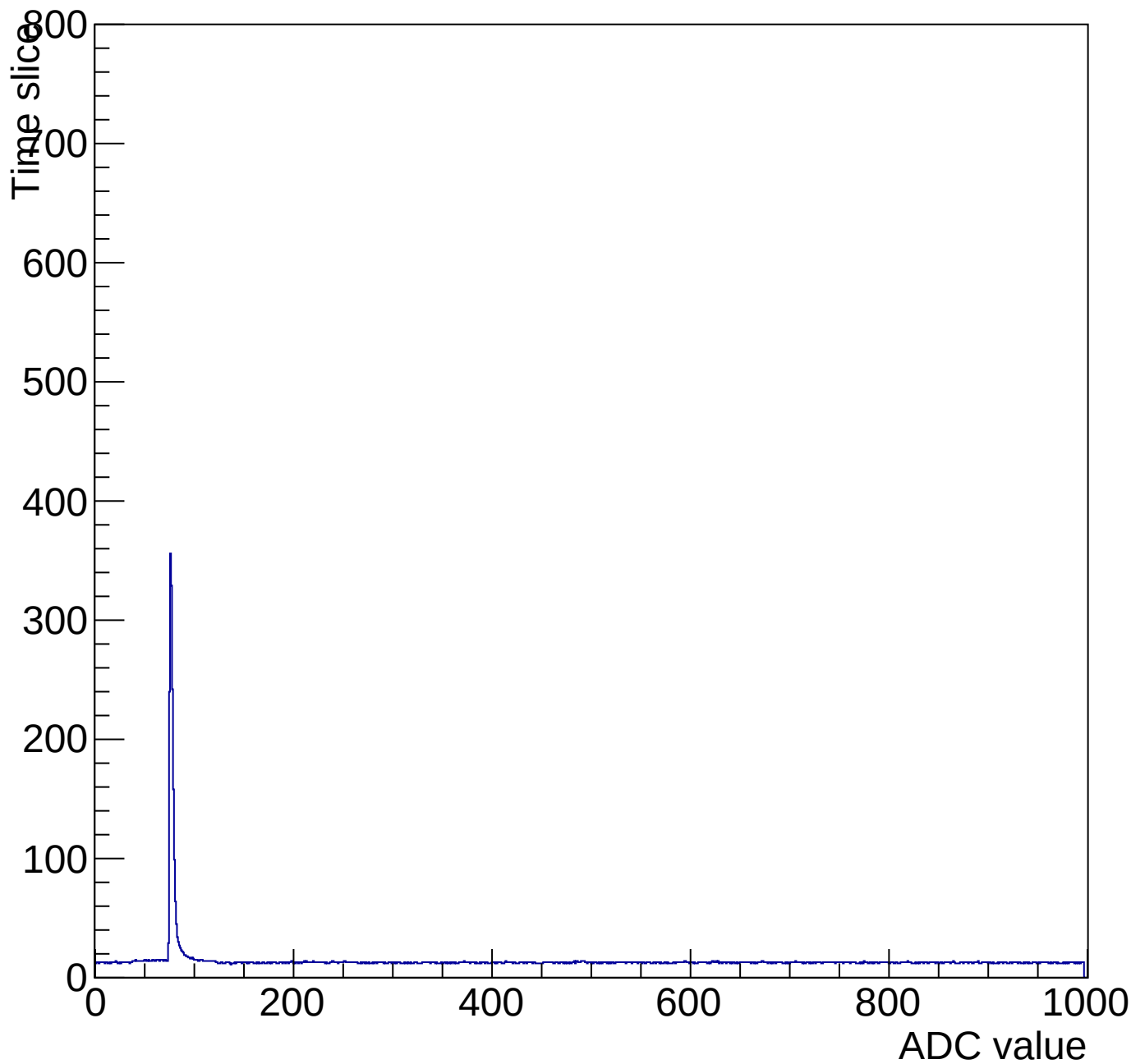
Evt 10 Time mcm 2006 chip 6 chan 14 pulser-10V-wire64
