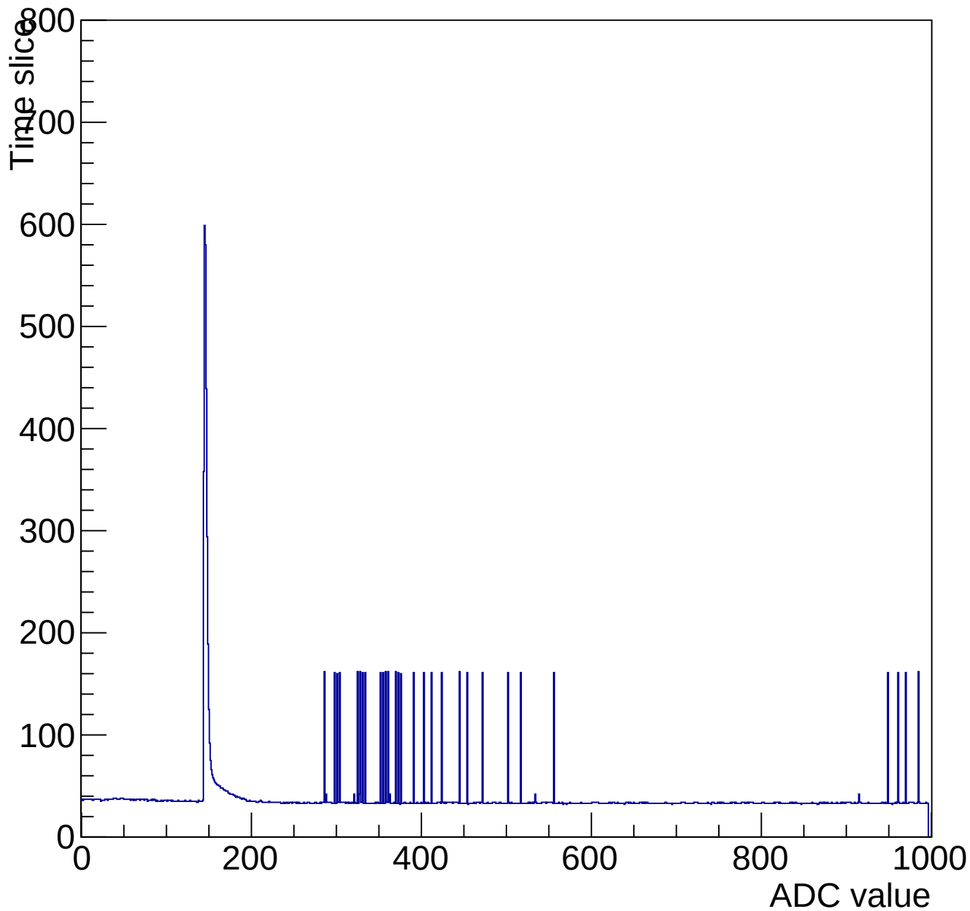
Evt 10 Time mcm 2006 chip 6 chan 0 pulser-10V-wire64
