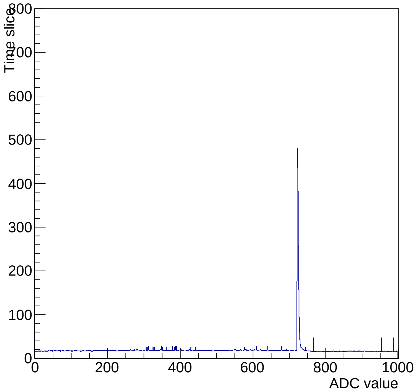
Evt 10 Time mcm 2006 chip 6 chan 2 pulser-10V-wire64
