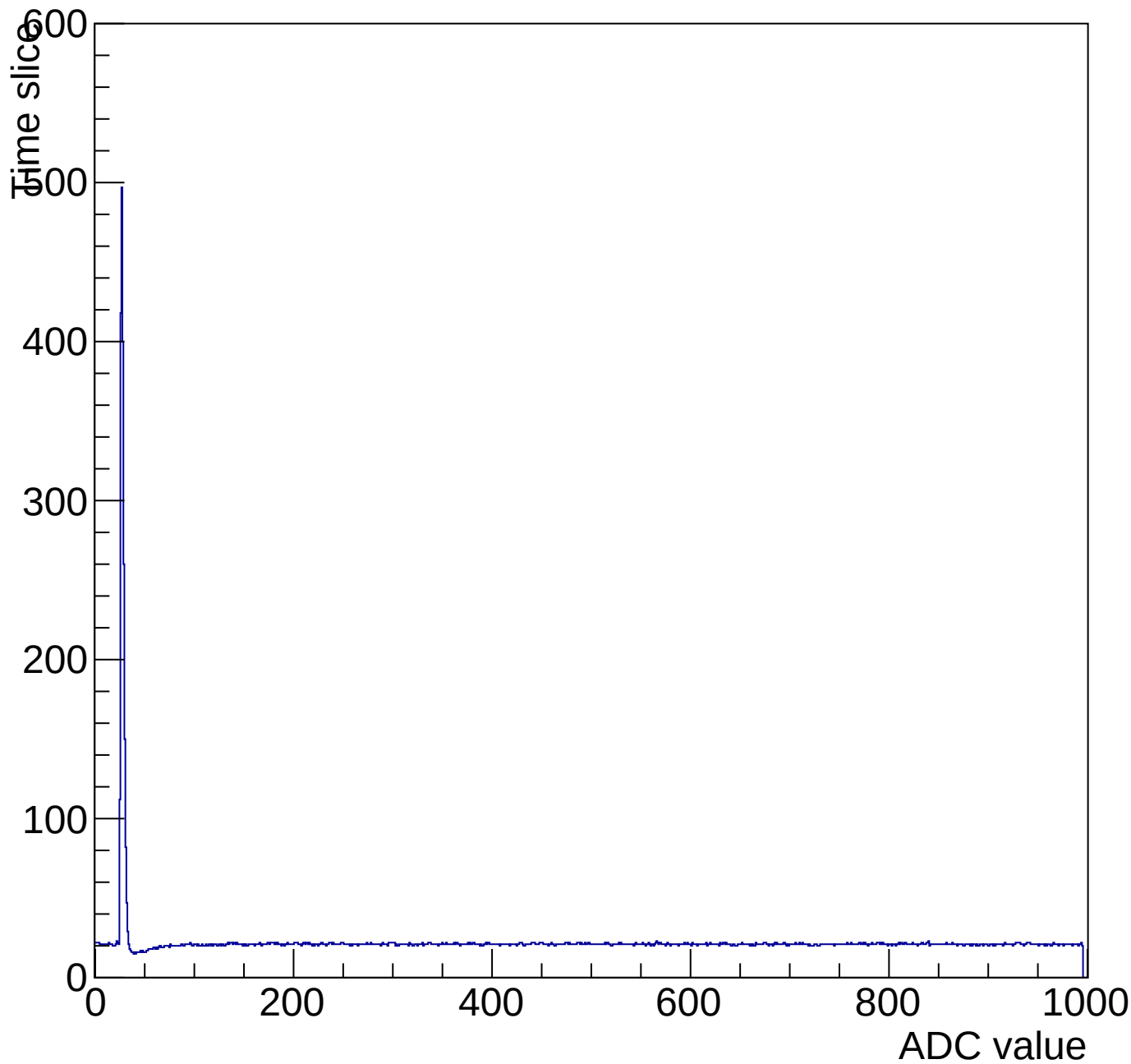
Evt 10 Time mcm 2007 chip 7 chan 6 pulser-10V-wire64
