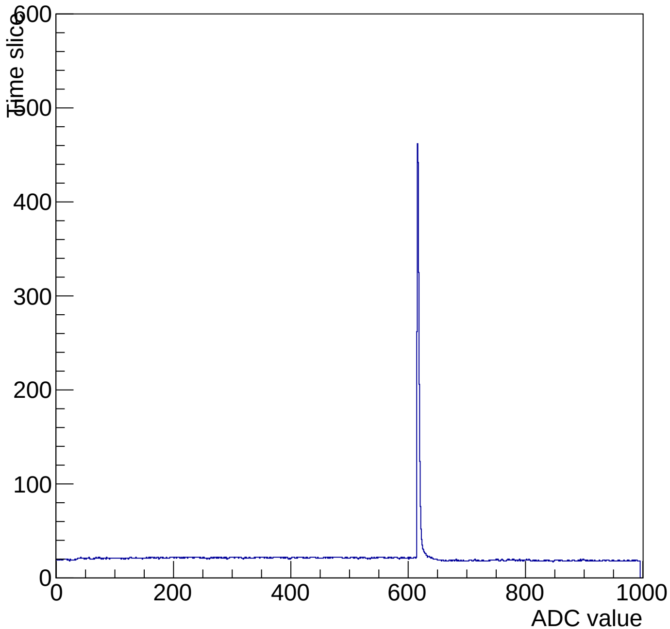
Evt 10 Time mcm 2007 chip 7 chan 10 pulser-10V-wire64
