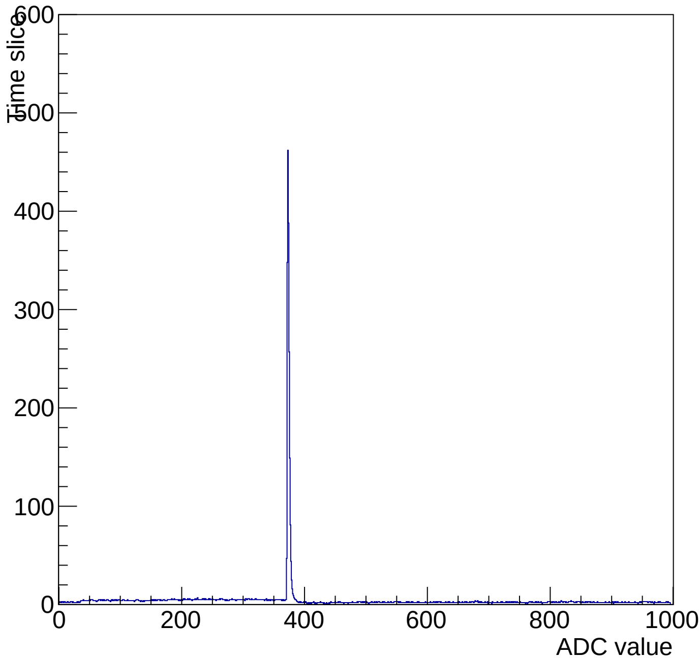
Evt 10 Time mcm 2007 chip 7 chan 0 pulser-10V-wire64
