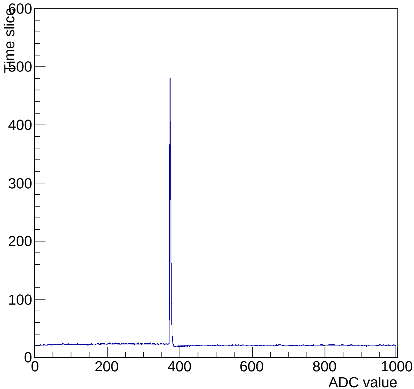
Evt 10 Time mcm 2007 chip 7 chan 1 pulser-10V-wire64
