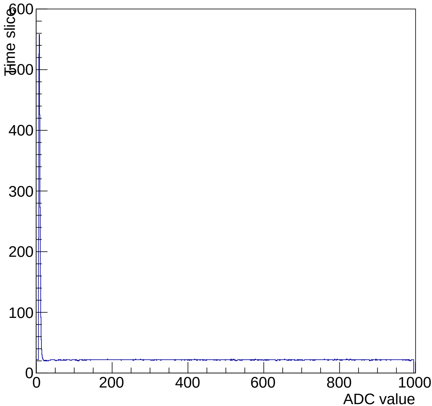
Evt 10 Time mcm 2007 chip 7 chan 13 pulser-10V-wire64
