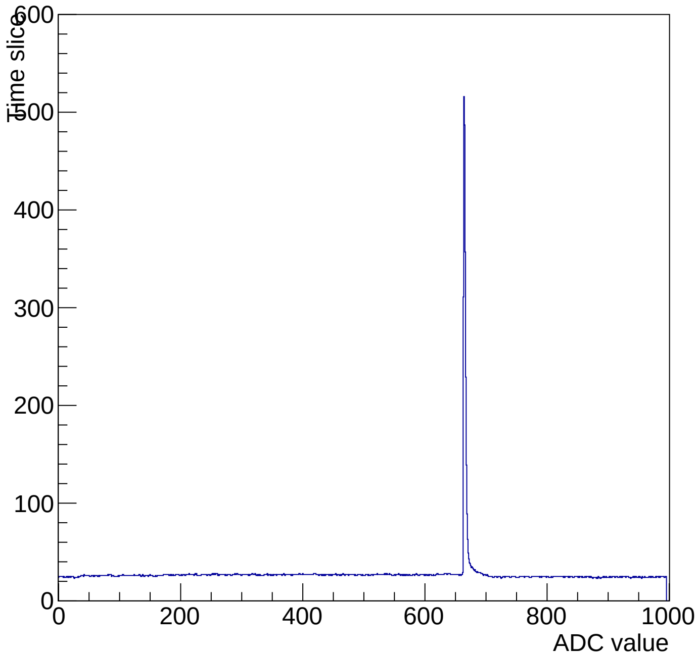
Evt 10 Time mcm 2007 chip 7 chan 14 pulser-10V-wire64
