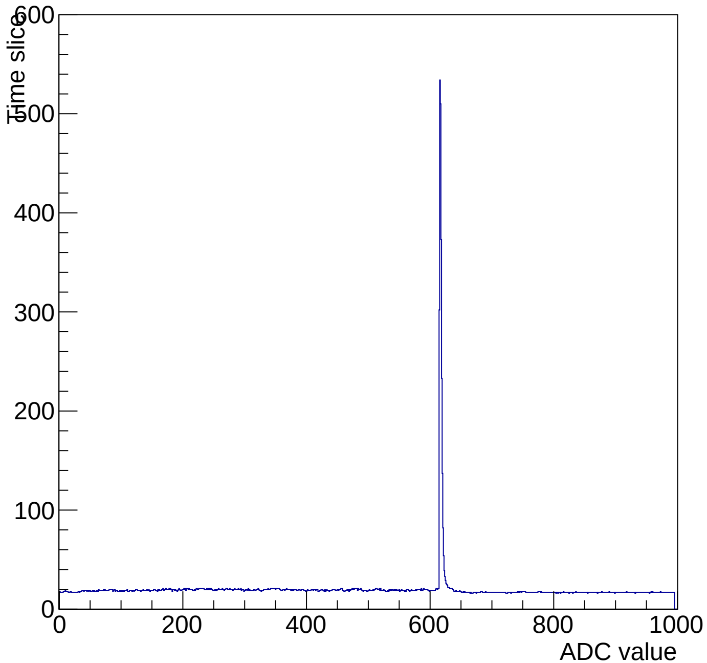
Evt 10 Time mcm 2007 chip 7 chan 11 pulser-10V-wire64
