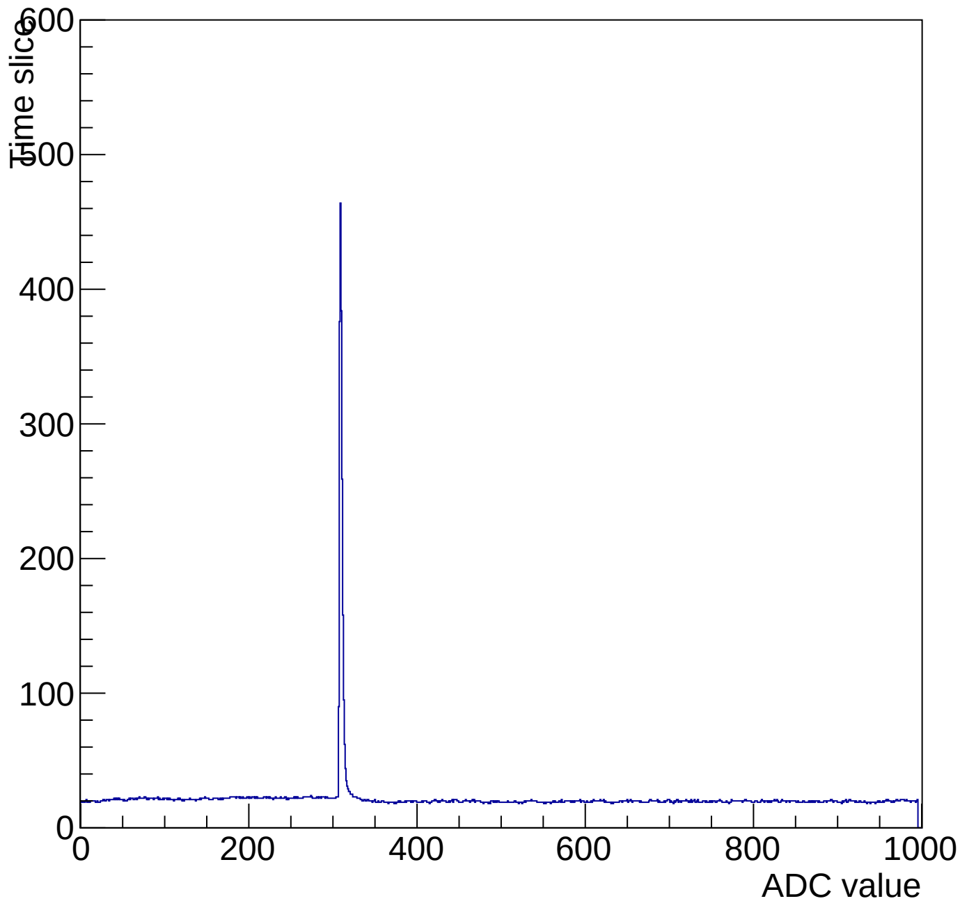
Evt 10 Time mcm 2007 chip 7 chan 3 pulser-10V-wire64
