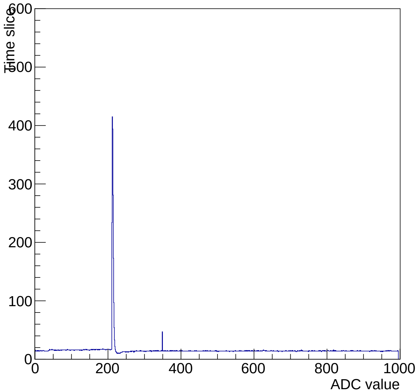
Evt 10 Time mcm 2007 chip 7 chan 8 pulser-10V-wire64
