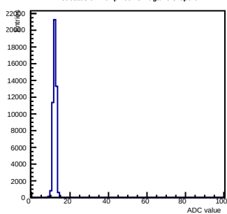
Pedestals ch 1 chip 2004 shift-gain0-shaper0
