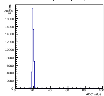
Pedestals ch 3 chip 2004 shift-gain0-shaper0
