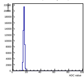
Pedestals ch 8 chip 2004 shift-gain0-shaper0
