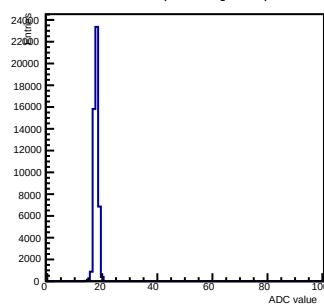
Pedestals ch 10 chip 2004 shift-gain0-shaper0
