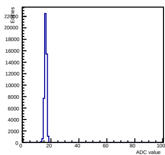
Pedestals ch 13 chip 2004 shift-gain0-shaper0
