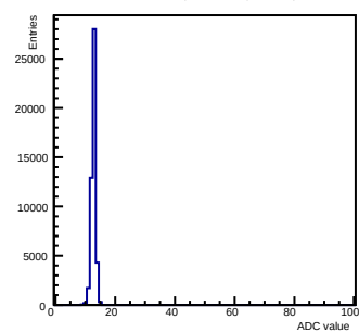
Pedestals ch 15 chip 2004 shift-gain0-shaper0
