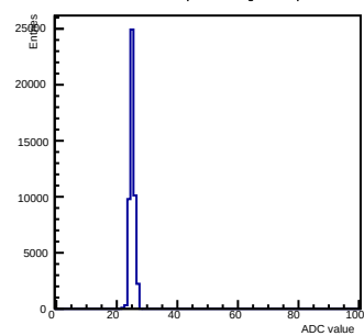
Pedestals ch 11 chip 2004 shift-gain0-shaper0
