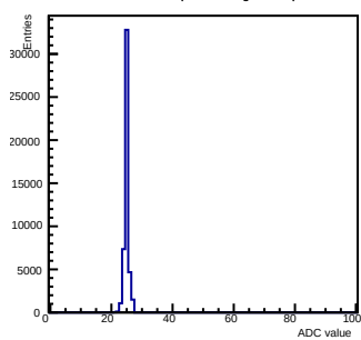
Pedestals ch 9 chip 2004 shift-gain0-shaper0
