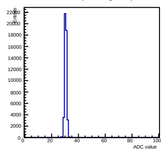
Pedestals ch 7 chip 2004 shift-gain0-shaper0
