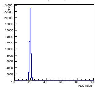
Pedestals ch 4 chip 2004 shift-gain0-shaper0
