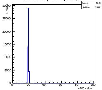
Pedestals ch 10 chip 2004 shift-gain0-shaper6
