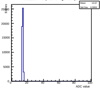
Pedestals ch 1 chip 2004 shift-gain0-shaper6
