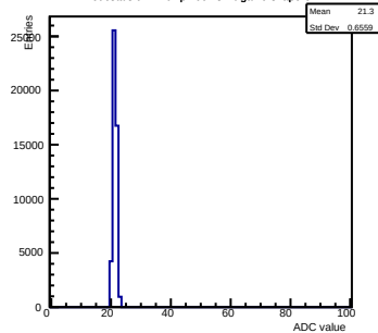
Pedestals ch 11 chip 2004 shift-gain0-shaper6
