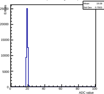
Pedestals ch 4 chip 2004 shift-gain0-shaper6
