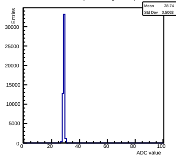
Pedestals ch 7 chip 2004 shift-gain0-shaper6
