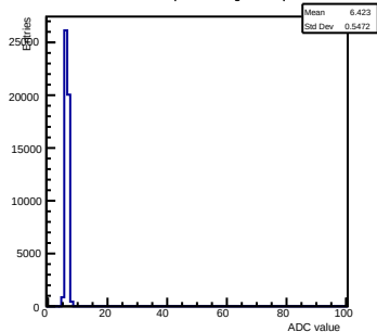
Pedestals ch 6 chip 2004 shift-gain0-shaper6
