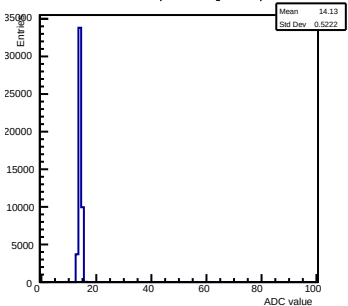
Pedestals ch 13 chip 2004 shift-gain0-shaper6
