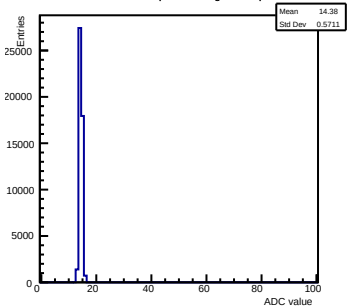
Pedestals ch 5 chip 2004 shift-gain0-shaper6
