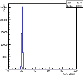
Pedestals ch 12 chip 2004 shift-gain0-shaper6
