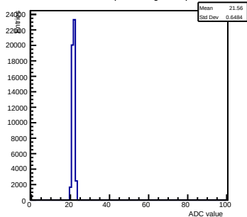
Pedestals ch 14 chip 2004 shift-gain0-shaper6
