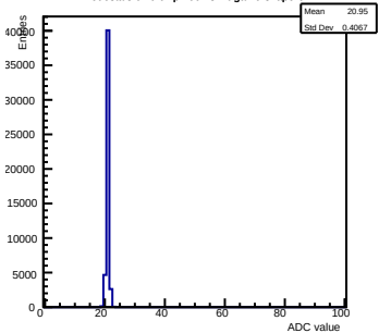
Pedestals ch 9 chip 2004 shift-gain0-shaper6
