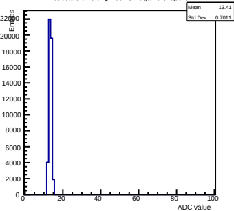
Pedestals ch 8 chip 2004 shift-gain0-shaper6
