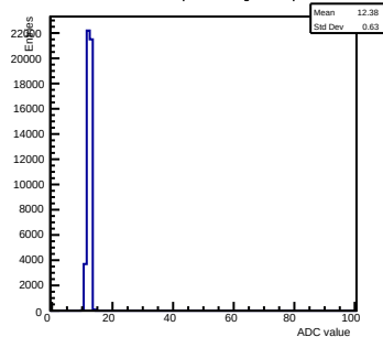
Pedestals ch 15 chip 2004 shift-gain0-shaper6
