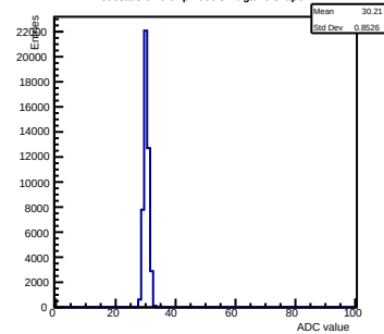
Pedestals ch 0 chip 2006 shift-gain0-shaper7
