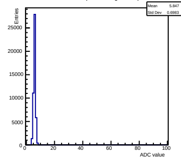
Pedestals ch 4 chip 2006 shift-gain0-shaper7
