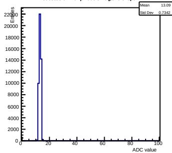
Pedestals ch 2 chip 2006 shift-gain0-shaper7
