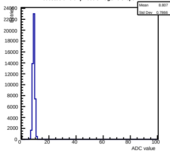
Pedestals ch 9 chip 2006 shift-gain0-shaper7
