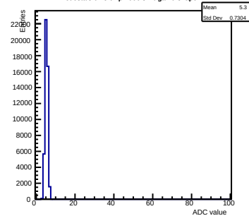
Pedestals ch 8 chip 2006 shift-gain0-shaper7
