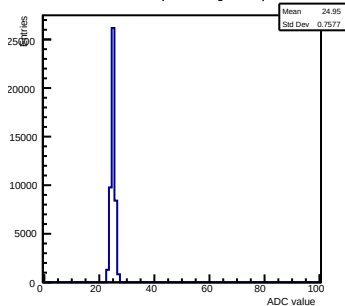
Pedestals ch 5 chip 2006 shift-gain0-shaper7
