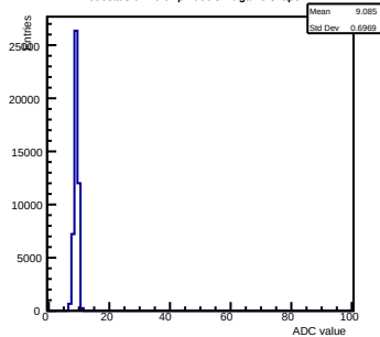
Pedestals ch 10 chip 2006 shift-gain0-shaper7
