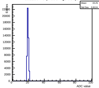
Pedestals ch 1 chip 2006 shift-gain0-shaper7
