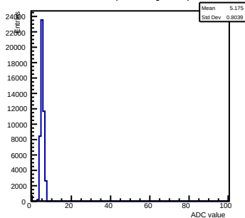
Pedestals ch 7 chip 2006 shift-gain0-shaper7
