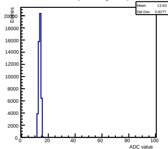
Pedestals ch 14 chip 2006 shift-gain0-shaper7
