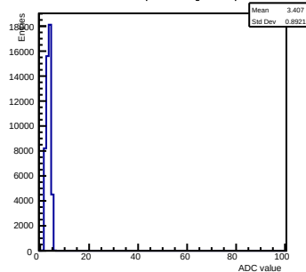
Pedestals ch 15 chip 2006 shift-gain0-shaper7
