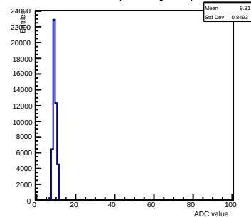
Pedestals ch 12 chip 2006 shift-gain0-shaper7
