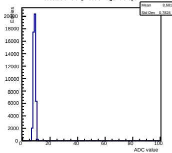
Pedestals ch 3 chip 2006 shift-gain0-shaper7
