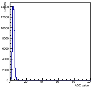
Pedestals ch 0 chip 2007 shift-gain0-shaper0
