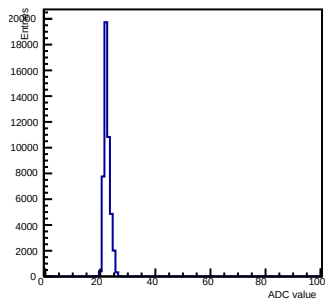
Pedestals ch 1 chip 2007 shift-gain0-shaper0
