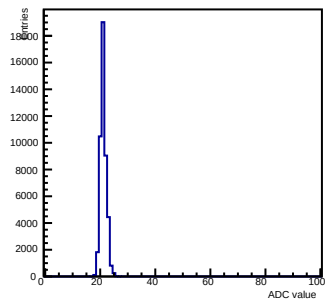
Pedestals ch 3 chip 2007 shift-gain0-shaper0
