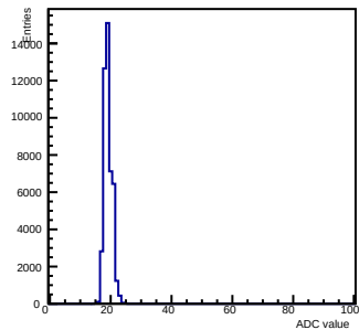
Pedestals ch 11 chip 2007 shift-gain0-shaper0
