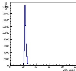
Pedestals ch 6 chip 2007 shift-gain0-shaper0
