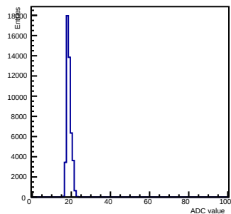
Pedestals ch 5 chip 2007 shift-gain0-shaper0
