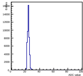
Pedestals ch 13 chip 2007 shift-gain0-shaper0
