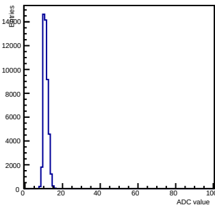
Pedestals ch 12 chip 2007 shift-gain0-shaper0
