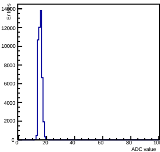
Pedestals ch 8 chip 2007 shift-gain0-shaper0
