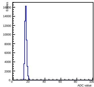
Pedestals ch 9 chip 2007 shift-gain0-shaper0
