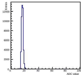
Pedestals ch 15 chip 2007 shift-gain0-shaper0
