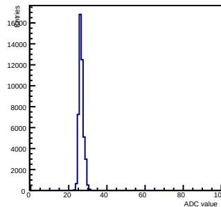
Pedestals ch 14 chip 2007 shift-gain0-shaper0
