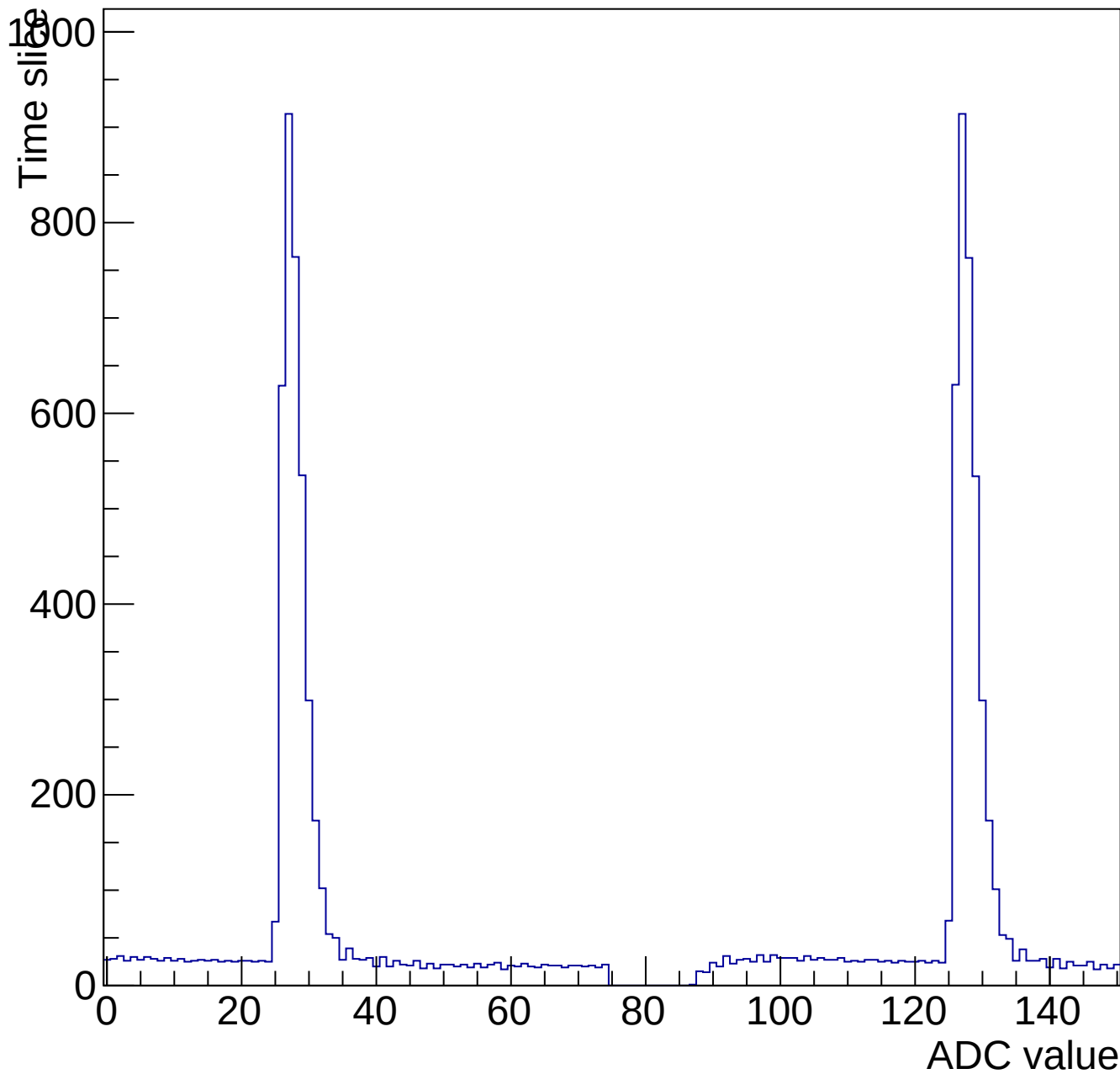
Evt 10 Time mcm 2007 chip 7 chan 1 square-7V-wire64-1000
