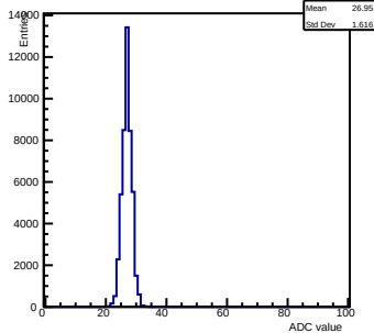
Pedestals ch 10 chip 2002 shift-gain3-shaper0
