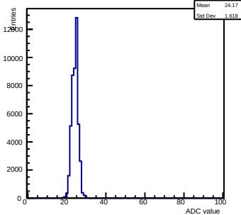
Pedestals ch 9 chip 2002 shift-gain3-shaper0
