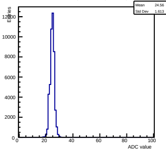
Pedestals ch 13 chip 2002 shift-gain3-shaper0
