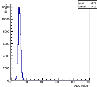
Pedestals ch 12 chip 2002 shift-gain3-shaper0
