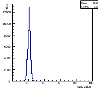
Pedestals ch 15 chip 2002 shift-gain3-shaper0
