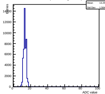
Pedestals ch 3 chip 2002 shift-gain3-shaper0
