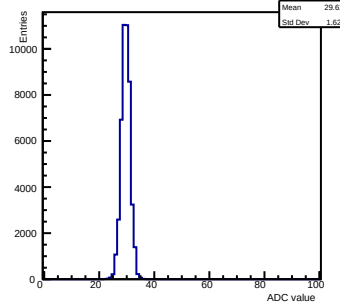
Pedestals ch 11 chip 2002 shift-gain3-shaper0
