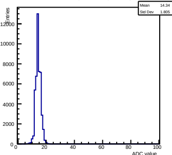
Pedestals ch 5 chip 2003 shift-gain3-shaper0
