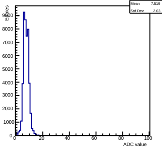
Pedestals ch 8 chip 2003 shift-gain3-shaper0
