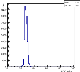
Pedestals ch 4 chip 2003 shift-gain3-shaper0
