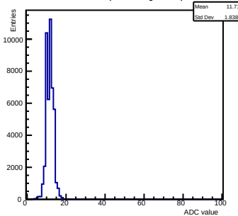
Pedestals ch 2 chip 2003 shift-gain3-shaper0
