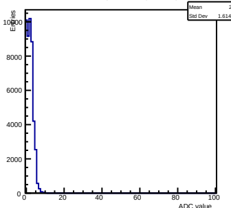
Pedestals ch 6 chip 2003 shift-gain3-shaper0
