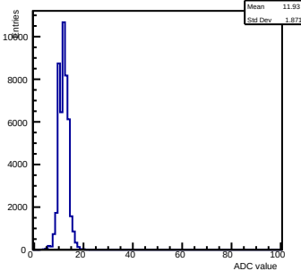
Pedestals ch 11 chip 2003 shift-gain3-shaper0
