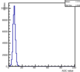
Pedestals ch 10 chip 2003 shift-gain3-shaper0
