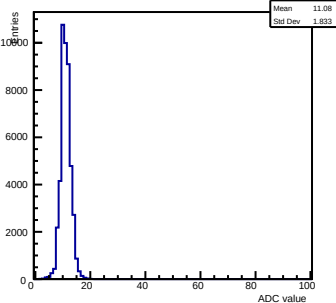
Pedestals ch 13 chip 2003 shift-gain3-shaper0
