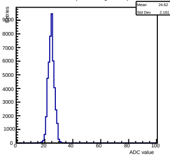
Pedestals ch 0 chip 2003 shift-gain3-shaper0
