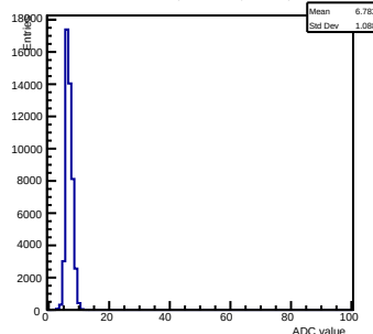
Pedestals ch 14 chip 2003 shift-gain0-shaper0
