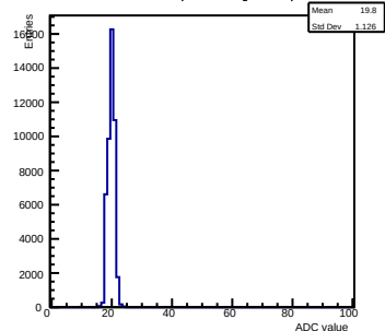
Pedestals ch 11 chip 2003 shift-gain0-shaper0
