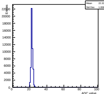
Pedestals ch 5 chip 2003 shift-gain0-shaper0
