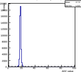
Pedestals ch 8 chip 2003 shift-gain0-shaper0
