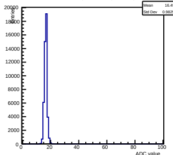
Pedestals ch 6 chip 2003 shift-gain0-shaper0
