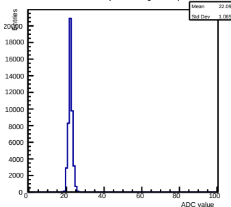
Pedestals ch 9 chip 2003 shift-gain0-shaper0
