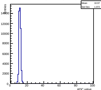
Pedestals ch 12 chip 2003 shift-gain0-shaper0
