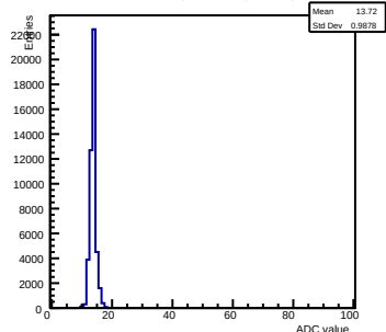
Pedestals ch 15 chip 2003 shift-gain0-shaper0
