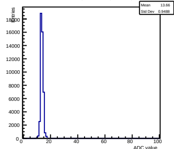
Pedestals ch 7 chip 2003 shift-gain0-shaper0
