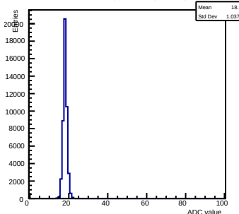
Pedestals ch 13 chip 2003 shift-gain0-shaper0
