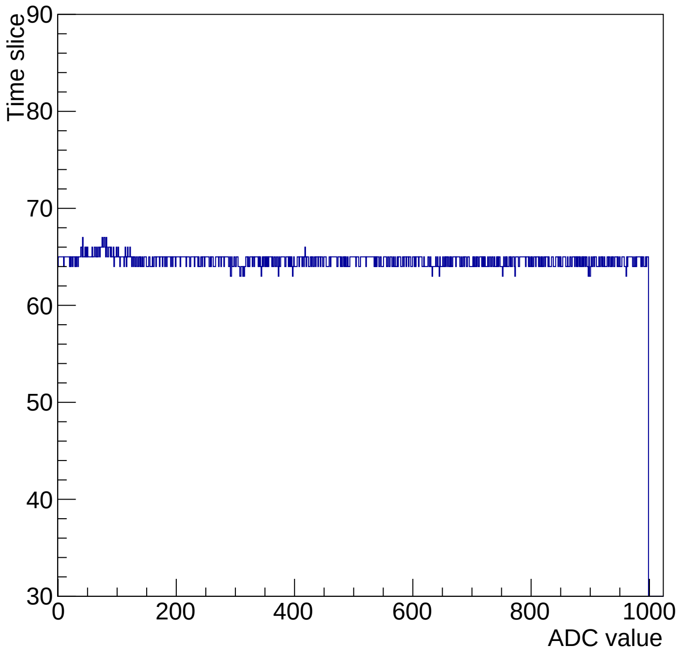
Evt 10 Time mcm 2000 chip 0 chan 4 1000-gain0-shaper0
