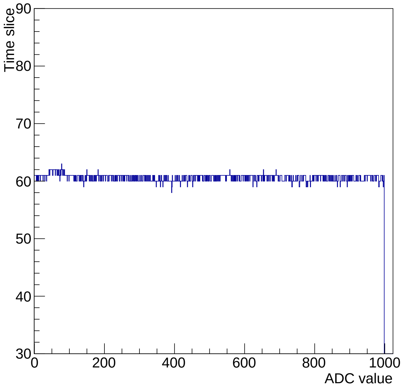
Evt 10 Time mcm 2000 chip 0 chan 15 1000-gain0-shaper0
