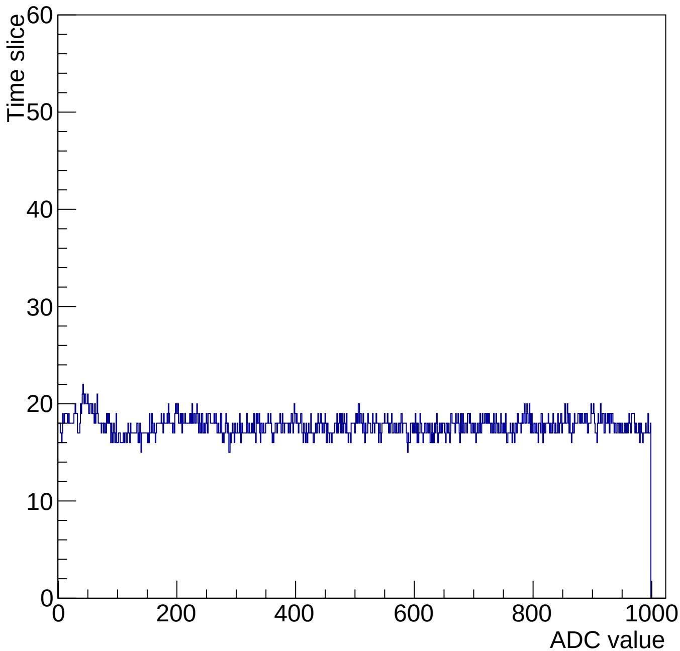
Evt 10 Time mcm 2000 chip 0 chan 4 1000-gain3-shaper0
