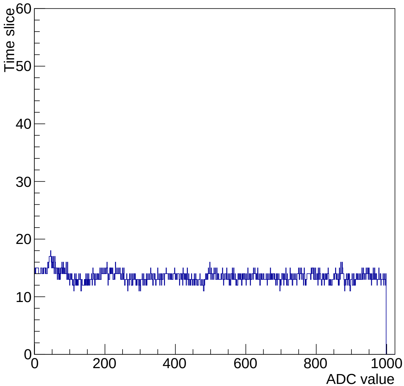
Evt 10 Time mcm 2000 chip 0 chan 9 1000-gain3-shaper0
