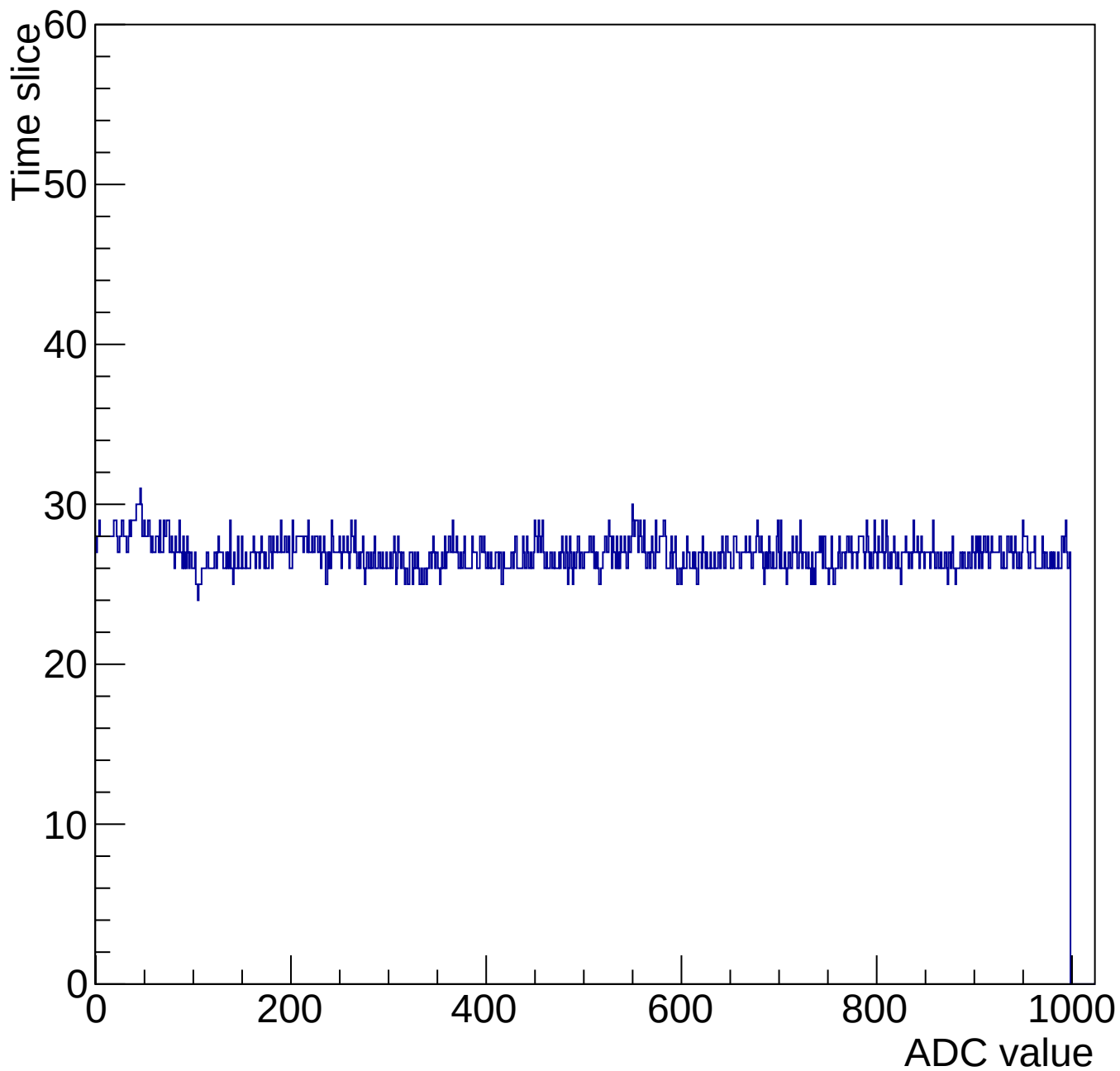
Evt 10 Time mcm 2000 chip 0 chan 12 1000-gain3-shaper0
