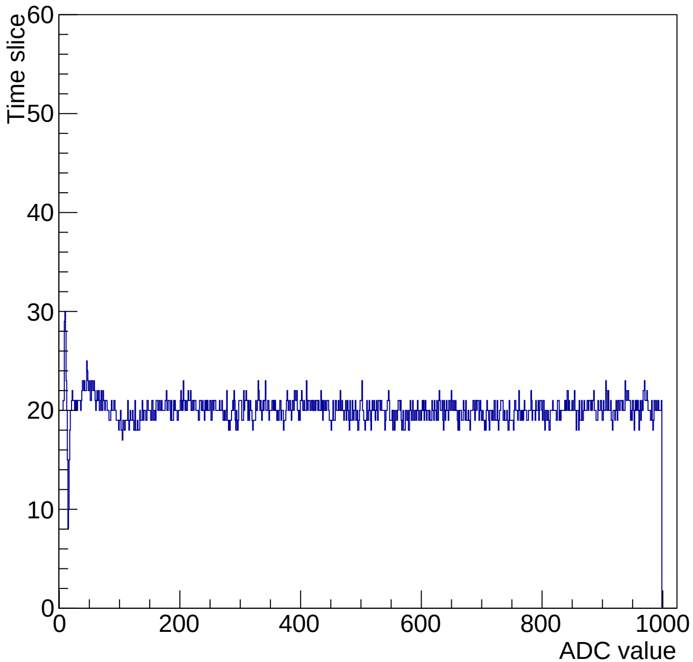
Evt 10 Time mcm 2000 chip 0 chan 2 1000-gain3-shaper0
