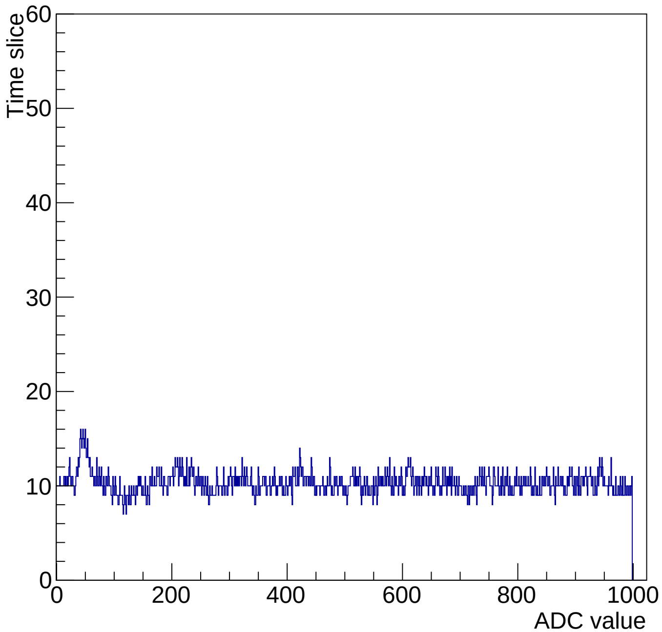
Evt 10 Time mcm 2000 chip 0 chan 0 1000-gain3-shaper0
