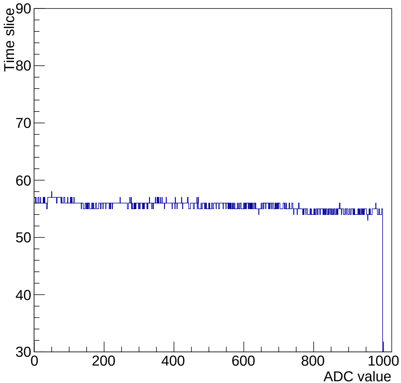
Evt 10 Time mcm 2001 chip 1 chan 7 1000-gain0-shaper0
