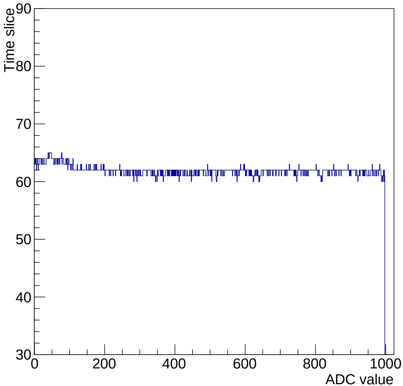
Evt 10 Time mcm 2001 chip 1 chan 5 1000-gain0-shaper0
