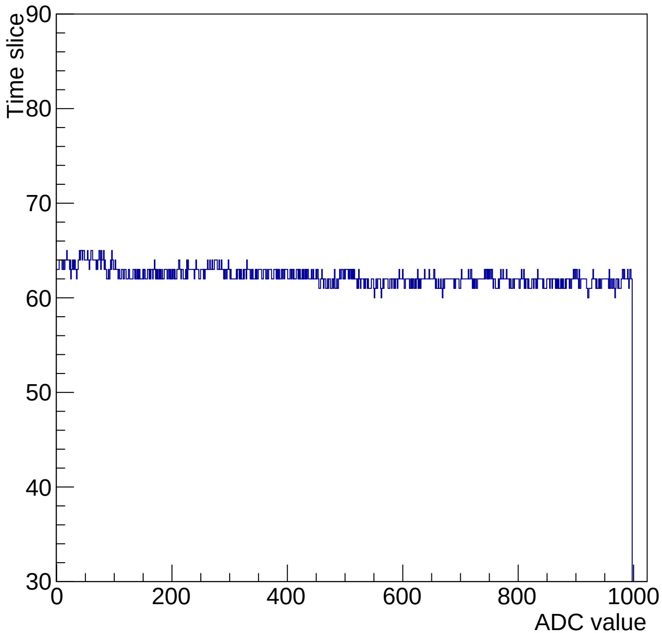
Evt 10 Time mcm 2001 chip 1 chan 12 1000-gain0-shaper0
