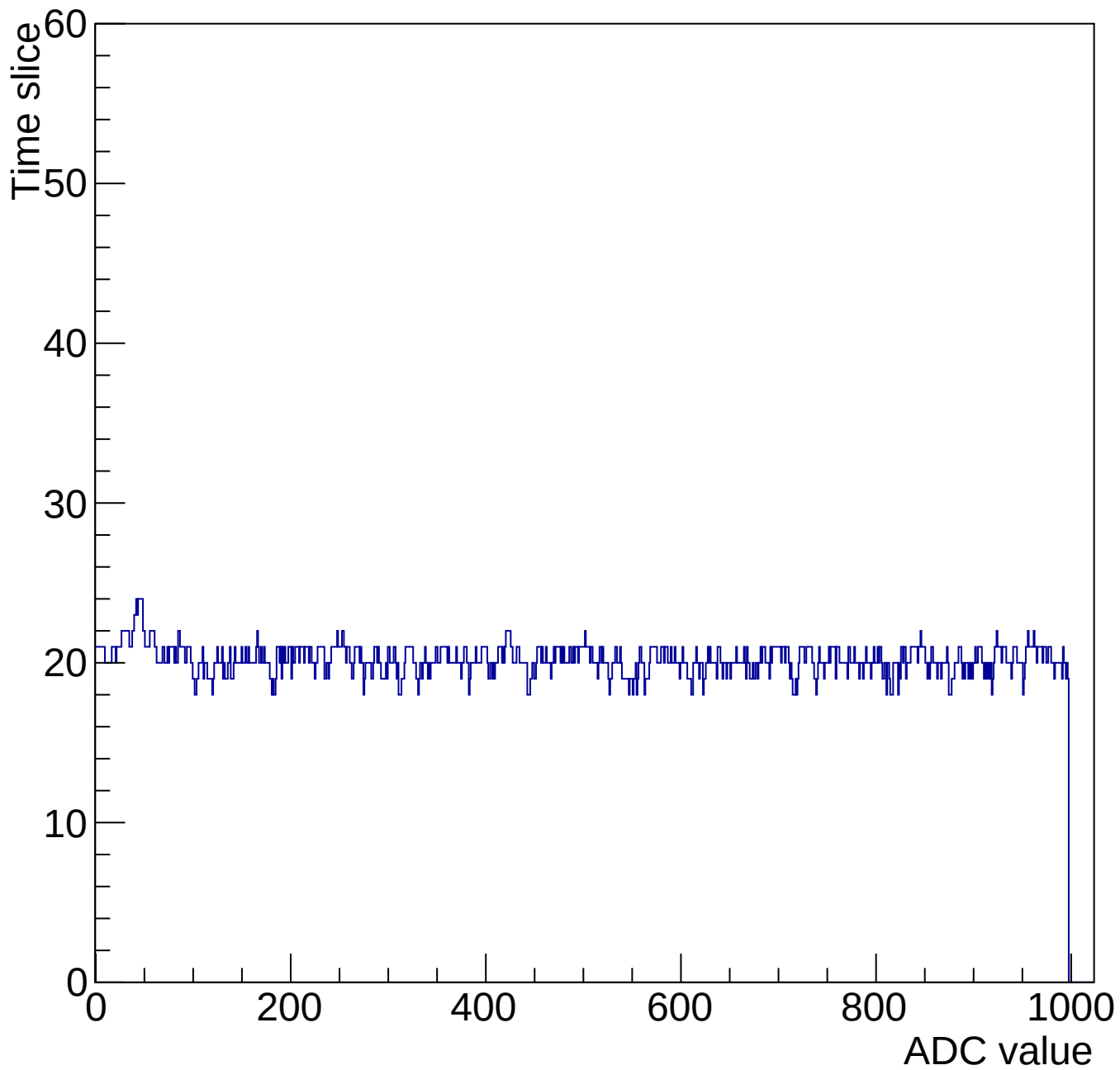
Evt 10 Time mcm 2001 chip 1 chan 11 1000-gain3-shaper0
