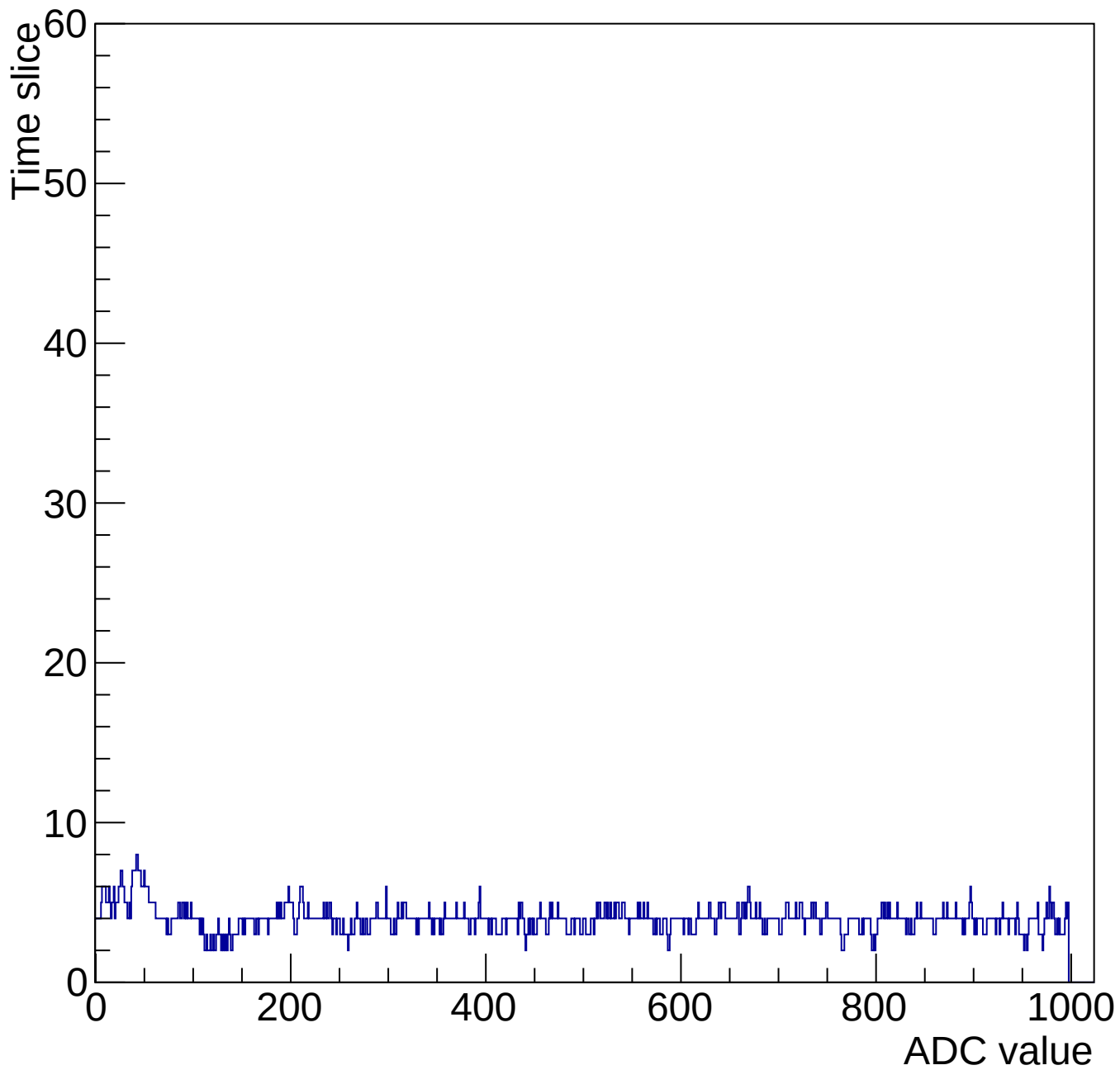
Evt 10 Time mcm 2001 chip 1 chan 2 1000-gain3-shaper0
