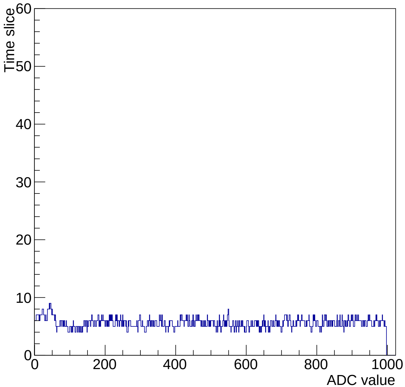
Evt 10 Time mcm 2001 chip 1 chan 7 1000-gain3-shaper0
