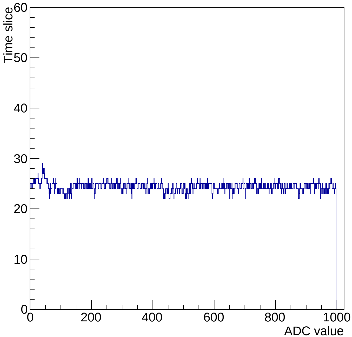
Evt 10 Time mcm 2001 chip 1 chan 3 1000-gain3-shaper0
