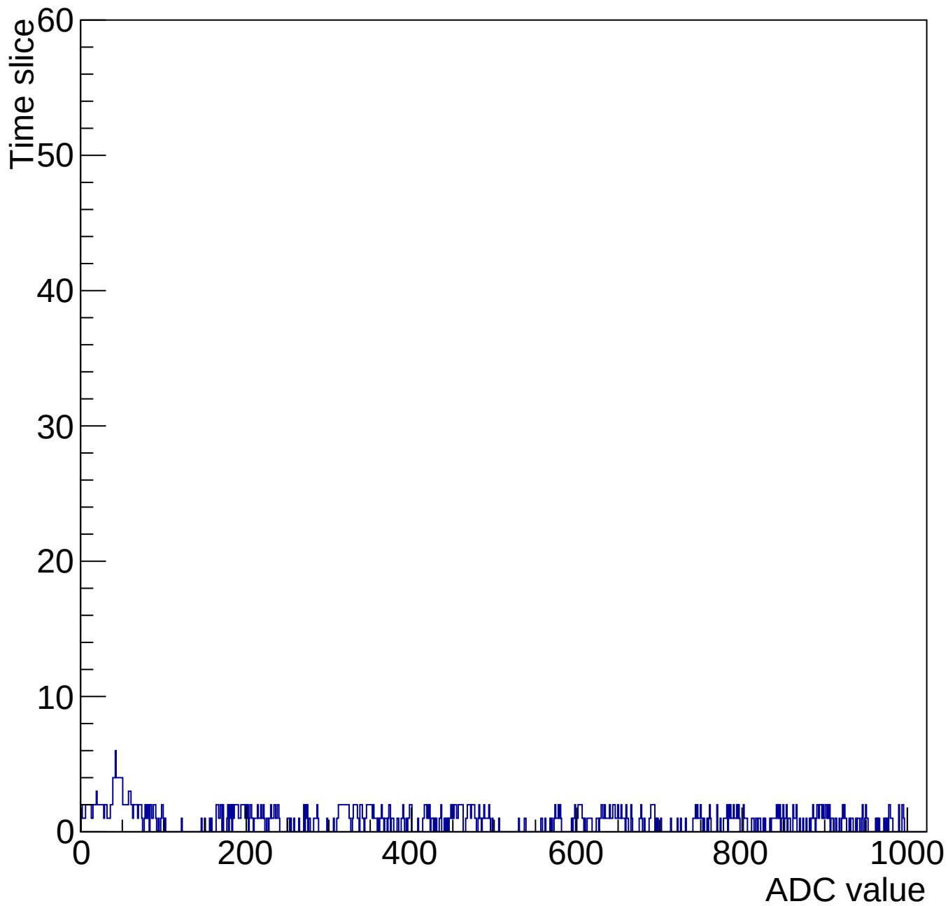
Evt 10 Time mcm 2001 chip 1 chan 1 1000-gain3-shaper0
