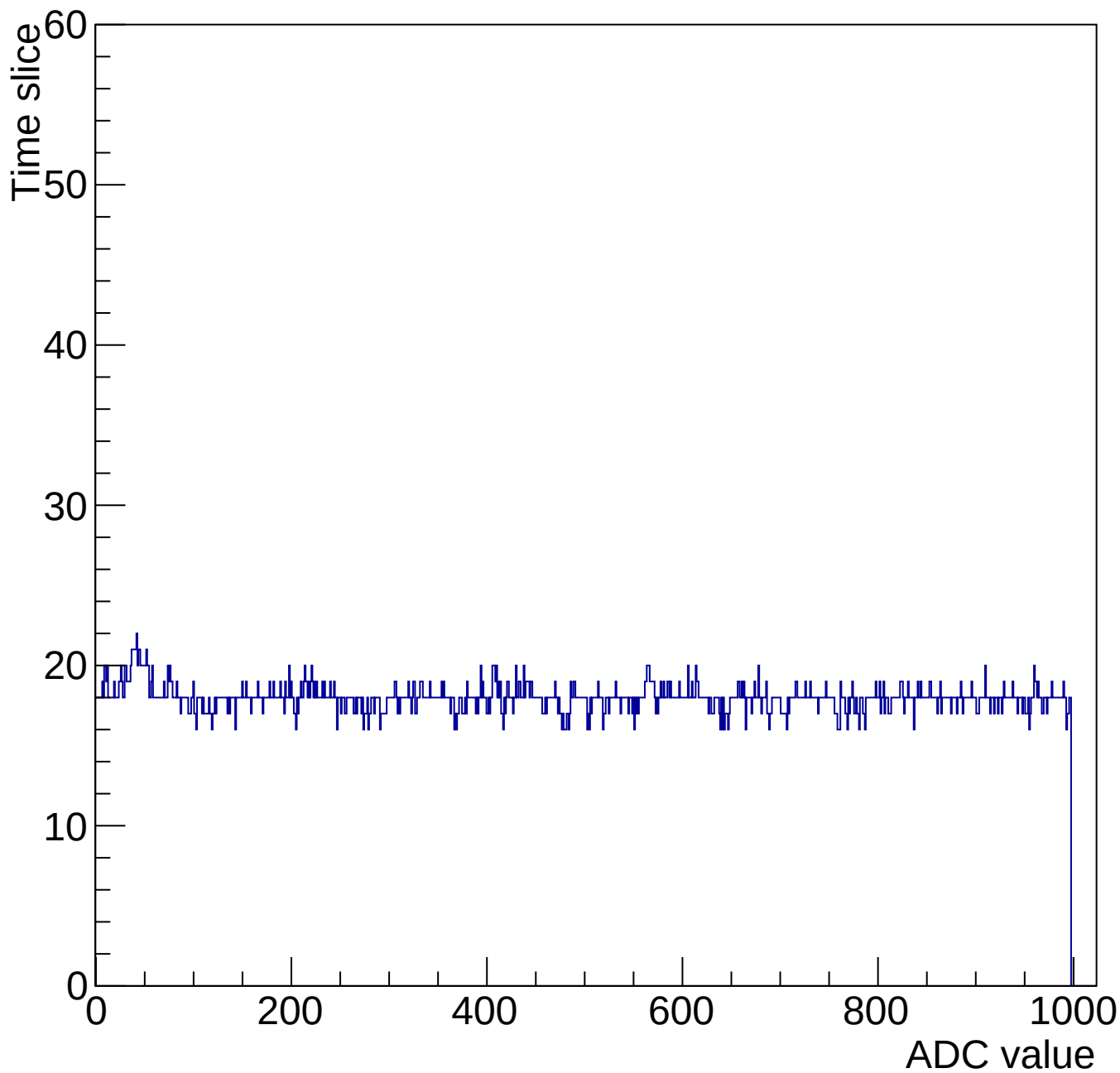
Evt 10 Time mcm 2001 chip 1 chan 9 1000-gain3-shaper0
