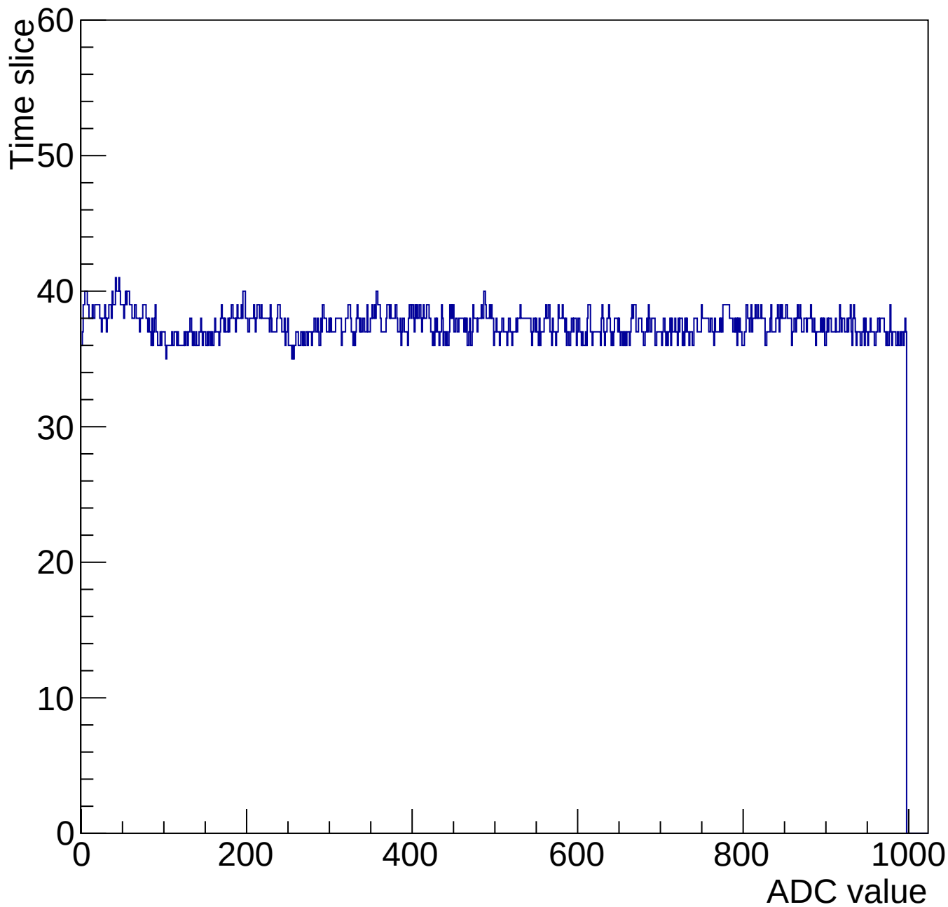
Evt 10 Time mcm 2001 chip 1 chan 15 1000-gain3-shaper0
