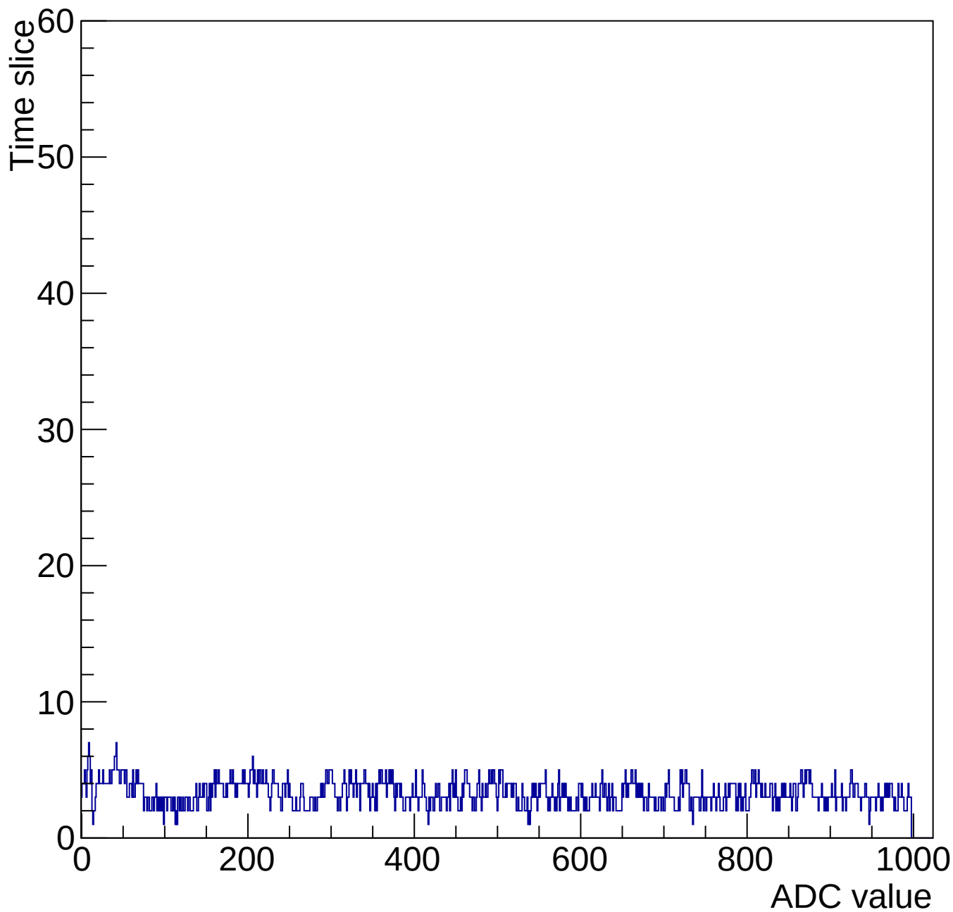
Evt 10 Time mcm 2001 chip 1 chan 14 1000-gain3-shaper0
