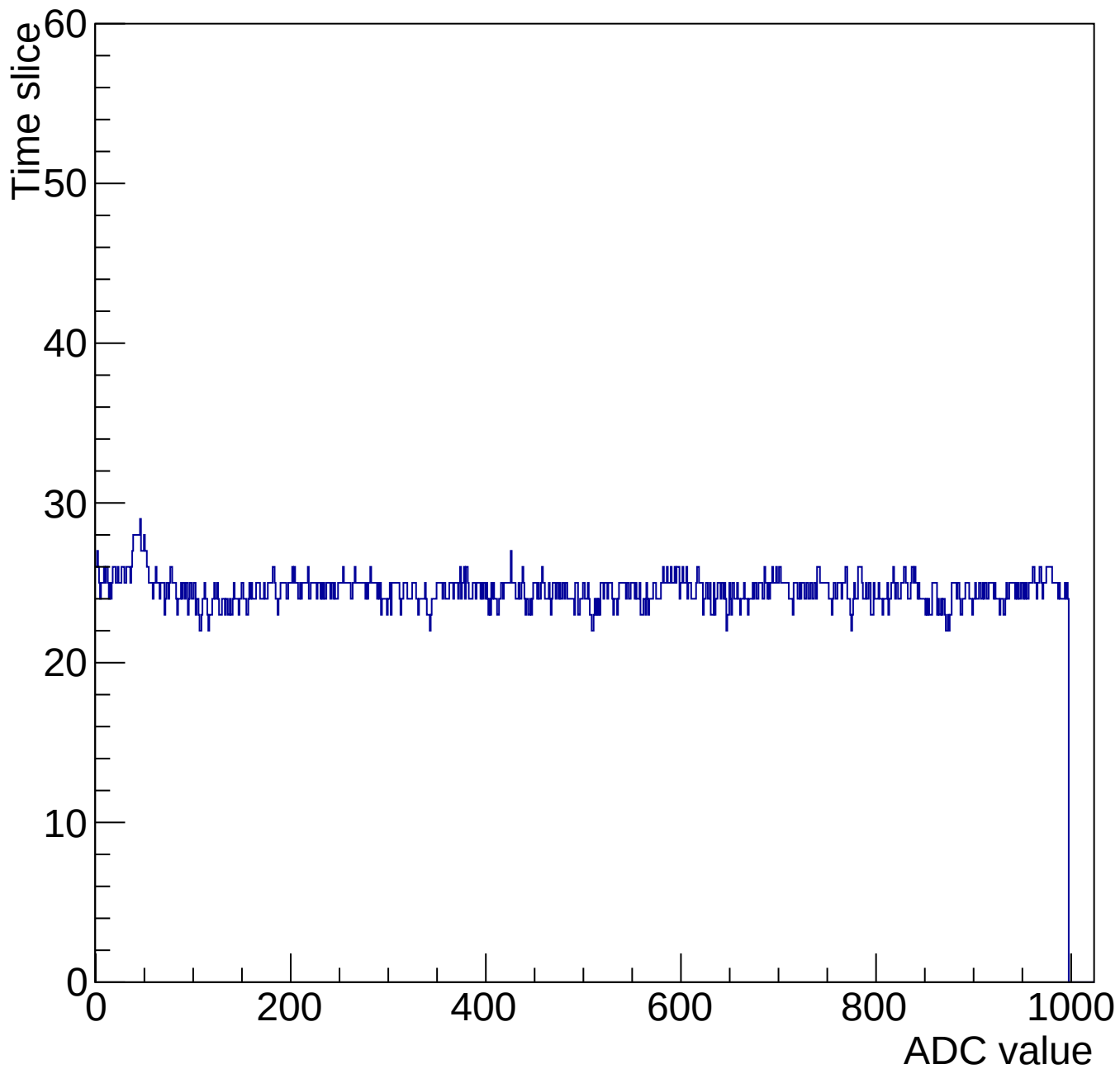
Evt 10 Time mcm 2001 chip 1 chan 10 1000-gain3-shaper0
