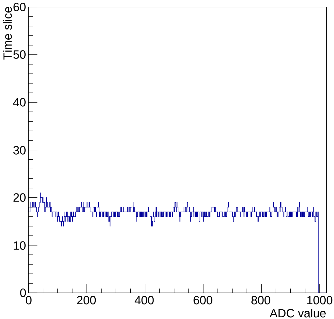
Evt 10 Time mcm 2002 chip 2 chan 0 1000-gain3-shaper0
