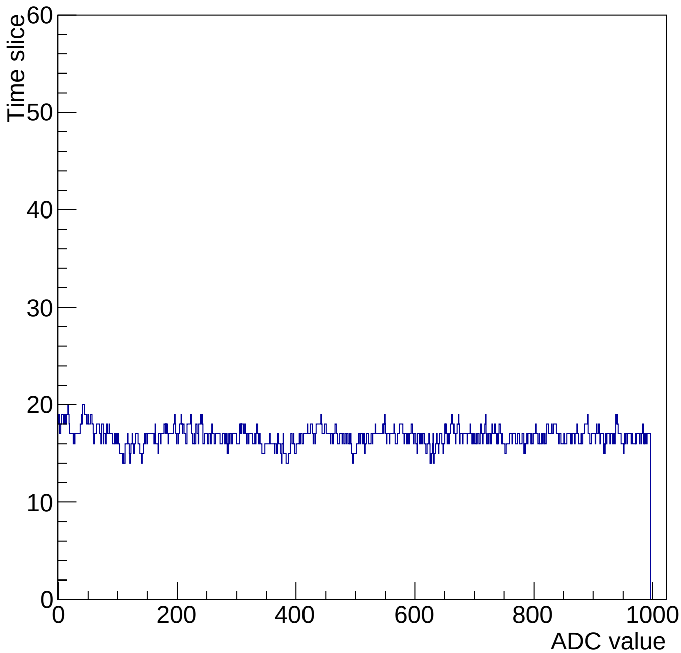
Evt 10 Time mcm 2002 chip 2 chan 11 1000-gain3-shaper0
