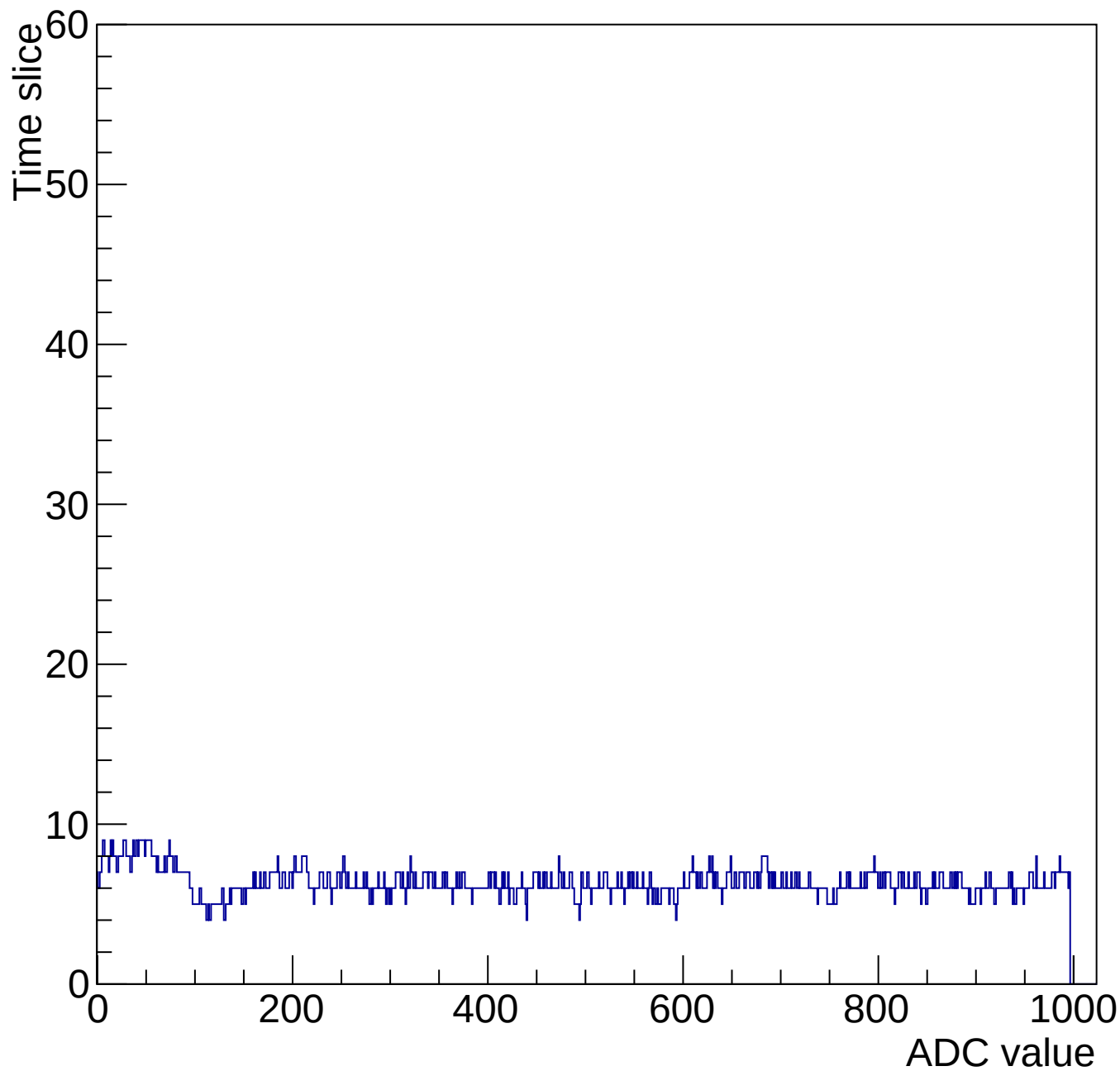
Evt 10 Time mcm 2002 chip 2 chan 15 1000-gain3-shaper0
