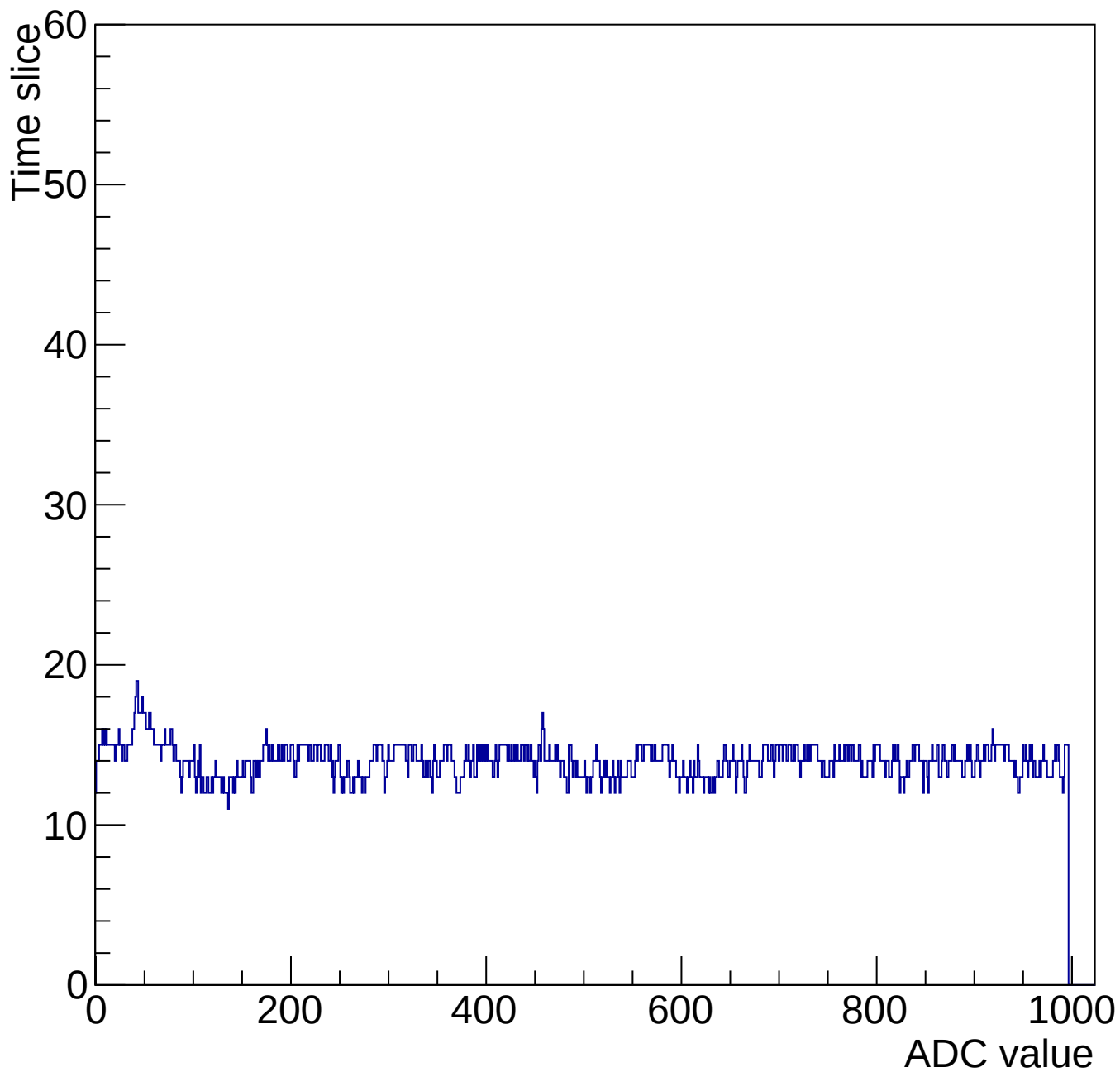
Evt 10 Time mcm 2002 chip 2 chan 10 1000-gain3-shaper0
