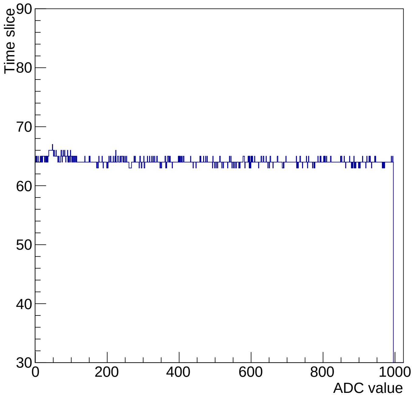
Evt 10 Time mcm 2003 chip 3 chan 5 1000-gain0-shaper0
