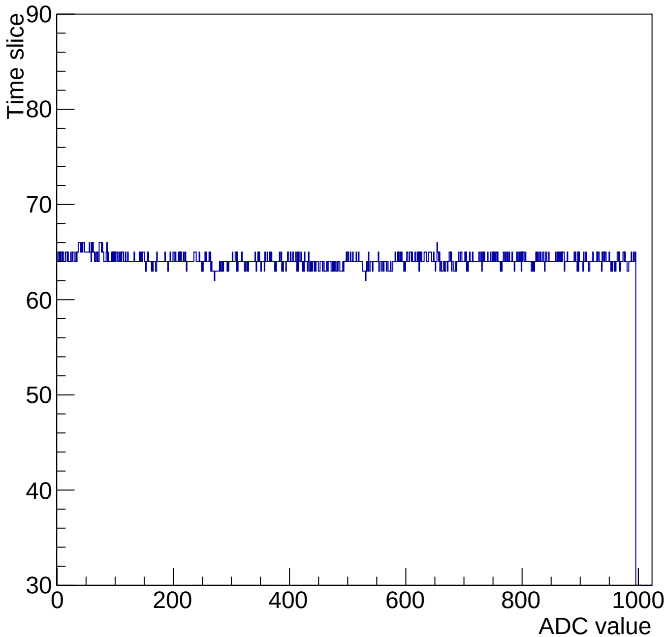
Evt 10 Time mcm 2003 chip 3 chan 9 1000-gain0-shaper0
