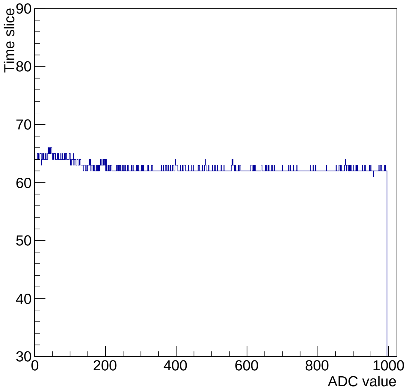
Evt 10 Time mcm 2003 chip 3 chan 11 1000-gain0-shaper0
