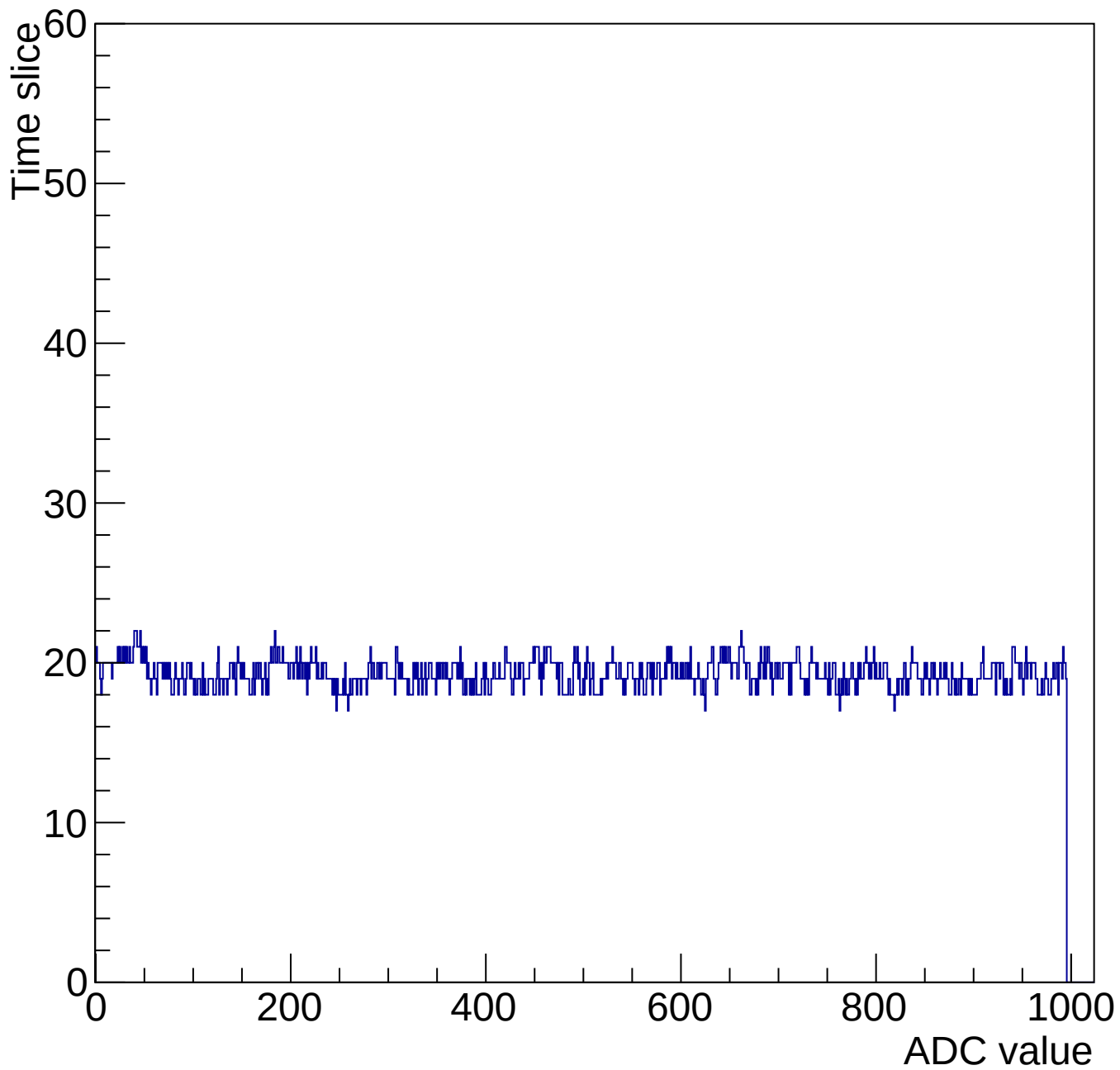
Evt 10 Time mcm 2003 chip 3 chan 13 1000-gain3-shaper0
