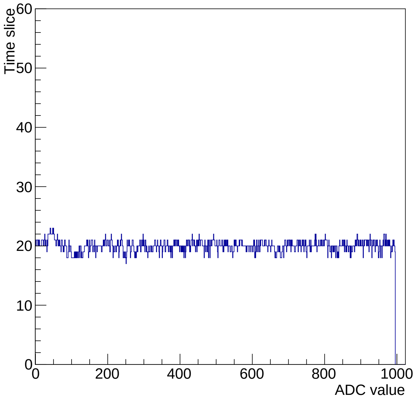
Evt 10 Time mcm 2003 chip 3 chan 2 1000-gain3-shaper0
