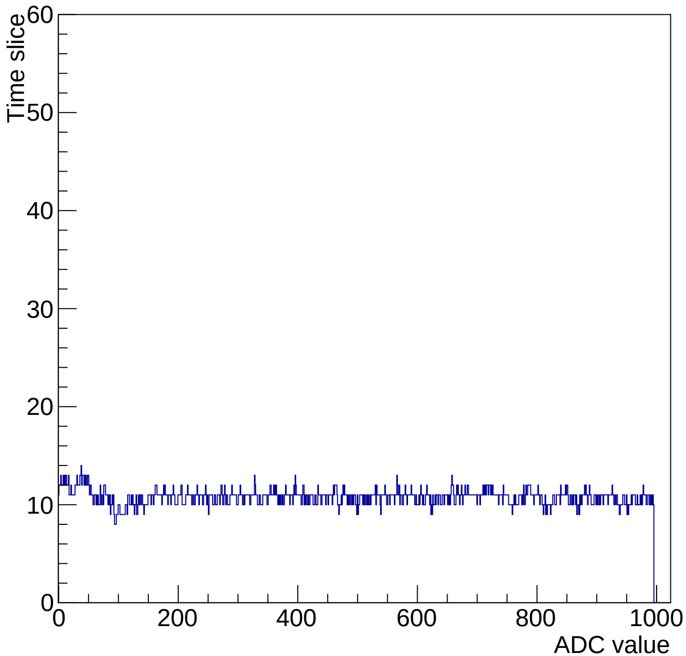
Evt 10 Time mcm 2003 chip 3 chan 6 1000-gain3-shaper0
