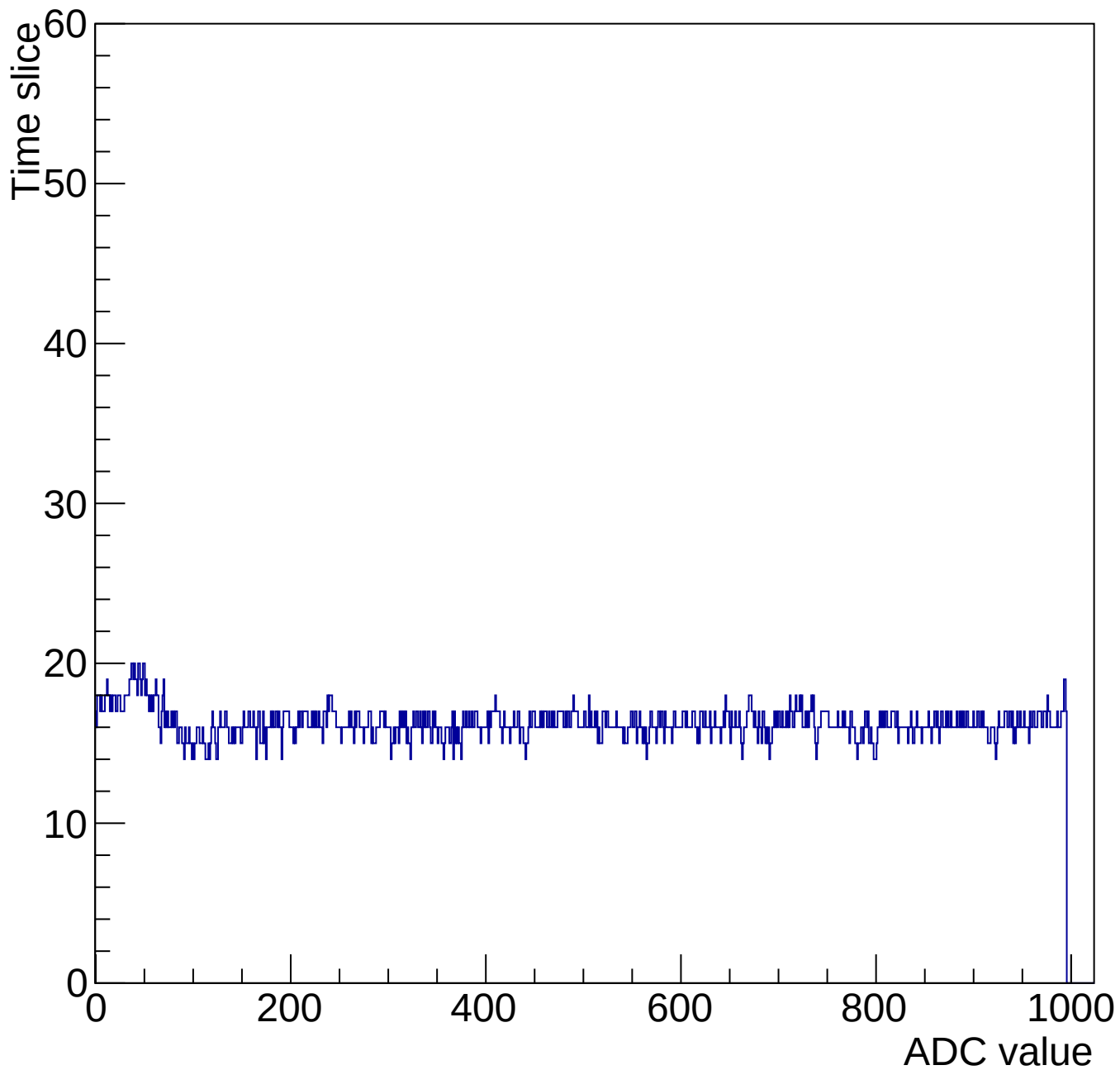
Evt 10 Time mcm 2003 chip 3 chan 10 1000-gain3-shaper0
