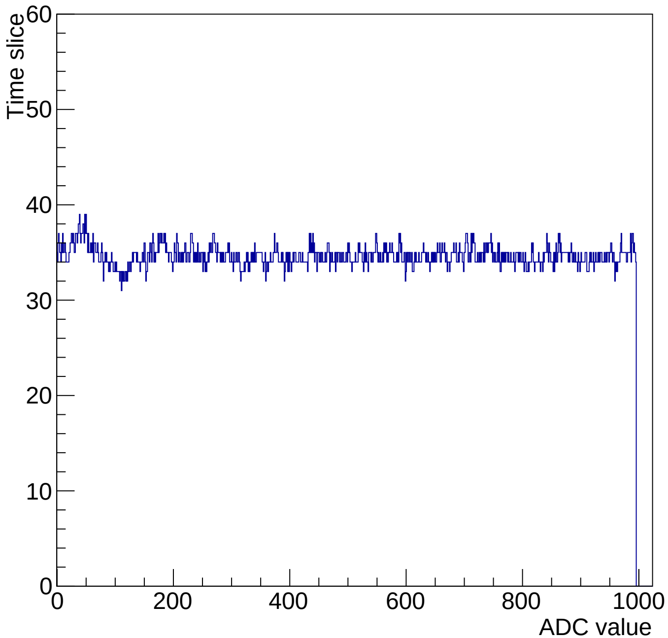
Evt 10 Time mcm 2003 chip 3 chan 4 1000-gain3-shaper0
