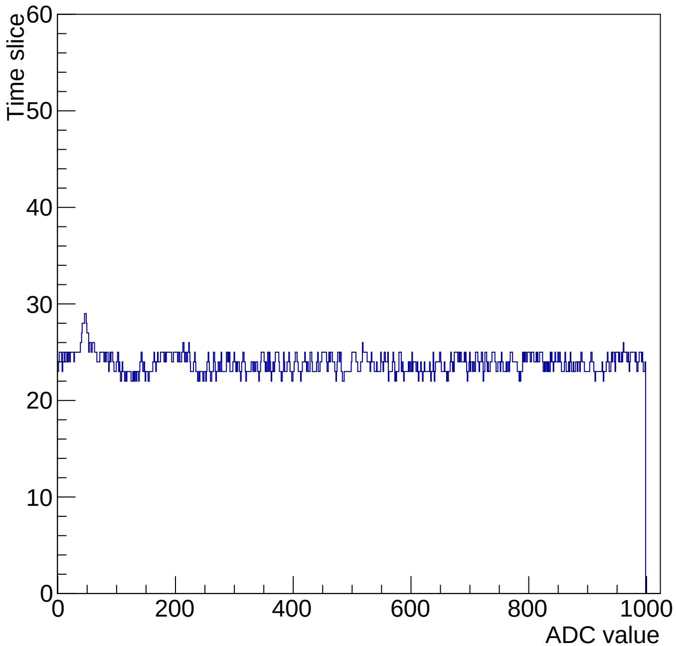
Evt 10 Time mcm 2004 chip 4 chan 9 1000-gain3-shaper0
