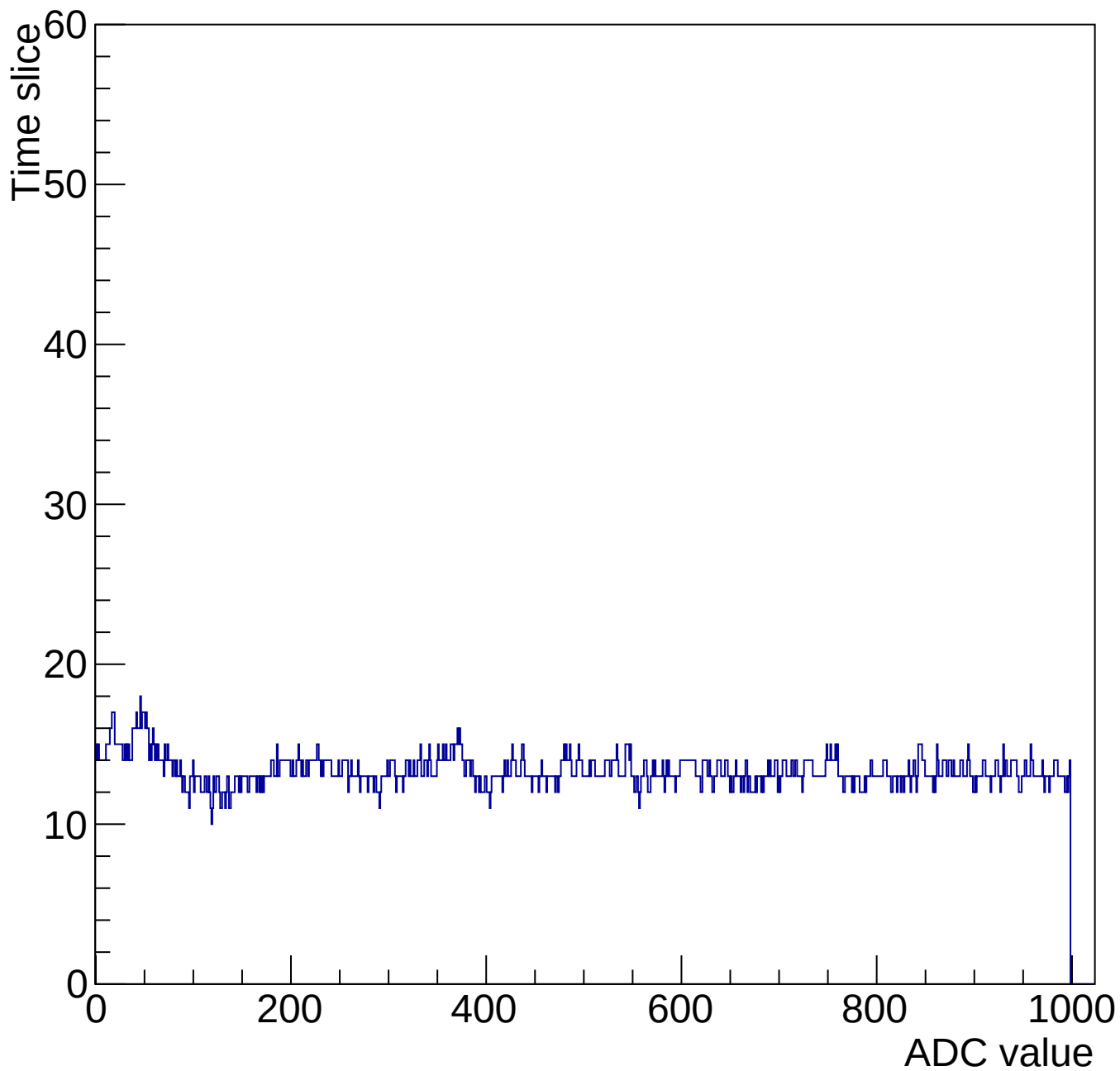
Evt 10 Time mcm 2004 chip 4 chan 10 1000-gain3-shaper0
