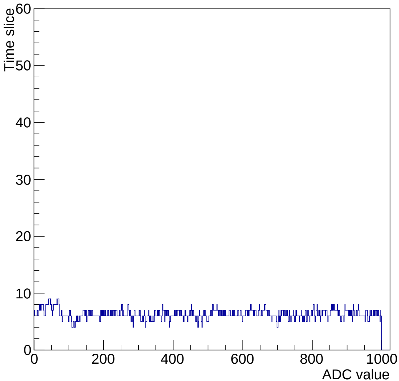
Evt 10 Time mcm 2004 chip 4 chan 5 1000-gain3-shaper0
