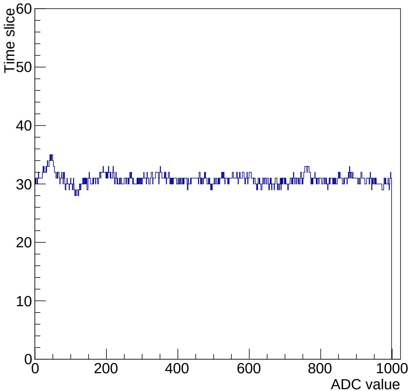
Evt 10 Time mcm 2004 chip 4 chan 7 1000-gain3-shaper0
