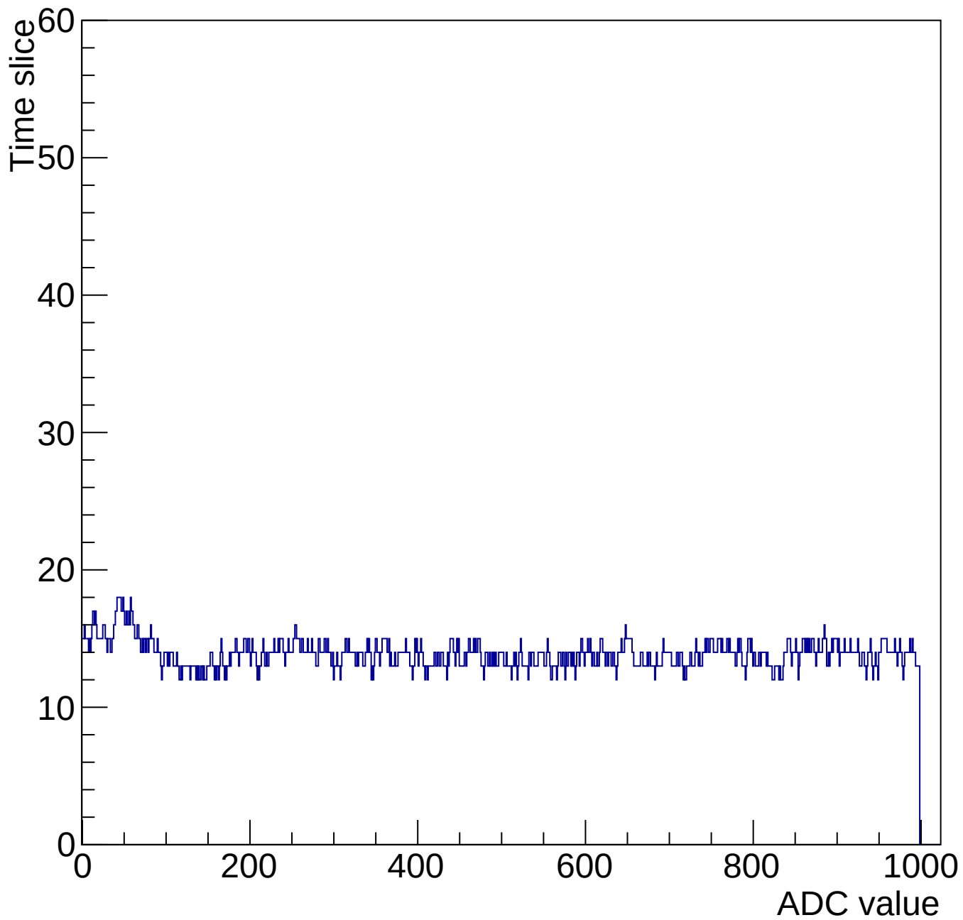
Evt 10 Time mcm 2004 chip 4 chan 14 1000-gain3-shaper0
