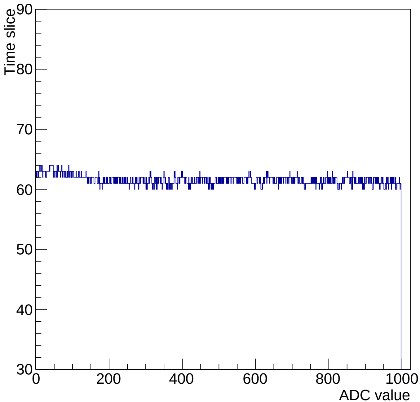
Evt 10 Time mcm 2005 chip 5 chan 10 1000-gain0-shaper0
