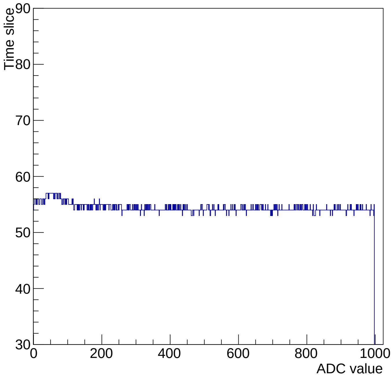
Evt 10 Time mcm 2005 chip 5 chan 4 1000-gain0-shaper0
