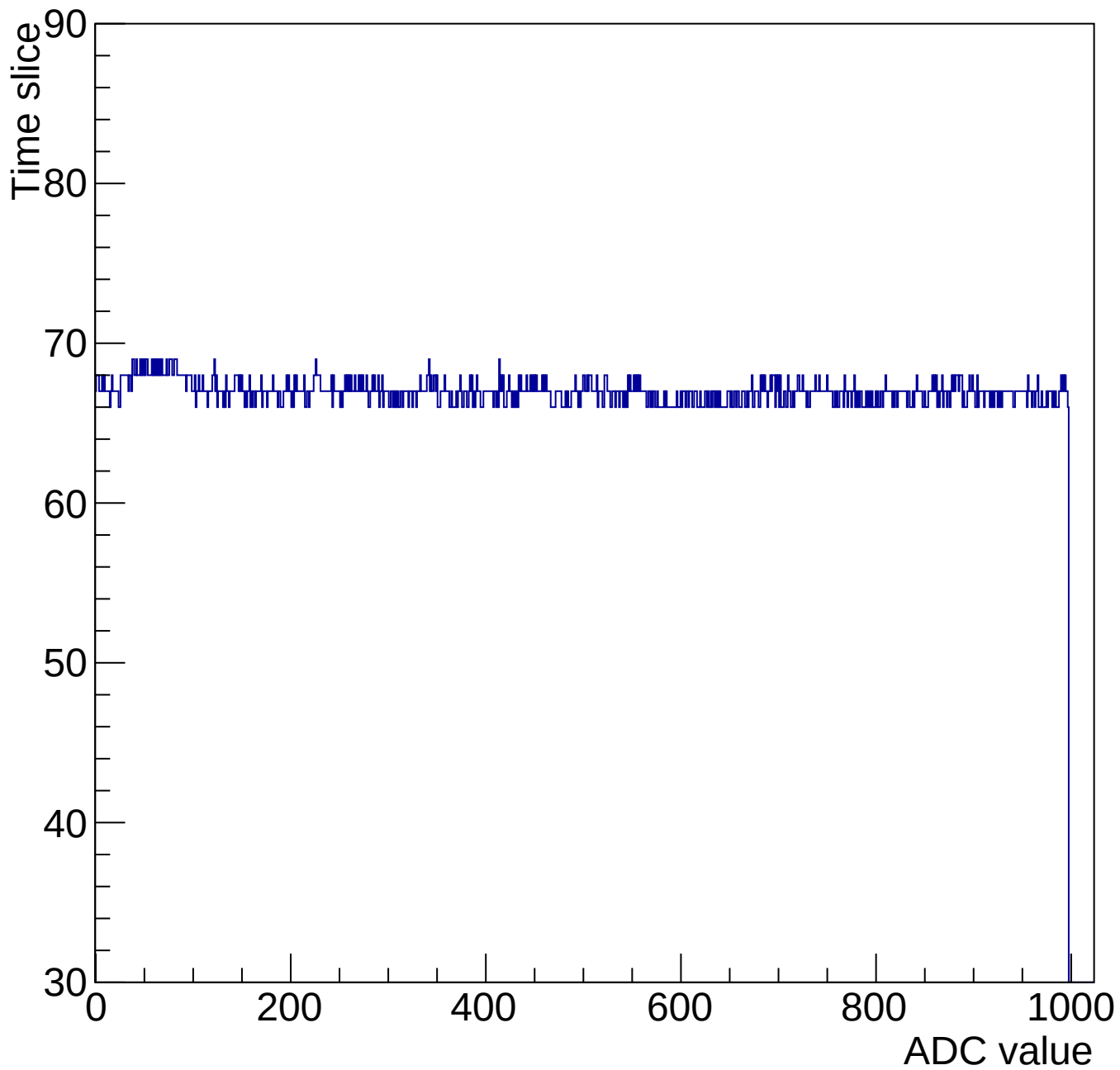
Evt 10 Time mcm 2005 chip 5 chan 1 1000-gain0-shaper0
