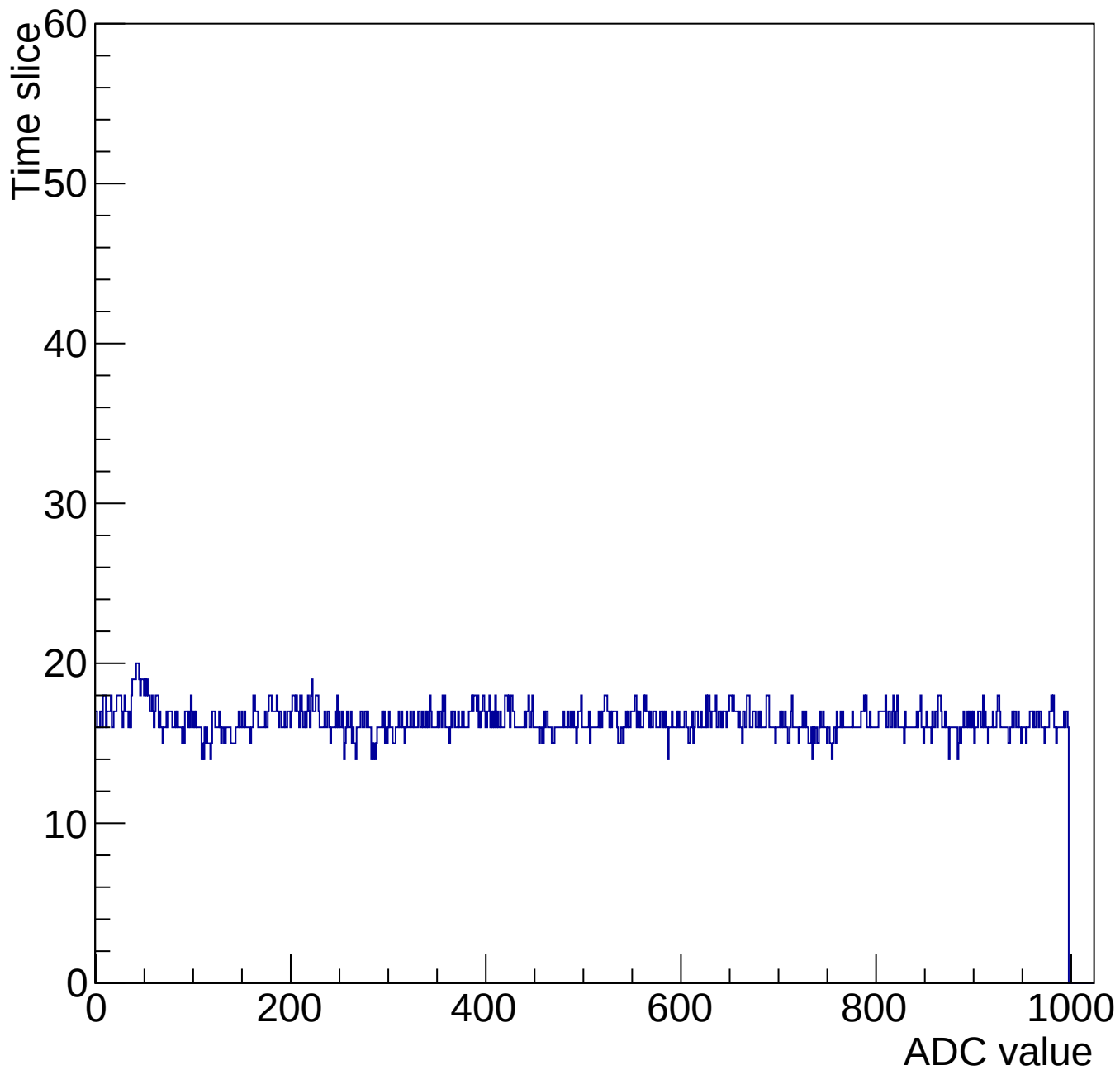
Evt 10 Time mcm 2005 chip 5 chan 10 1000-gain3-shaper0
