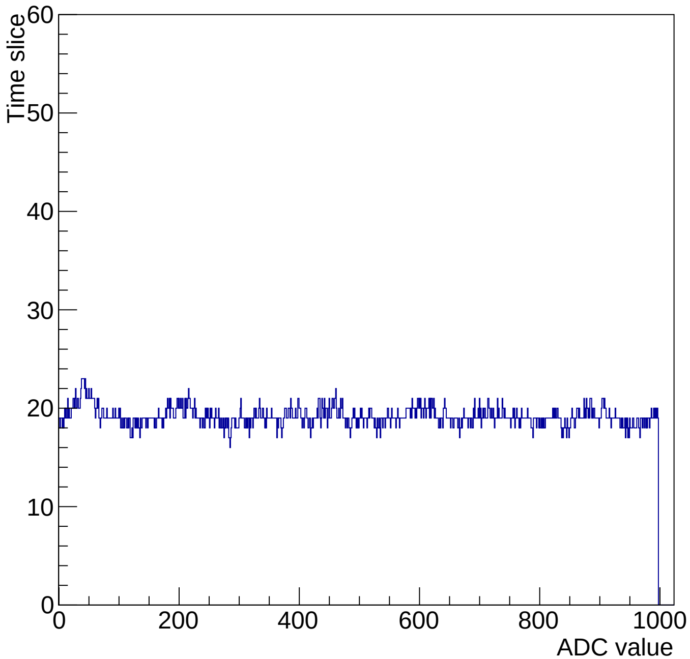
Evt 10 Time mcm 2005 chip 5 chan 8 1000-gain3-shaper0
