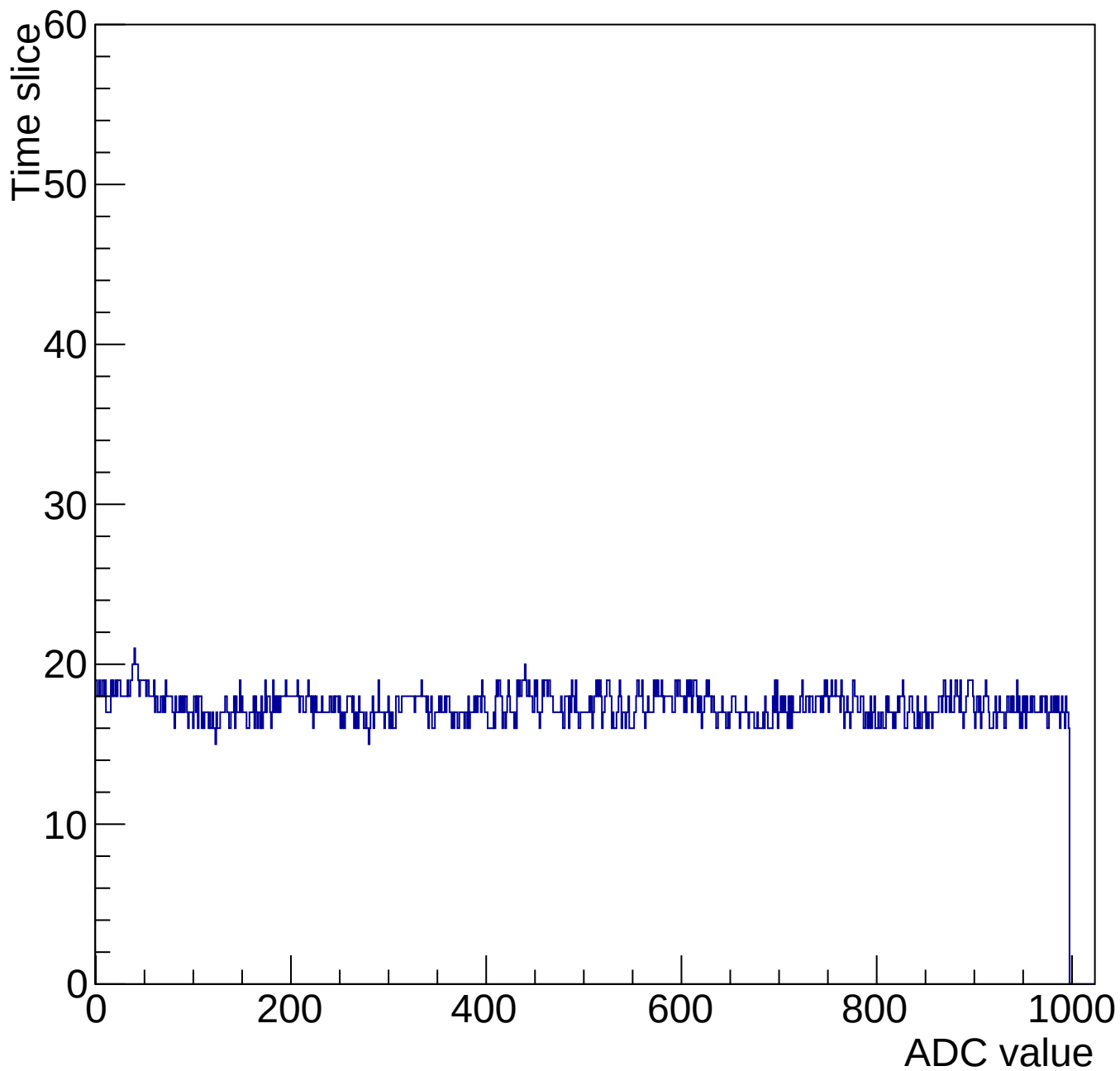
Evt 10 Time mcm 2005 chip 5 chan 9 1000-gain3-shaper0
