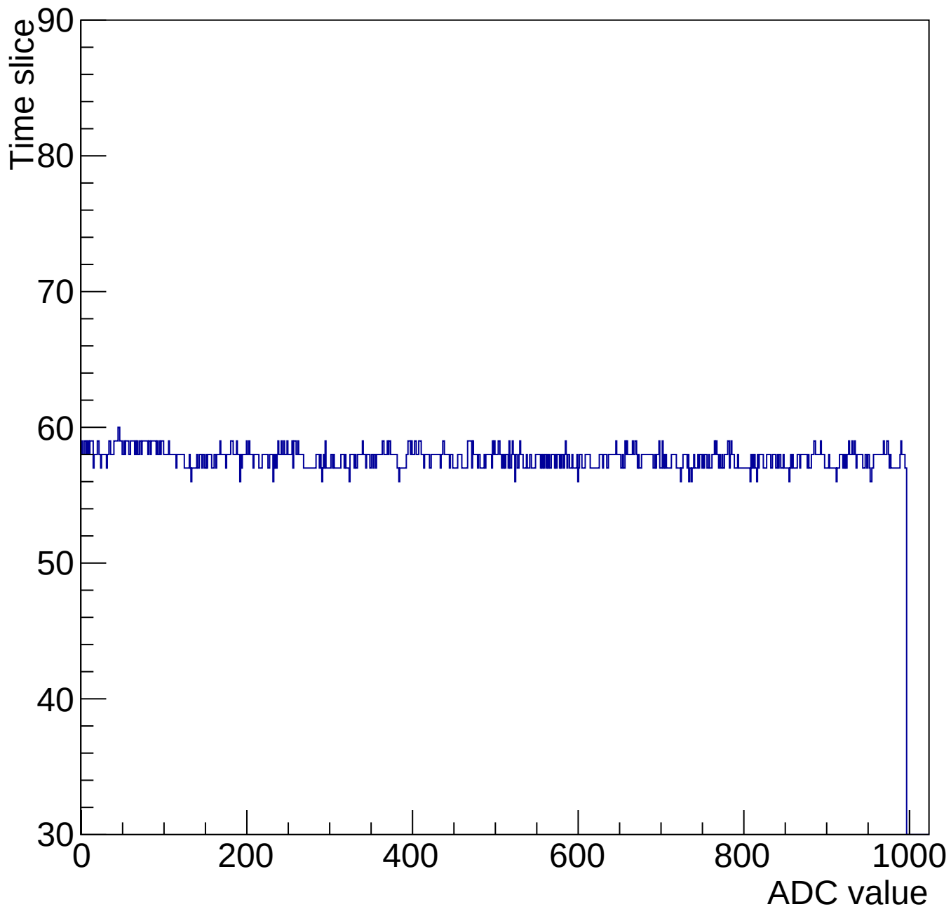
Evt 10 Time mcm 2006 chip 6 chan 12 1000-gain0-shaper0
