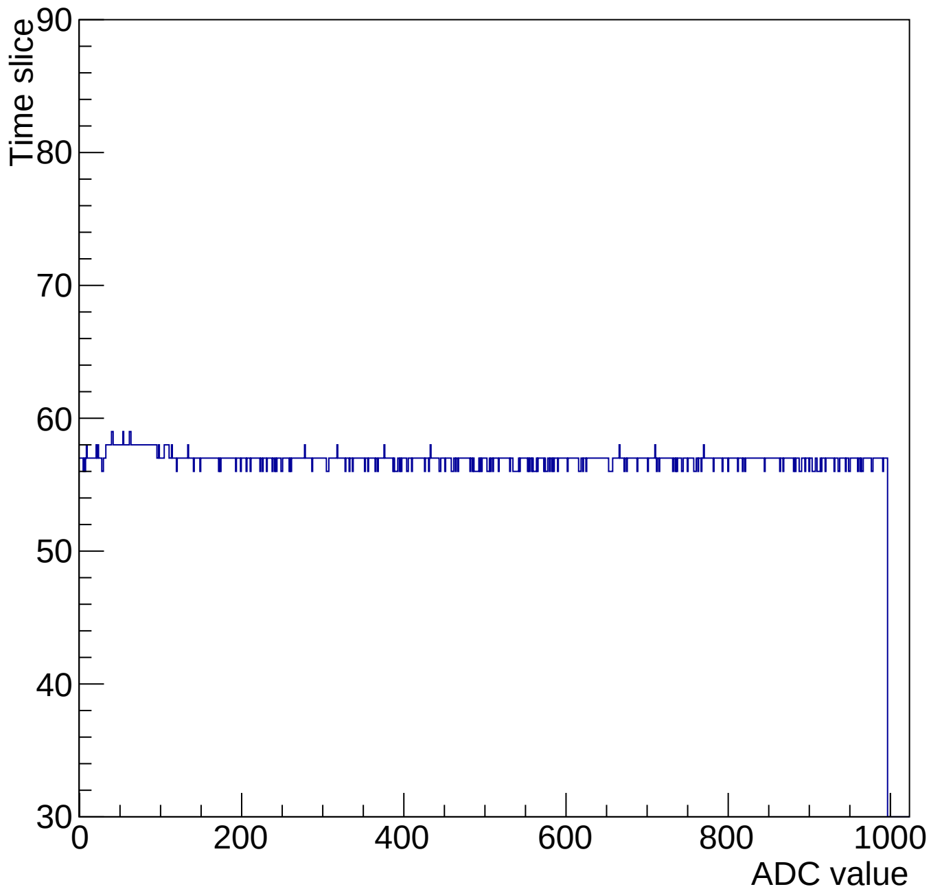
Evt 10 Time mcm 2006 chip 6 chan 10 1000-gain0-shaper0
