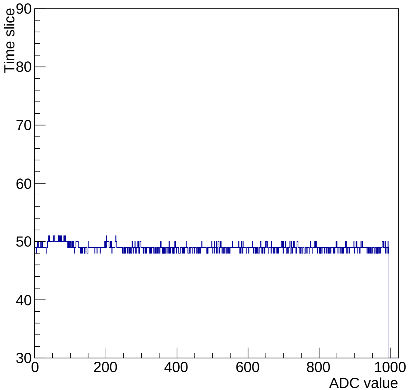
Evt 10 Time mcm 2006 chip 6 chan 8 1000-gain0-shaper0
