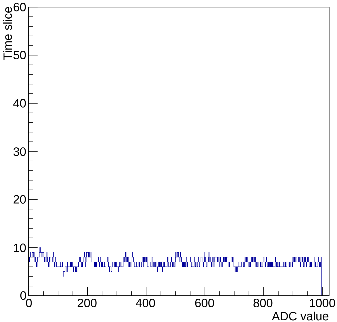
Evt 10 Time mcm 2006 chip 6 chan 10 1000-gain3-shaper0
