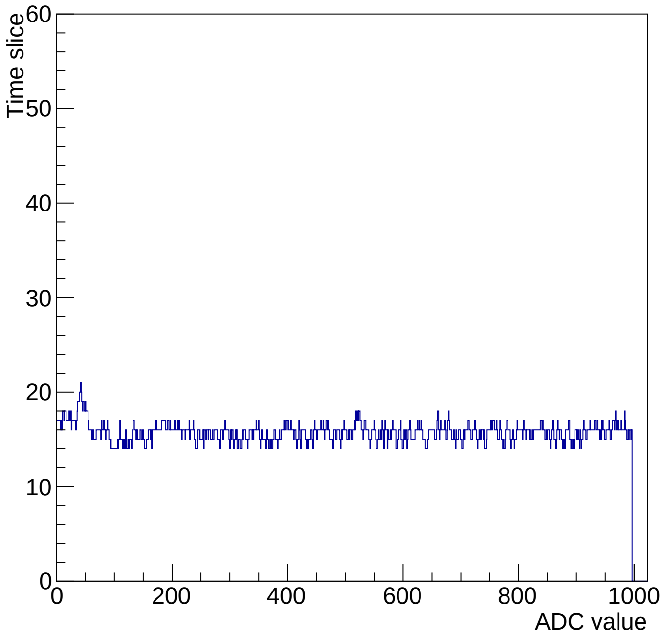
Evt 10 Time mcm 2006 chip 6 chan 2 1000-gain3-shaper0
