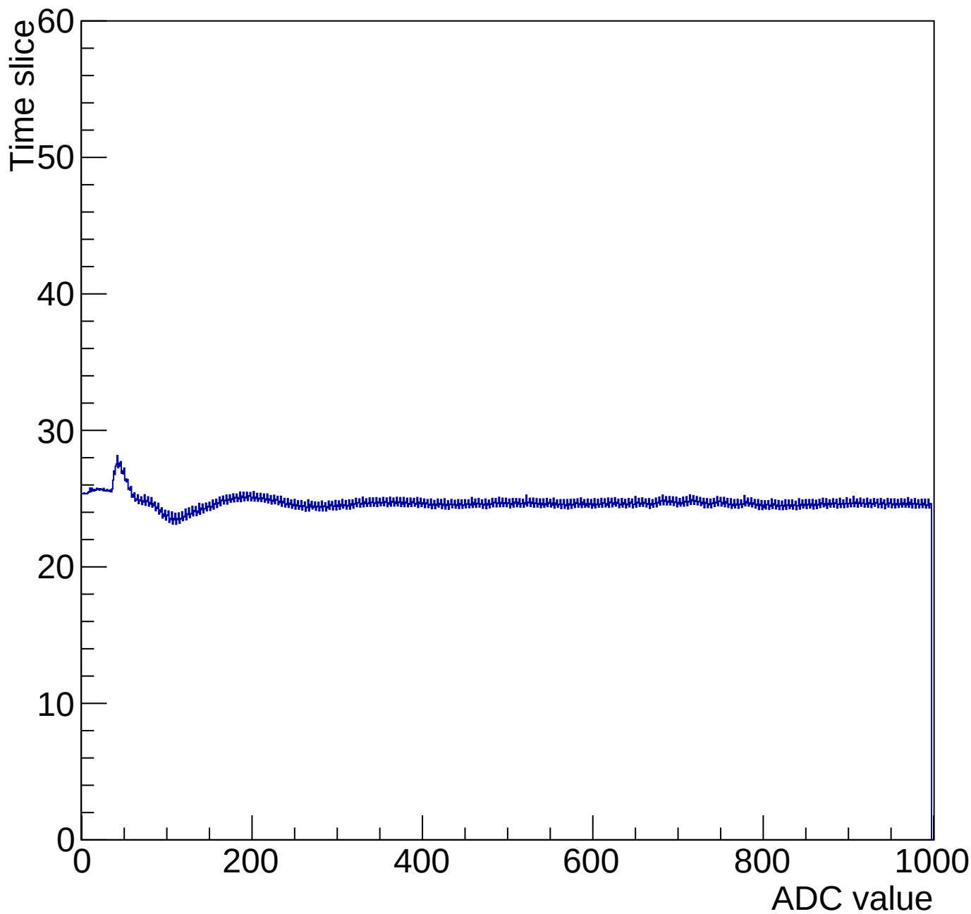
Time mcm 2001 chip 1 chan 10 1000-gain3-shaper0
