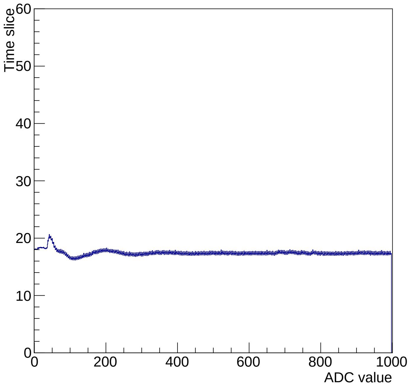
Time mcm 2001 chip 1 chan 5 1000-gain3-shaper0
