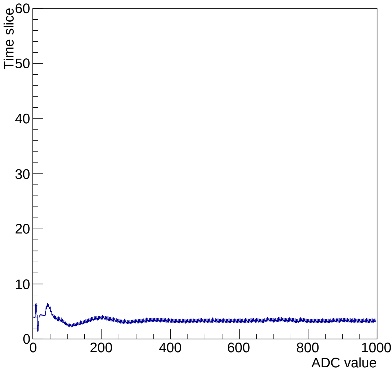
Time mcm 2001 chip 1 chan 14 1000-gain3-shaper0
