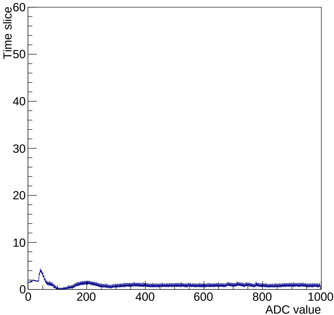
Time mcm 2001 chip 1 chan 1 1000-gain3-shaper0
