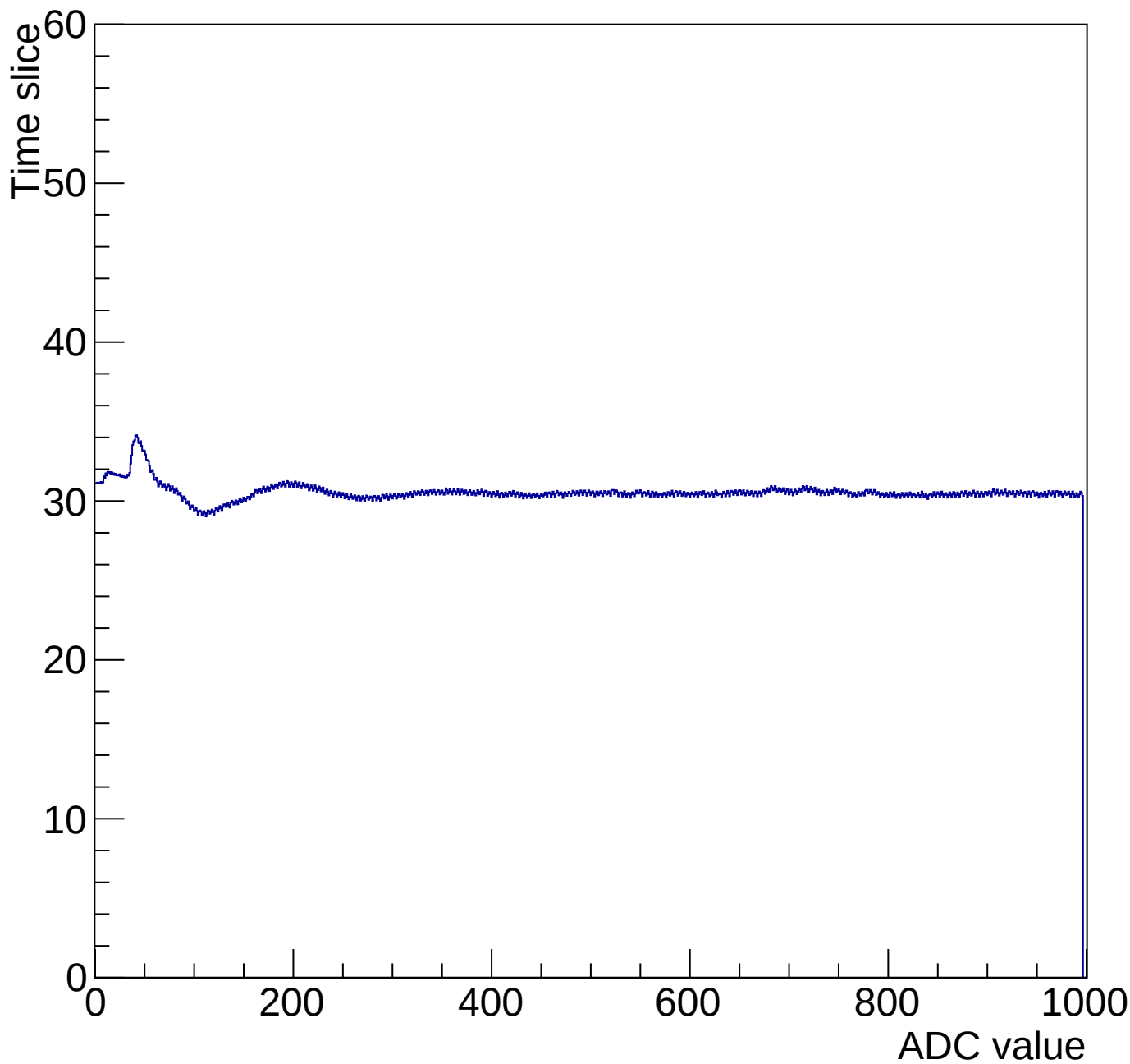
Time mcm 2002 chip 2 chan 4 1000-gain3-shaper0
