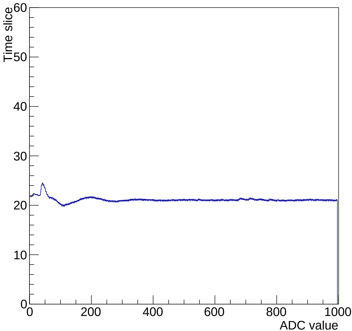
Time mcm 2002 chip 2 chan 5 1000-gain3-shaper0
