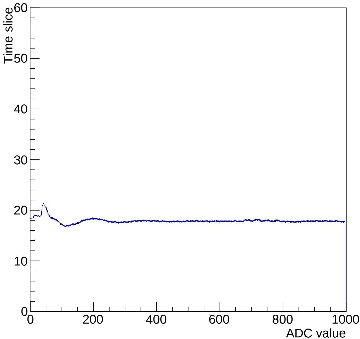
Time mcm 2002 chip 2 chan 7 1000-gain3-shaper0
