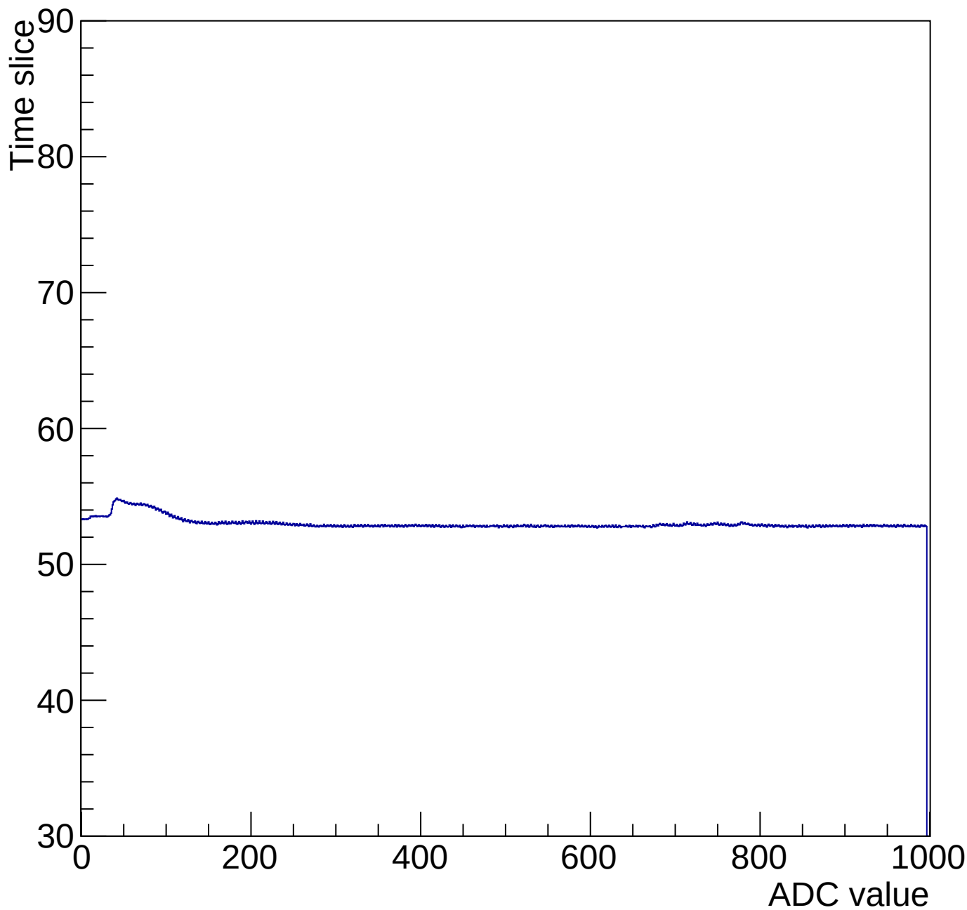
Time mcm 2002 chip 2 chan 12 1000-gain0-shaper0
