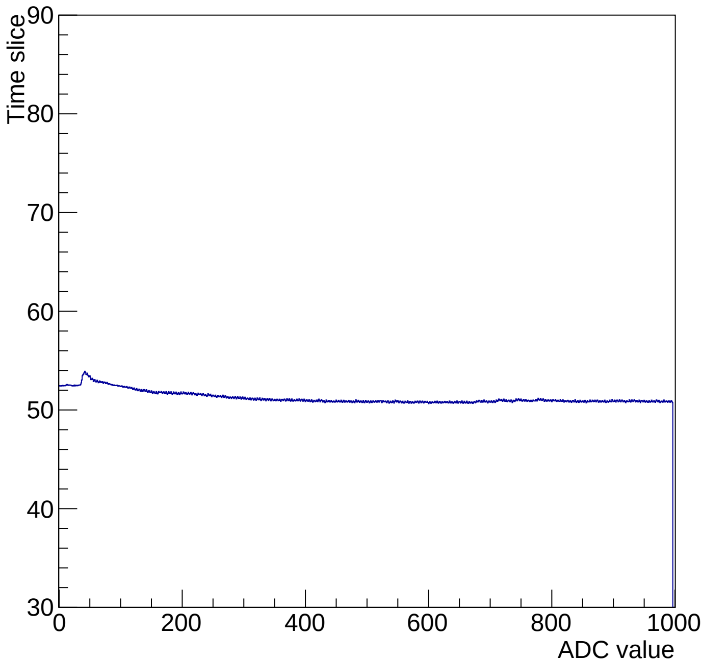
Time mcm 2002 chip 2 chan 2 1000-gain0-shaper0
