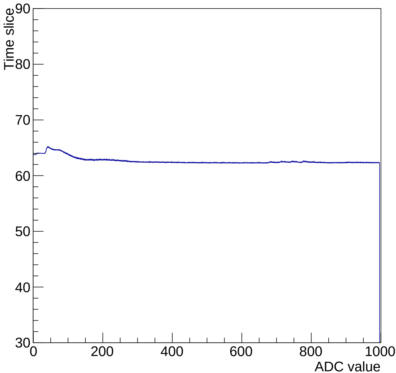
Time mcm 2002 chip 2 chan 7 1000-gain0-shaper0
