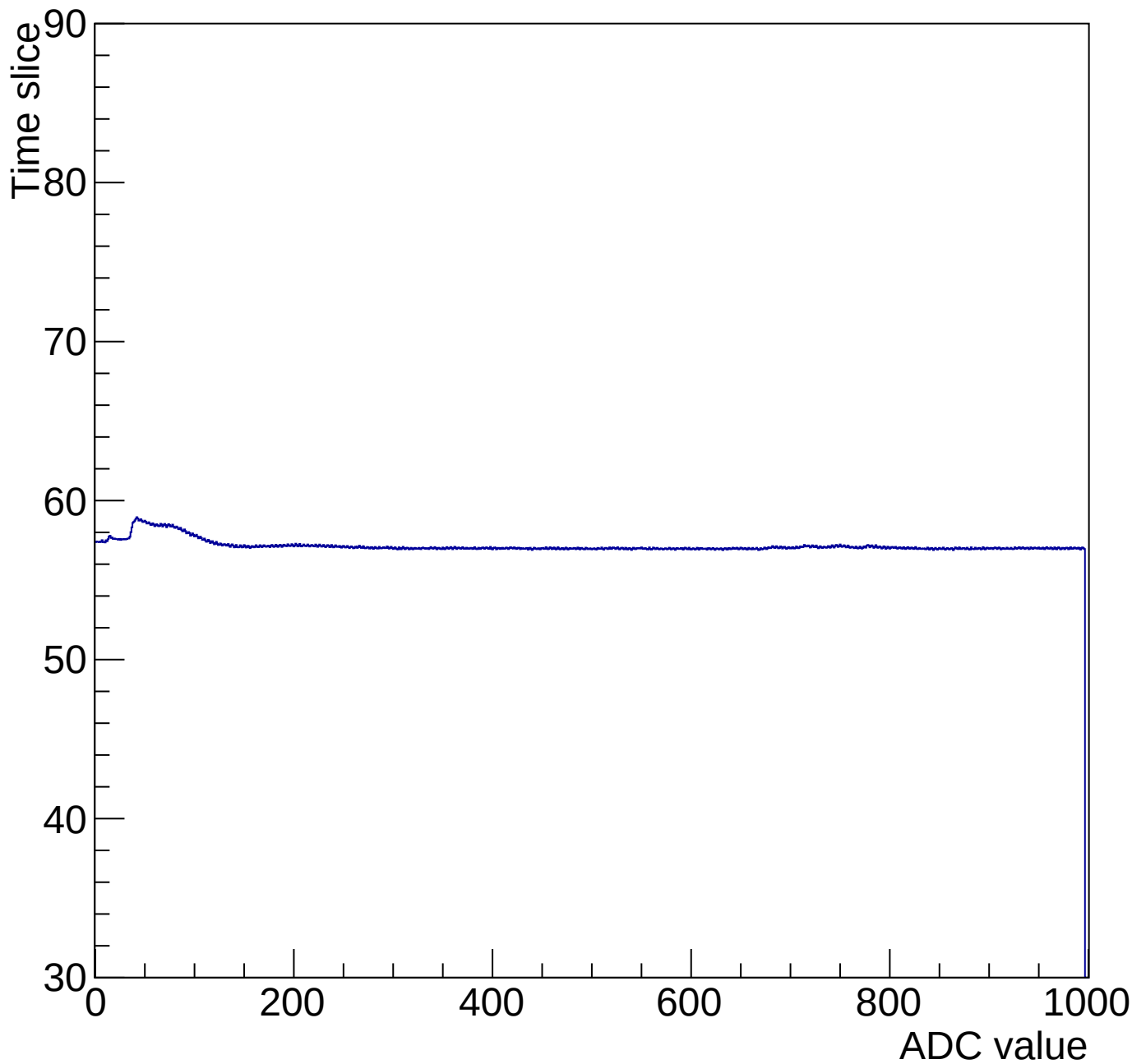
Time mcm 2002 chip 2 chan 15 1000-gain0-shaper0
