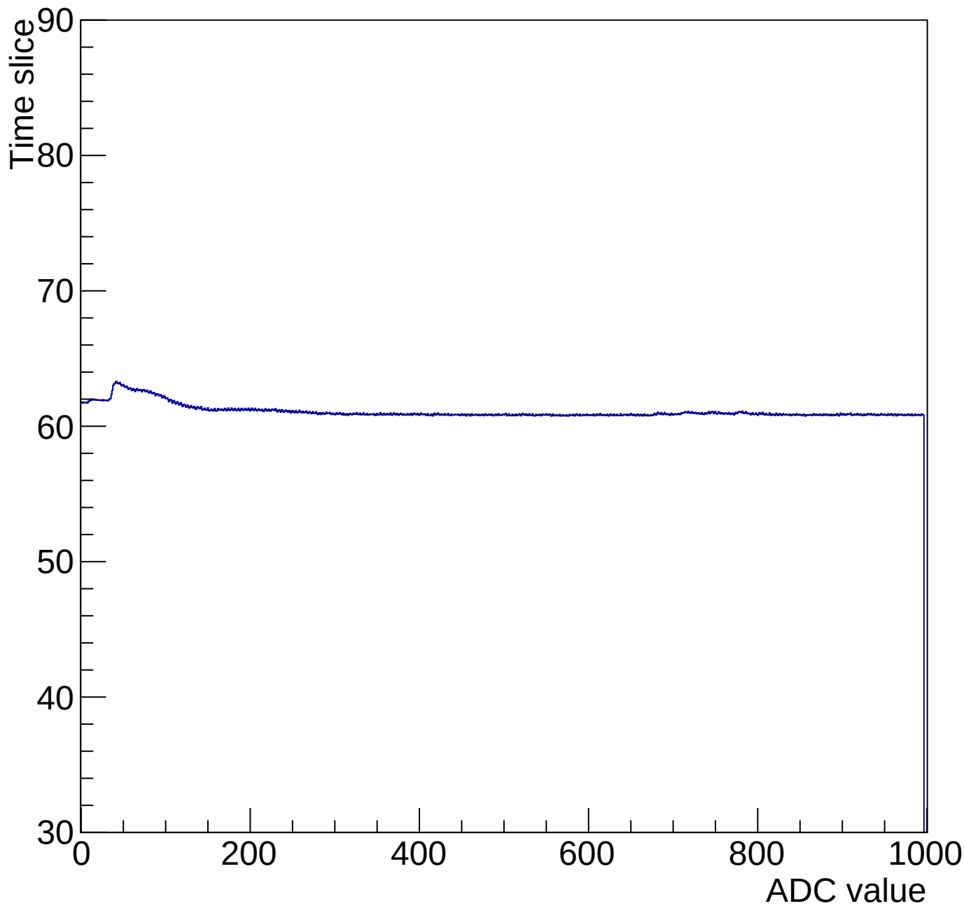
Time mcm 2002 chip 2 chan 11 1000-gain0-shaper0
