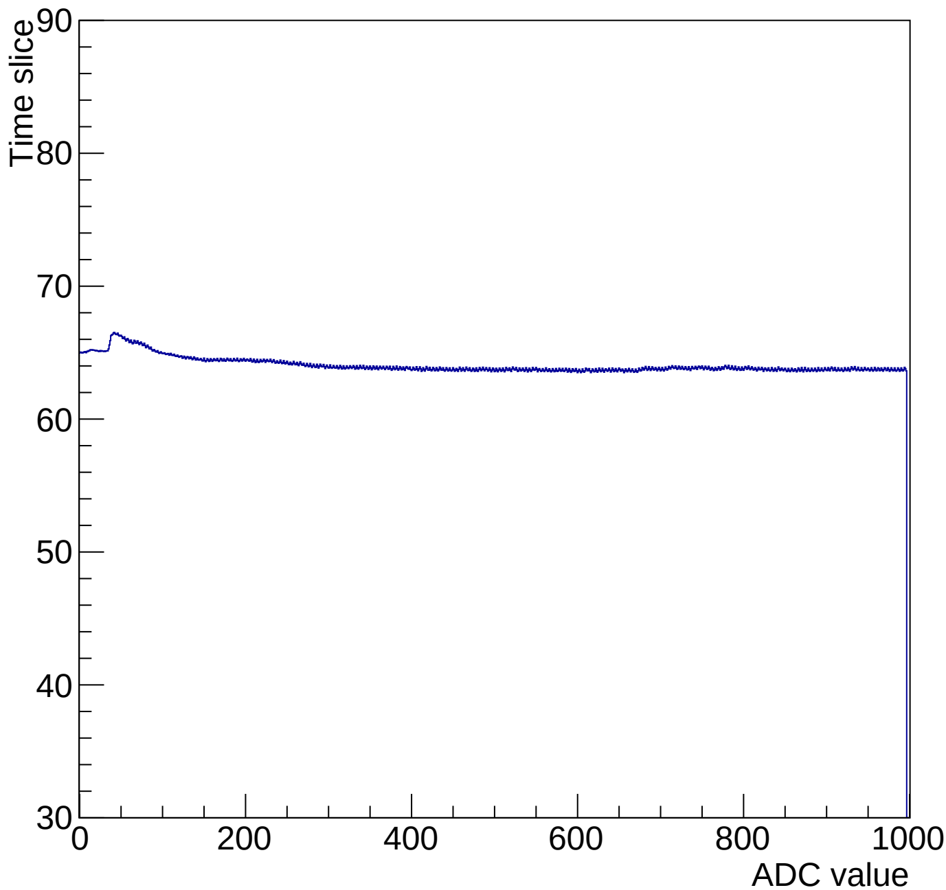
Time mcm 2002 chip 2 chan 0 1000-gain0-shaper0
