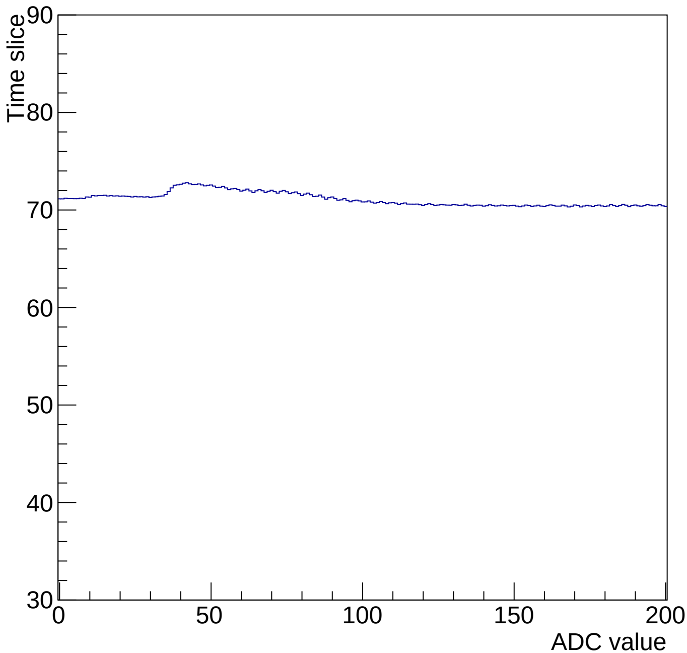
Time mcm 2002 chip 2 chan 4 200-gain0-shaper0
