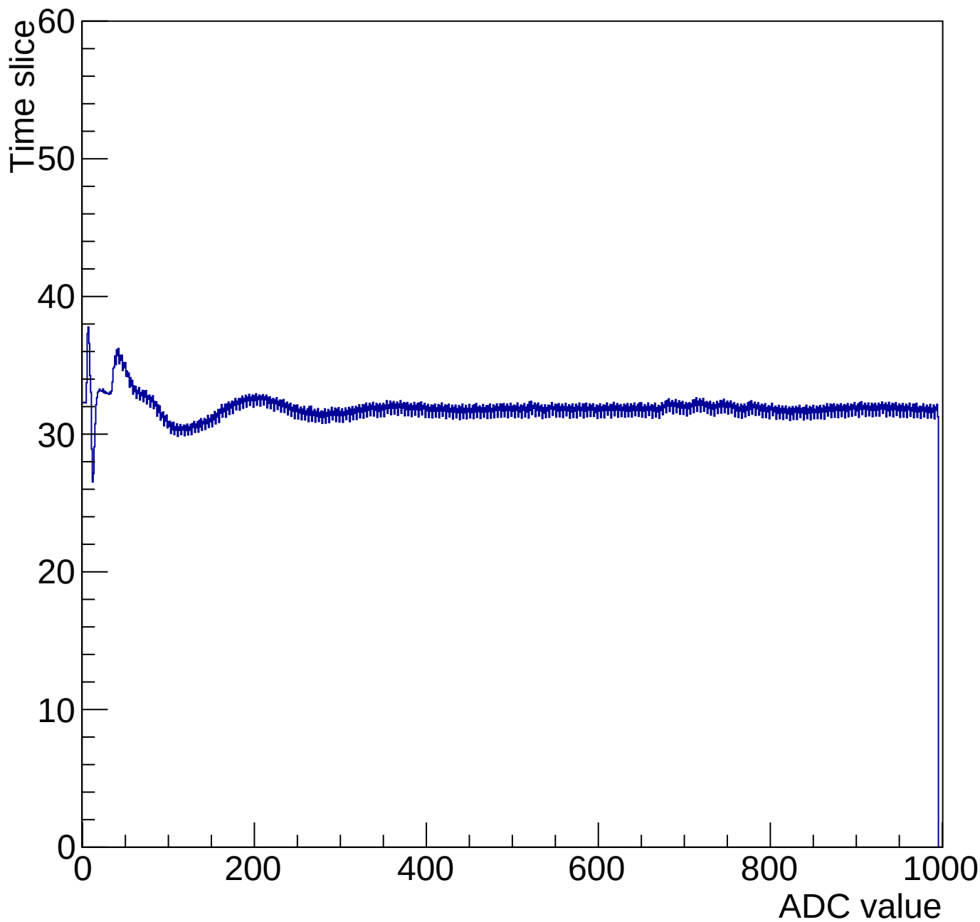
Time mcm 2003 chip 3 chan 0 1000-gain3-shaper0
