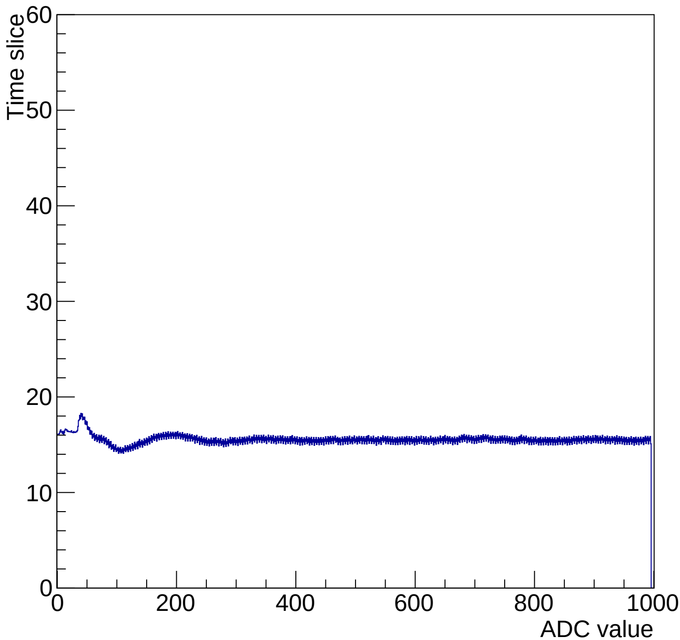
Time mcm 2003 chip 3 chan 15 1000-gain3-shaper0
