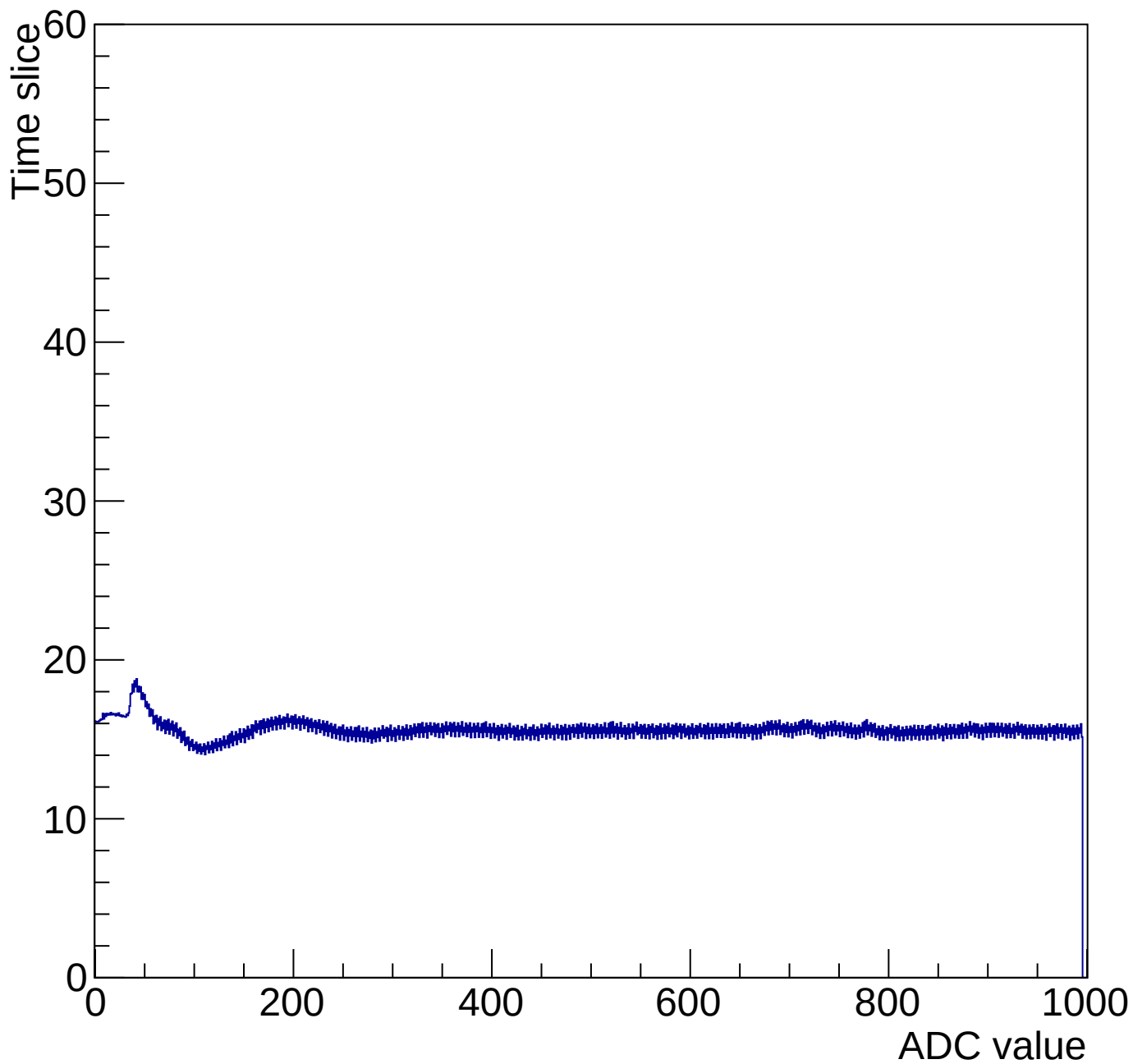
Time mcm 2003 chip 3 chan 8 1000-gain3-shaper0
