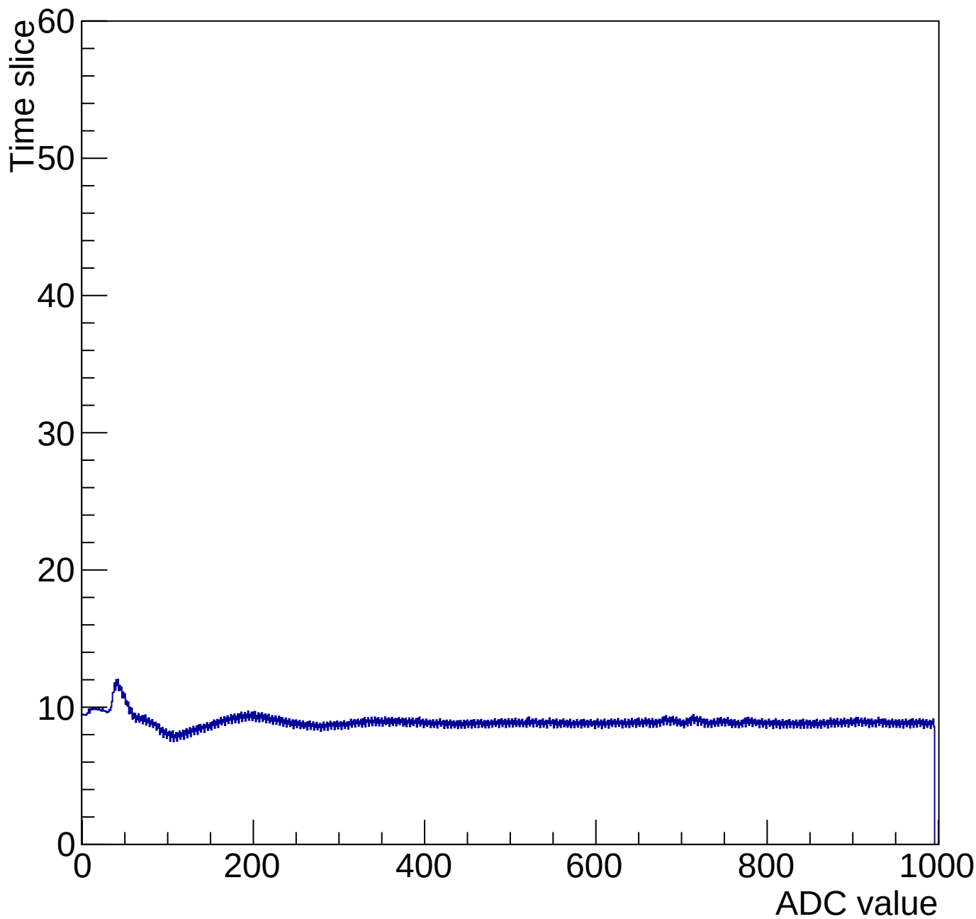
Time mcm 2003 chip 3 chan 3 1000-gain3-shaper0
