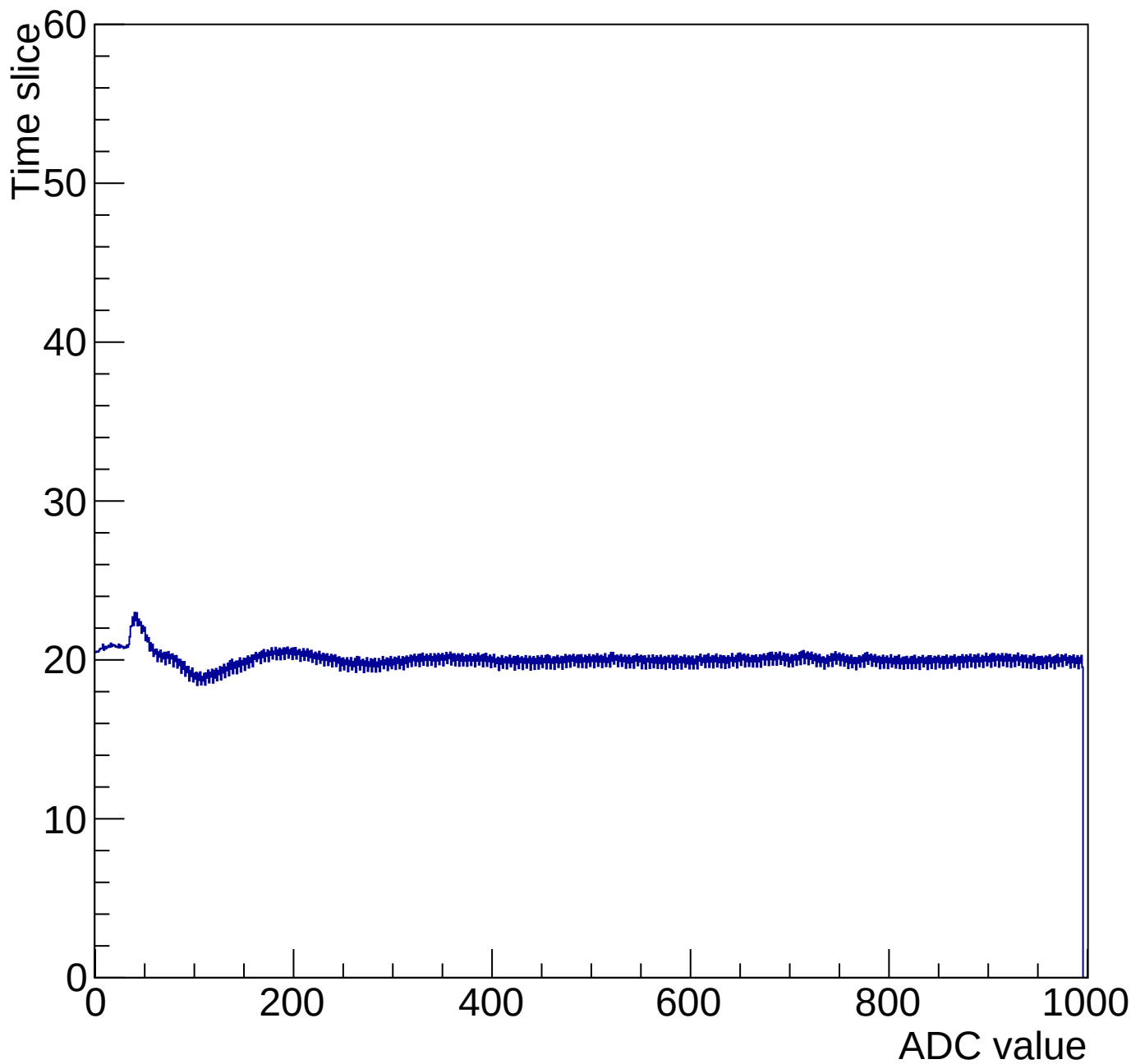
Time mcm 2003 chip 3 chan 2 1000-gain3-shaper0
