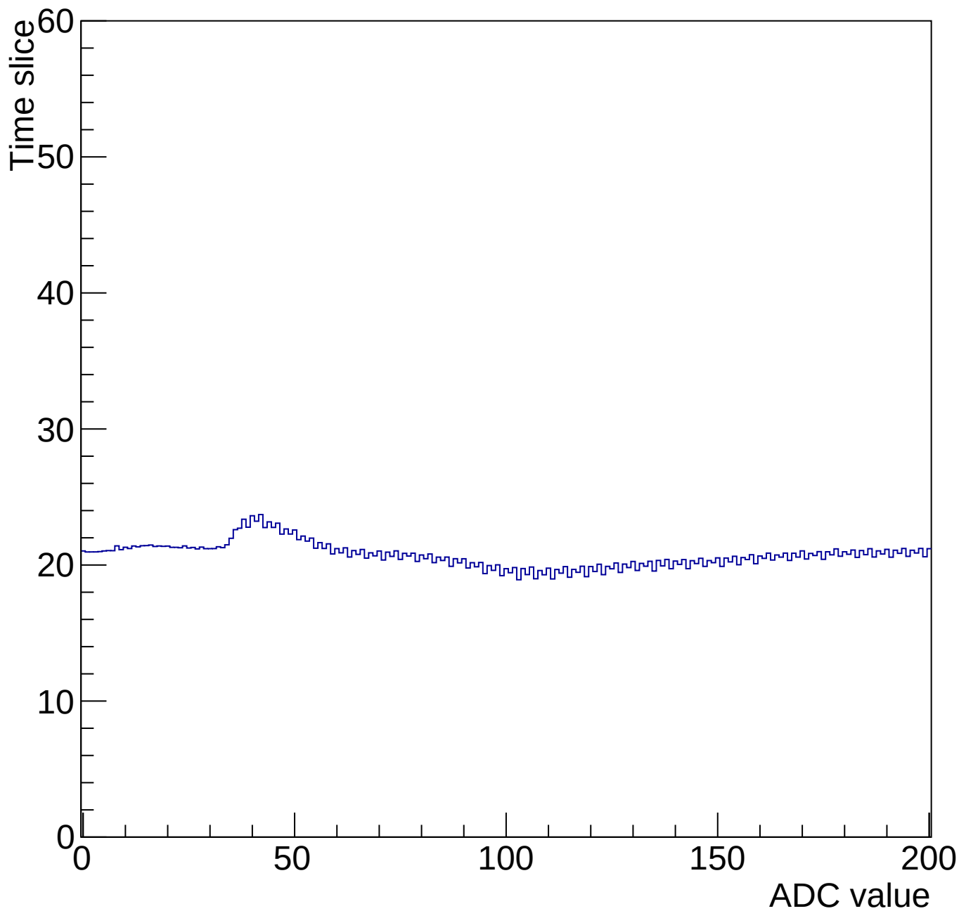
Time mcm 2003 chip 3 chan 11 200-gain3-shaper0
