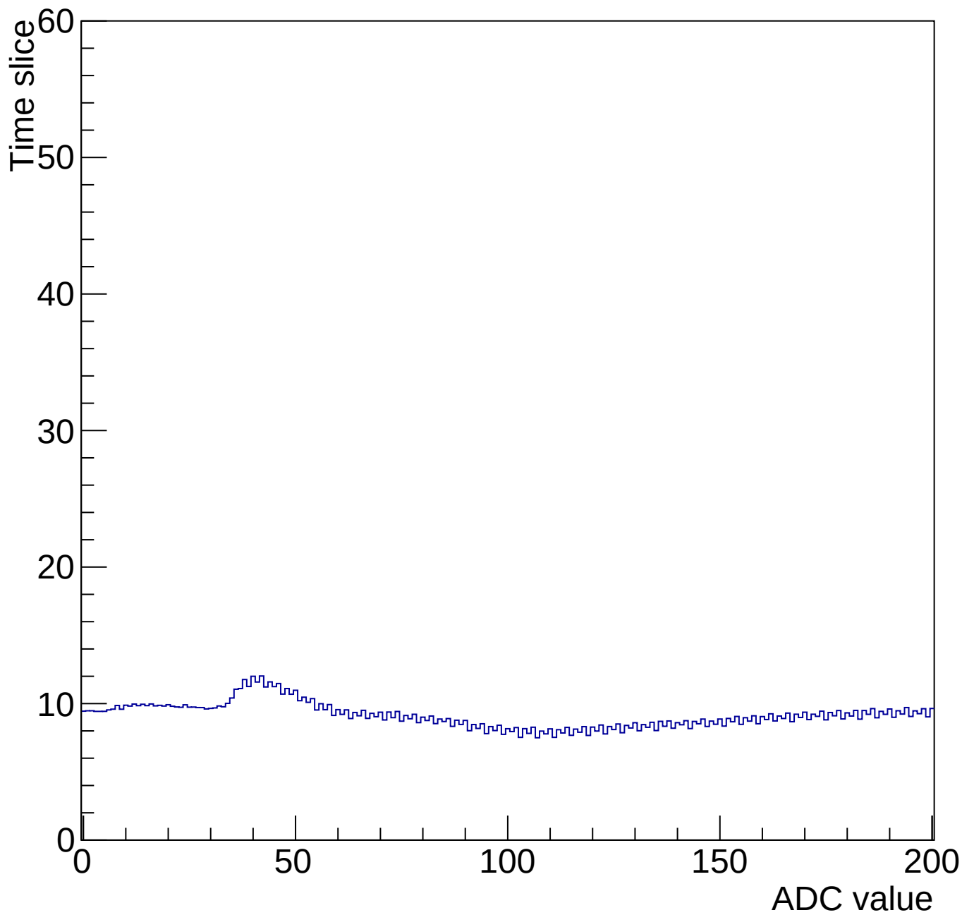
Time mcm 2003 chip 3 chan 3 200-gain3-shaper0
