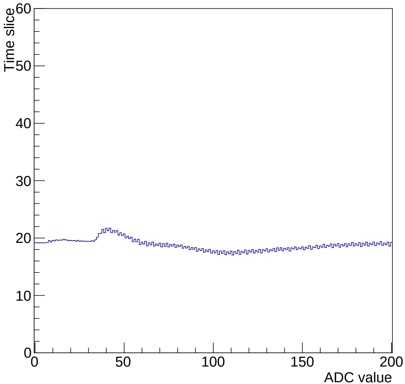
Time mcm 2003 chip 3 chan 9 200-gain3-shaper0
