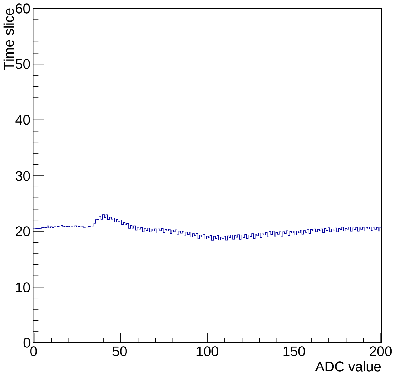
Time mcm 2003 chip 3 chan 2 200-gain3-shaper0
