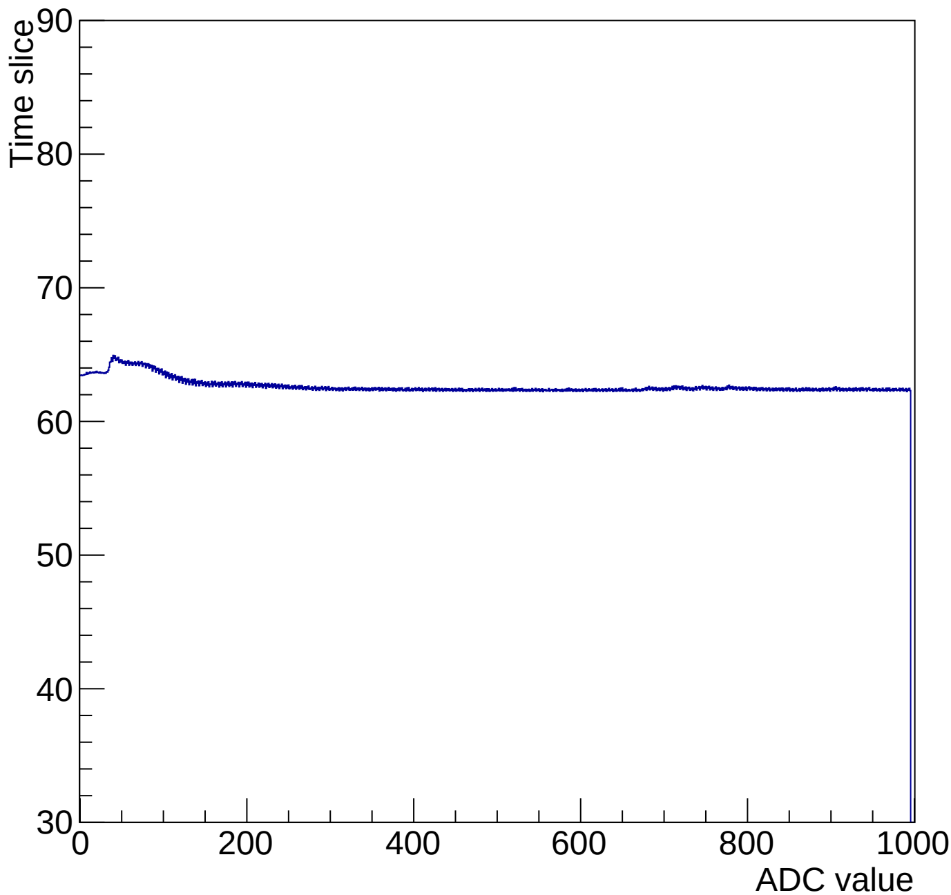
Time mcm 2003 chip 3 chan 11 1000-gain0-shaper0
