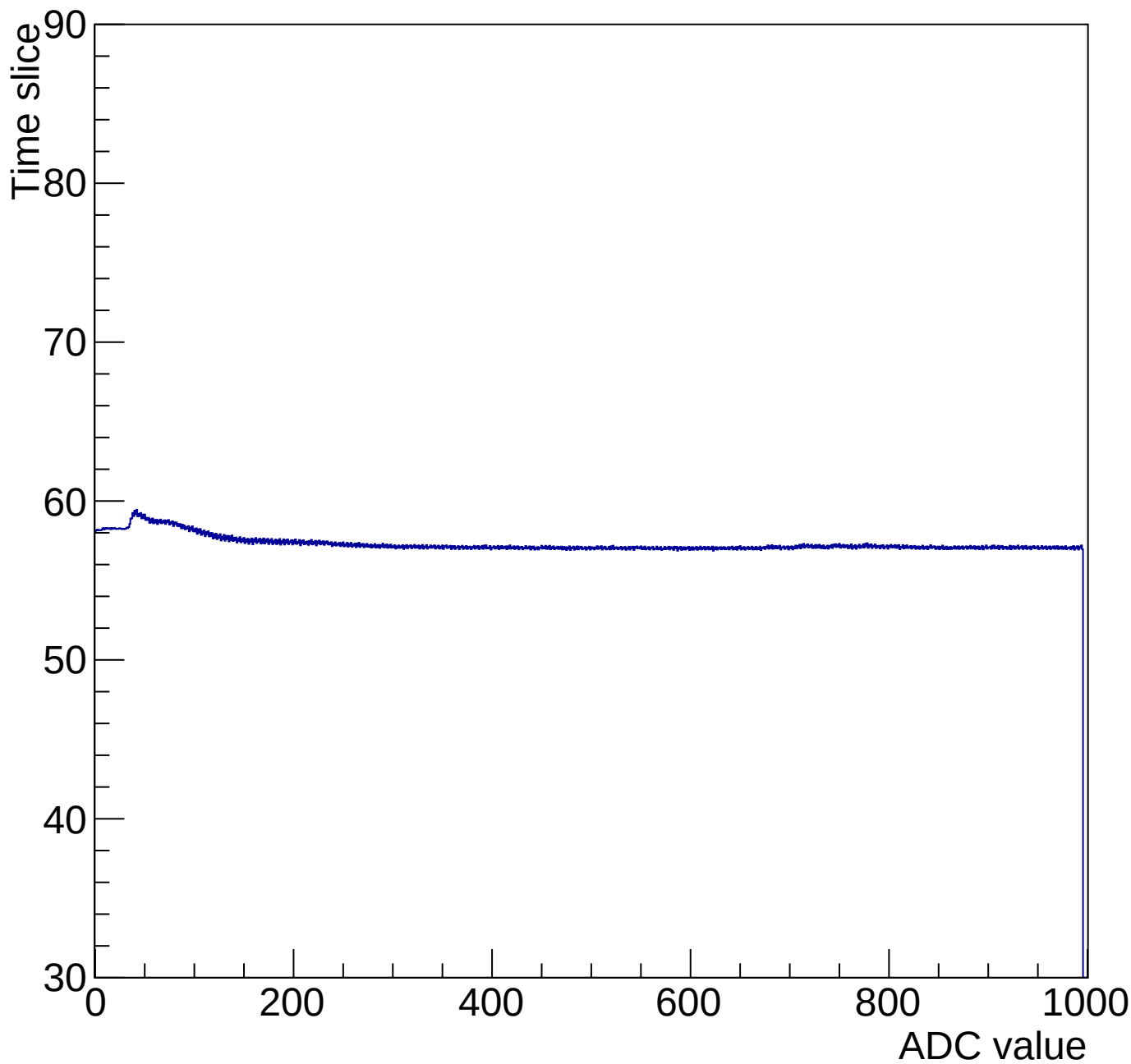
Time mcm 2003 chip 3 chan 7 1000-gain0-shaper0
