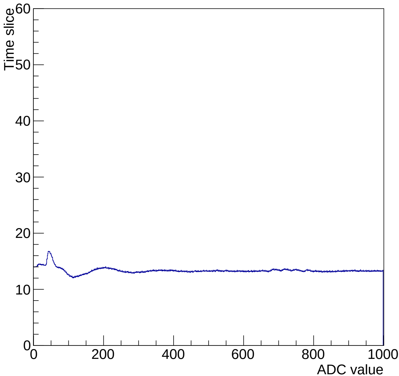
Time mcm 2004 chip 4 chan 10 1000-gain3-shaper0
