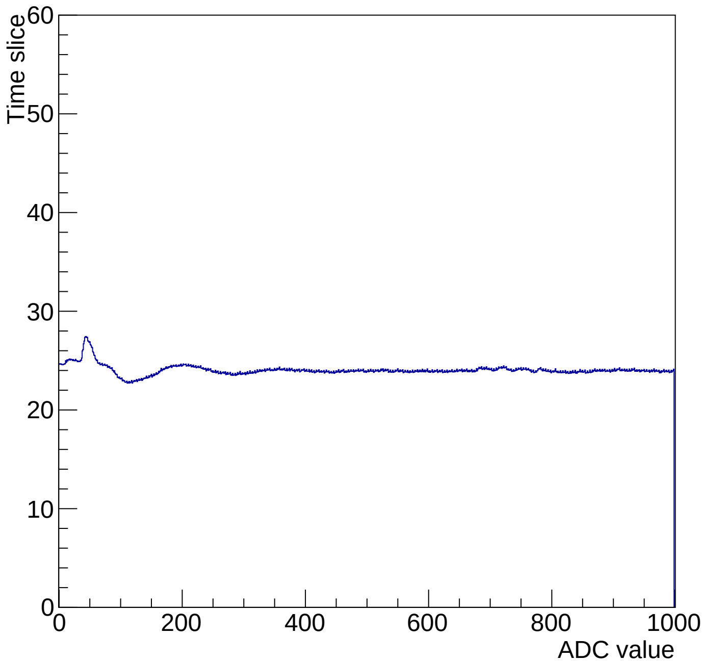
Time mcm 2004 chip 4 chan 9 1000-gain3-shaper0
