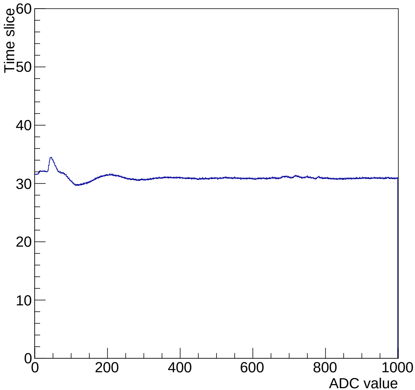
Time mcm 2004 chip 4 chan 7 1000-gain3-shaper0
