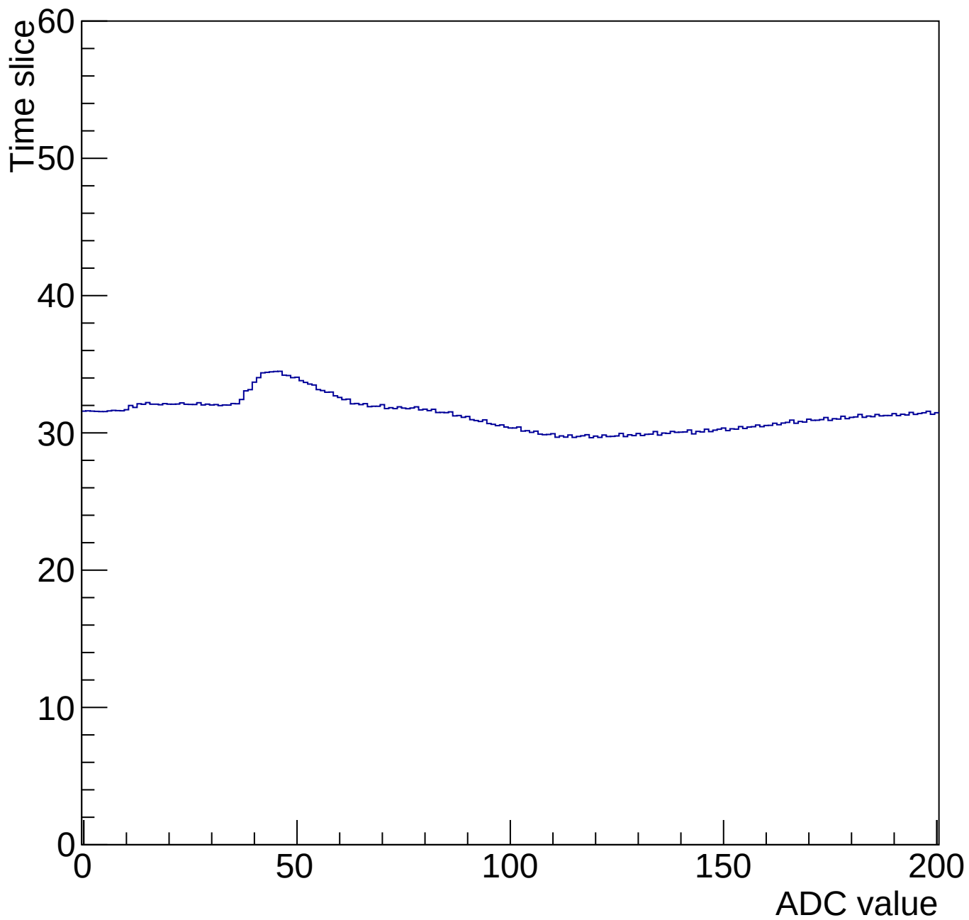
Time mcm 2004 chip 4 chan 7 200-gain3-shaper0
