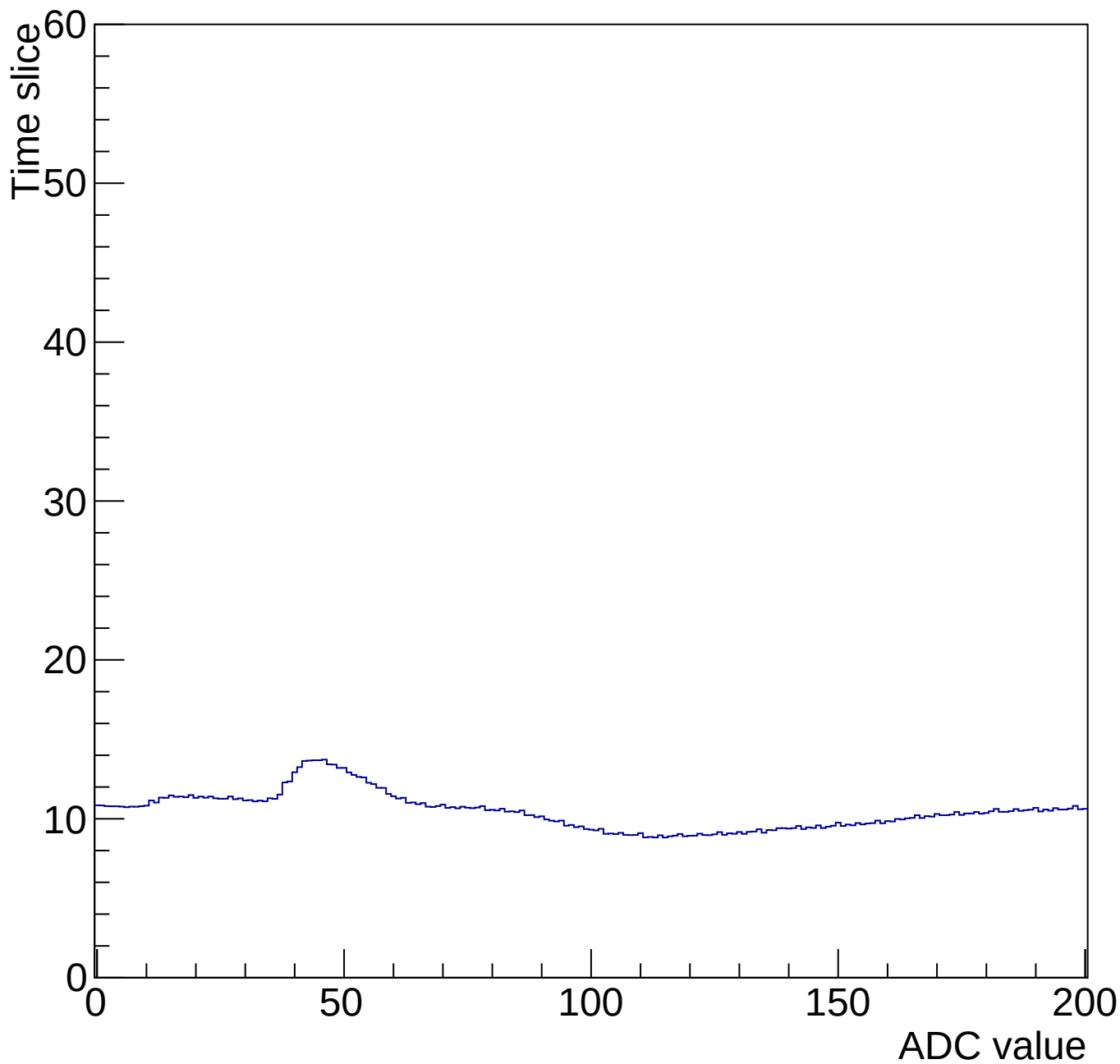
Time mcm 2004 chip 4 chan 4 200-gain3-shaper0
