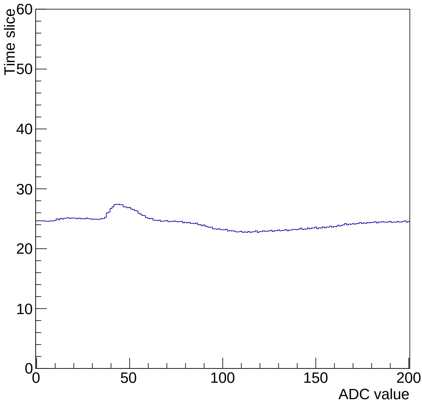
Time mcm 2004 chip 4 chan 9 200-gain3-shaper0
