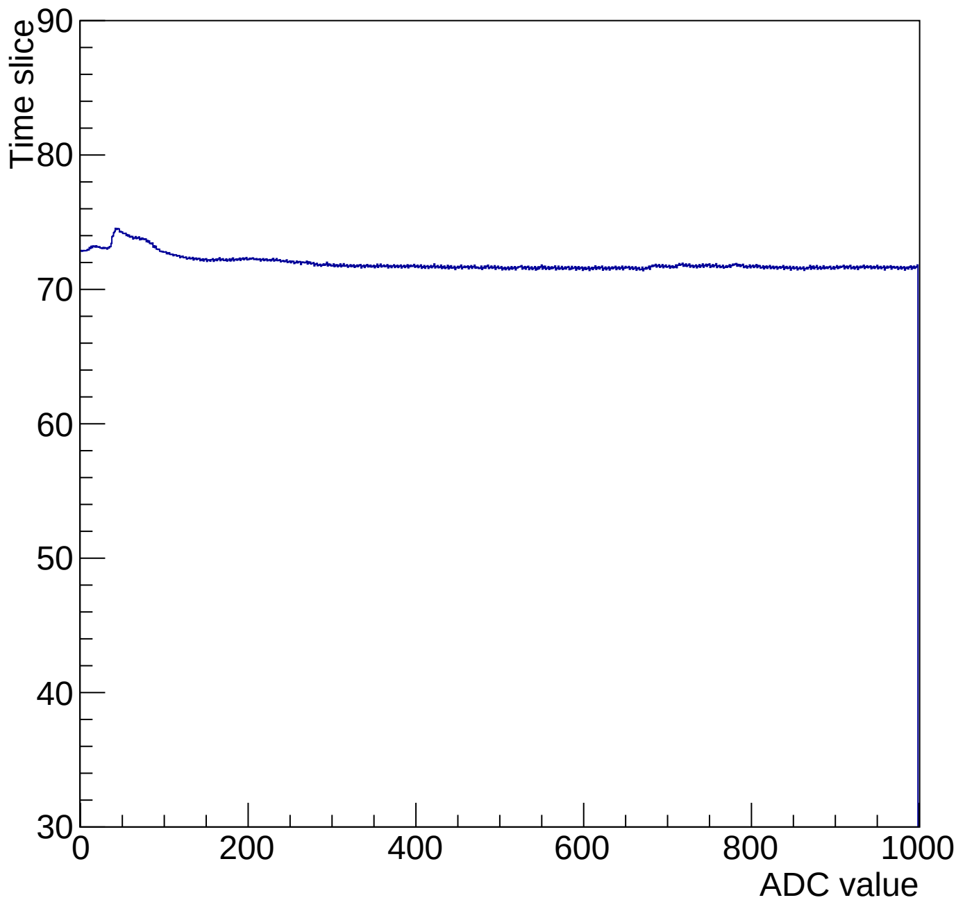
Time mcm 2004 chip 4 chan 0 1000-gain0-shaper0
