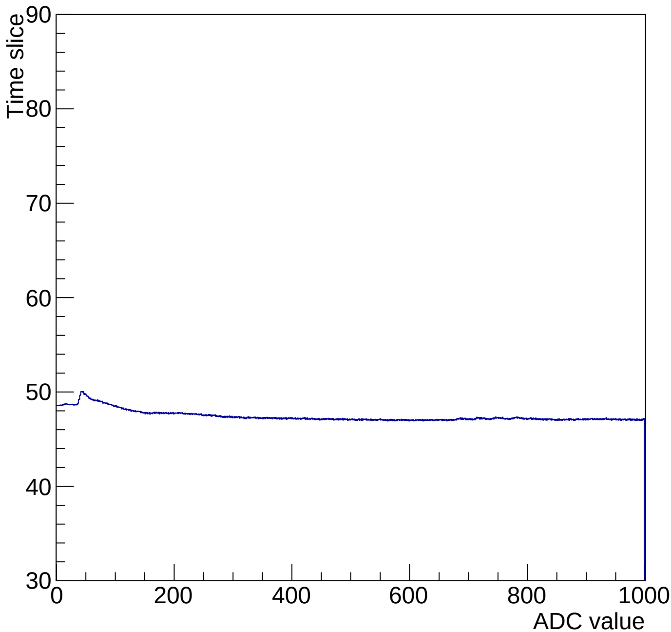
Time mcm 2004 chip 4 chan 6 1000-gain0-shaper0
