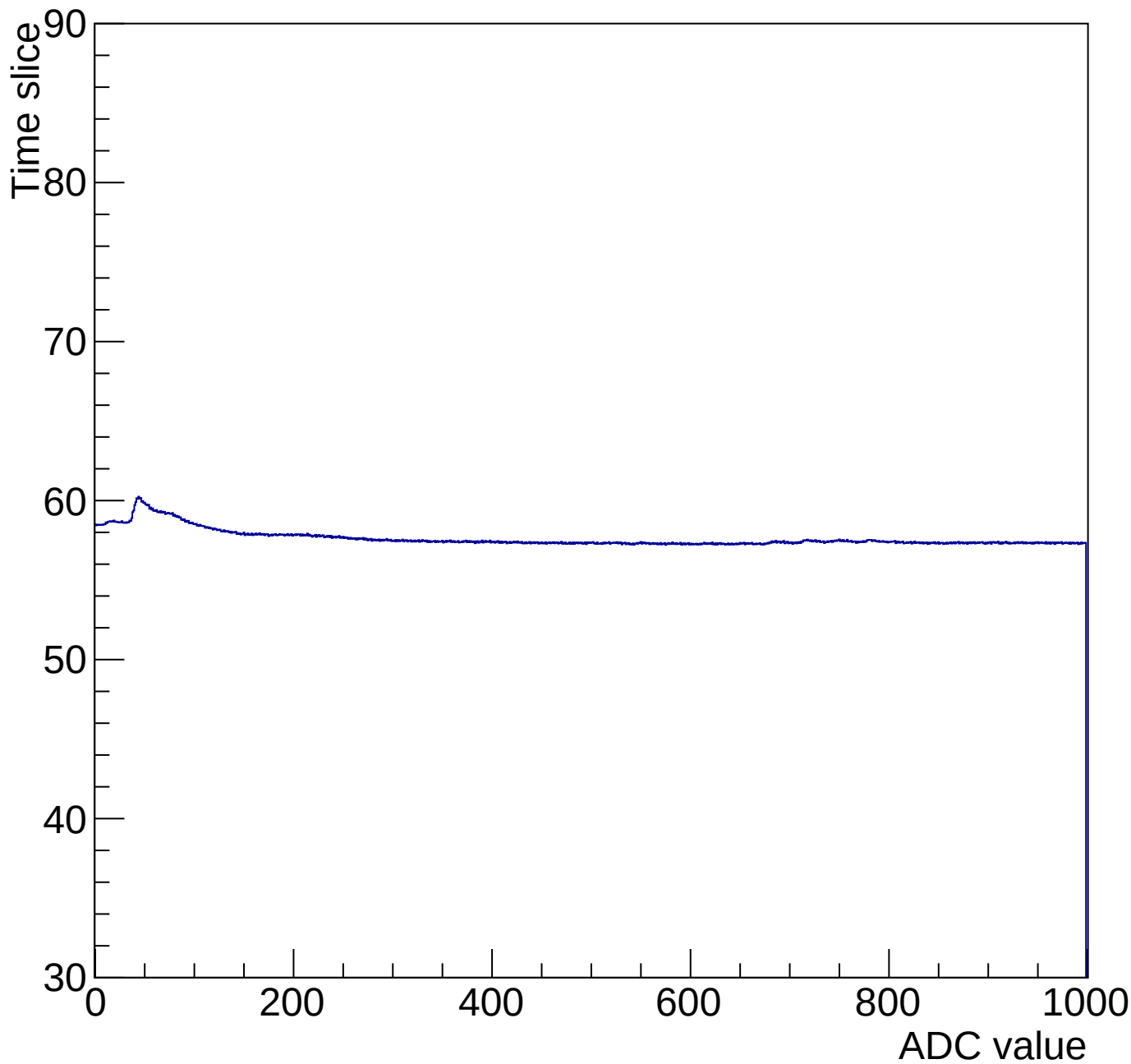
Time mcm 2004 chip 4 chan 13 1000-gain0-shaper0
