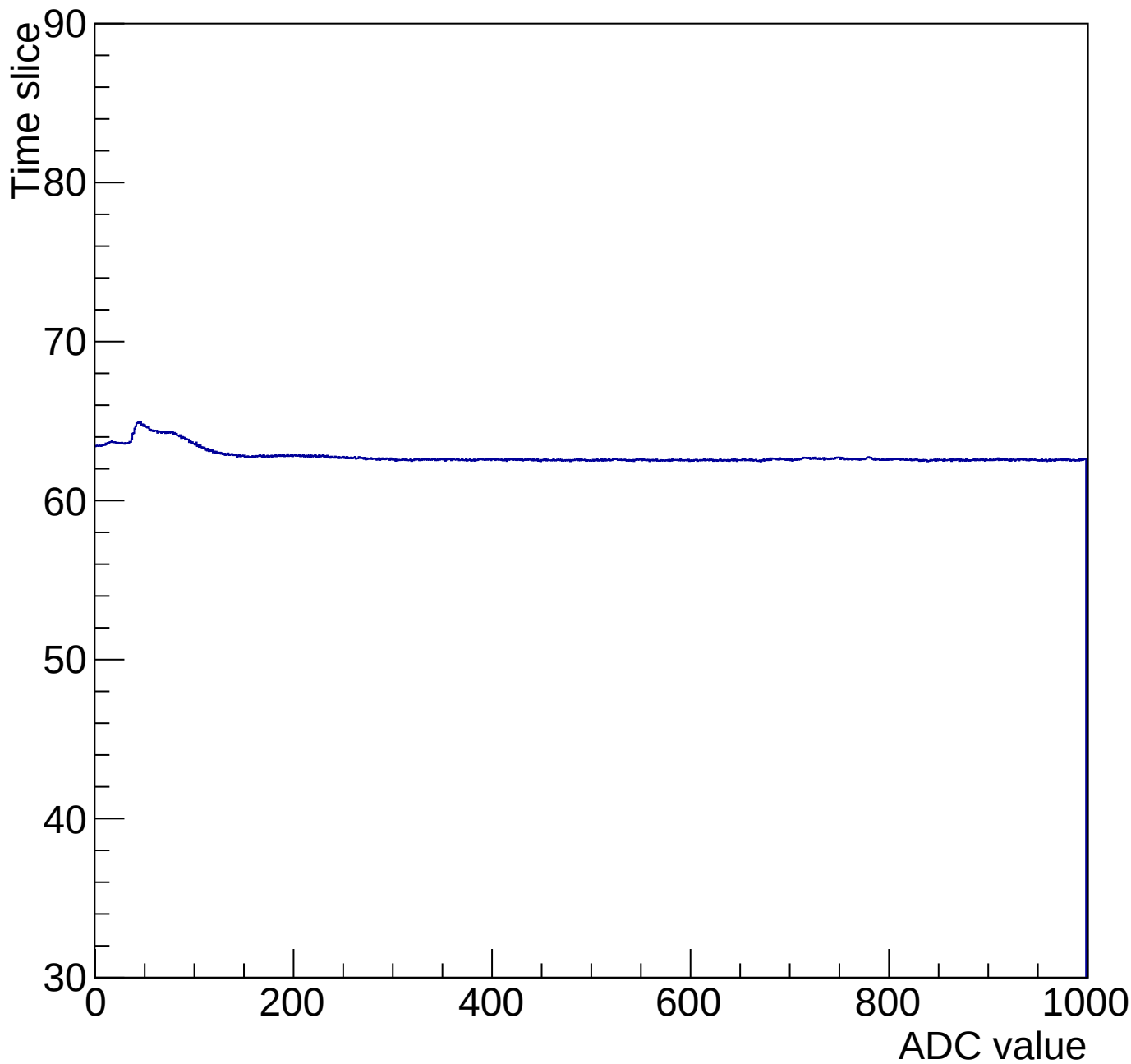
Time mcm 2004 chip 4 chan 14 1000-gain0-shaper0
