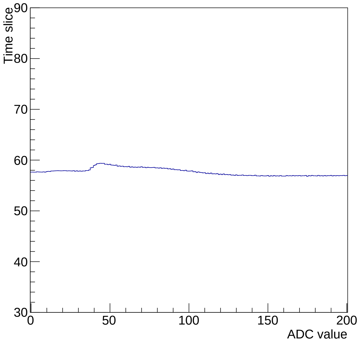
Time mcm 2004 chip 4 chan 8 200-gain0-shaper0
