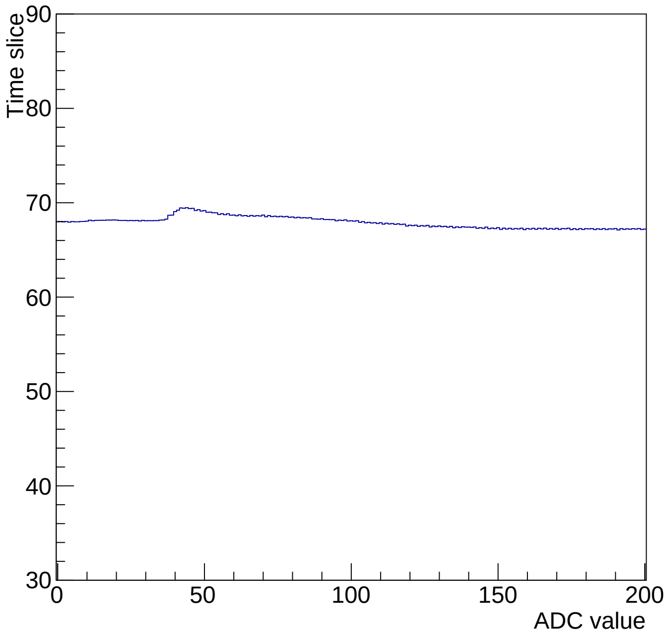
Time mcm 2004 chip 4 chan 11 200-gain0-shaper0
