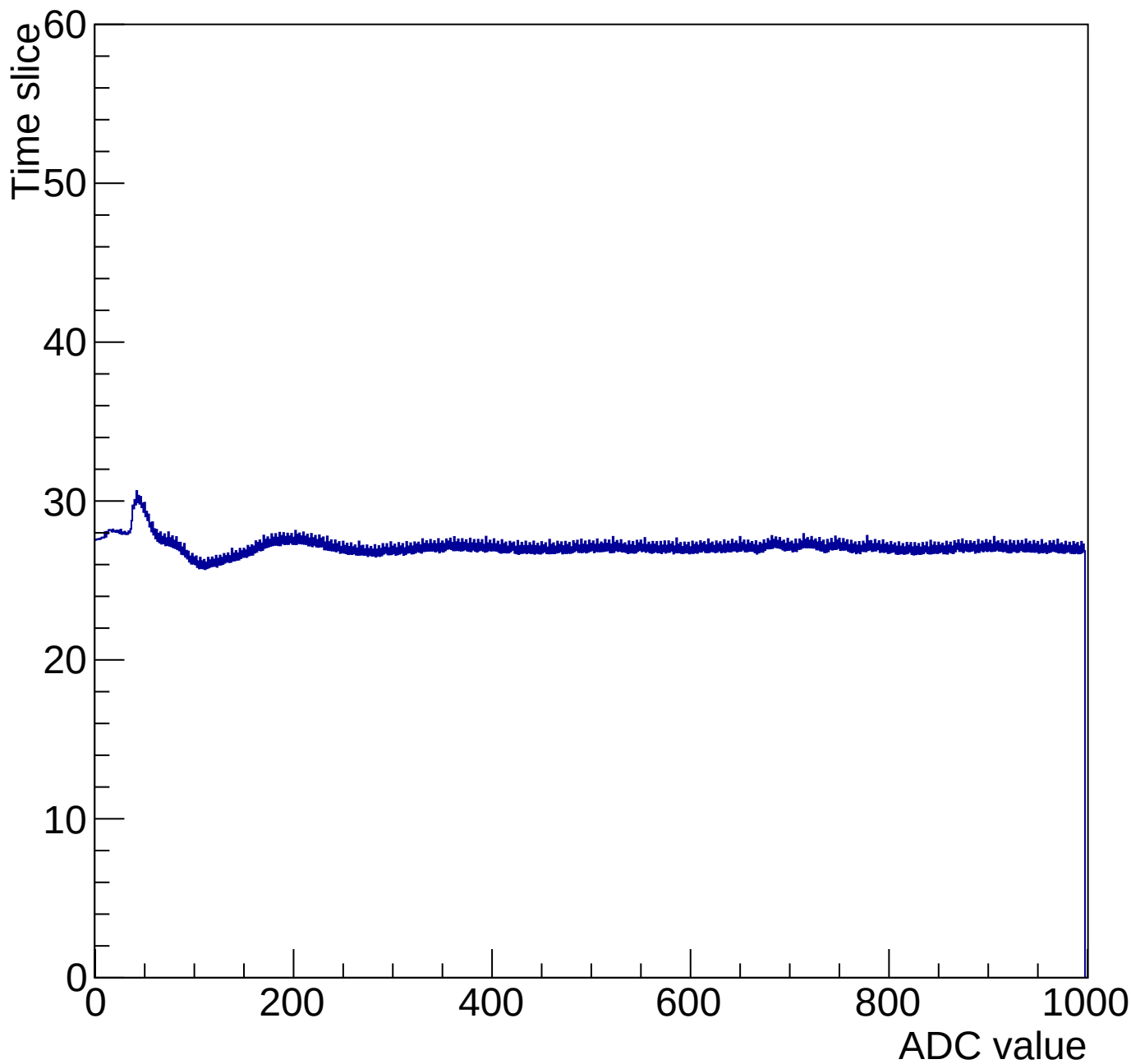
Time mcm 2005 chip 5 chan 2 1000-gain3-shaper0
