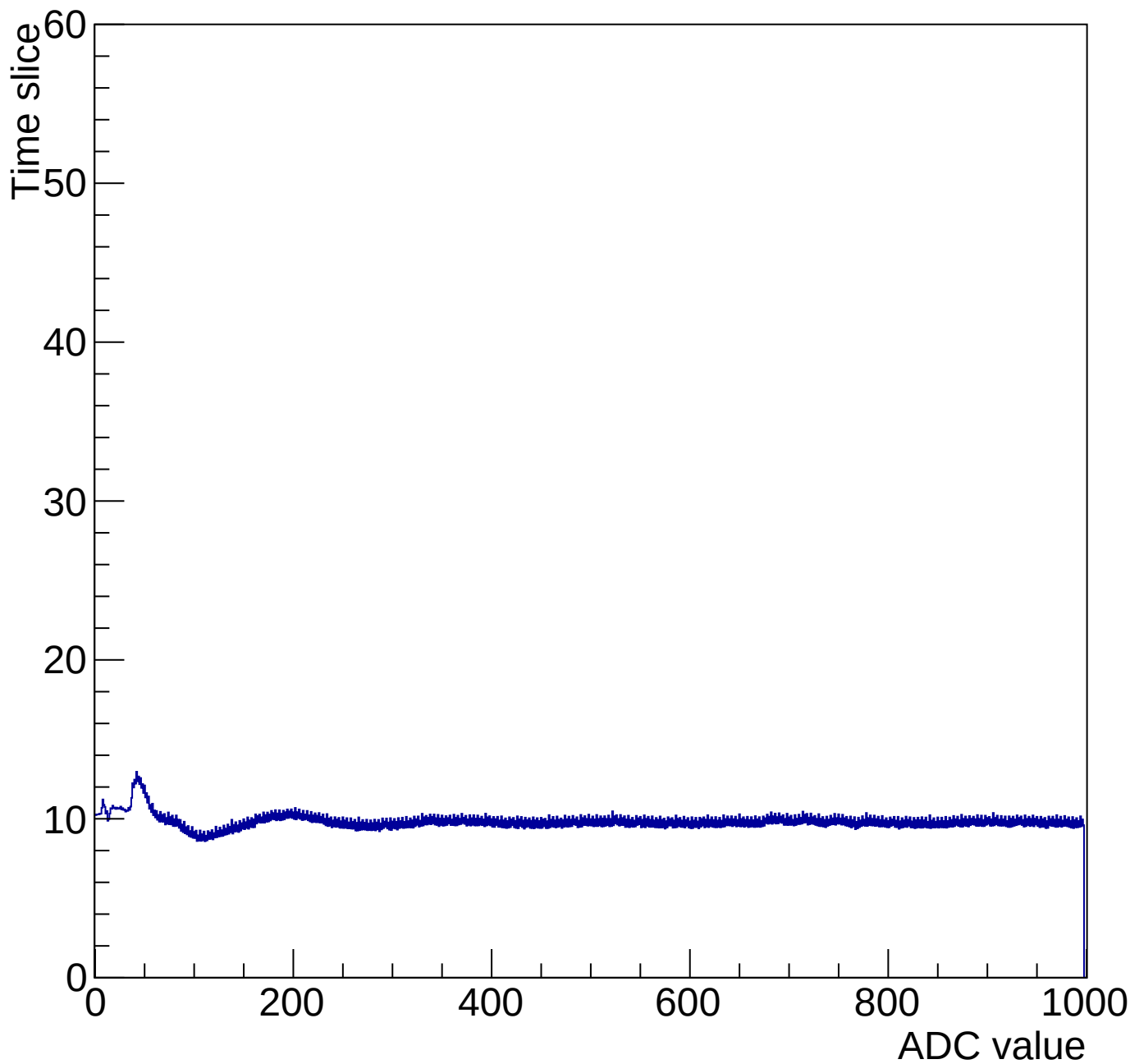
Time mcm 2005 chip 5 chan 15 1000-gain3-shaper0
