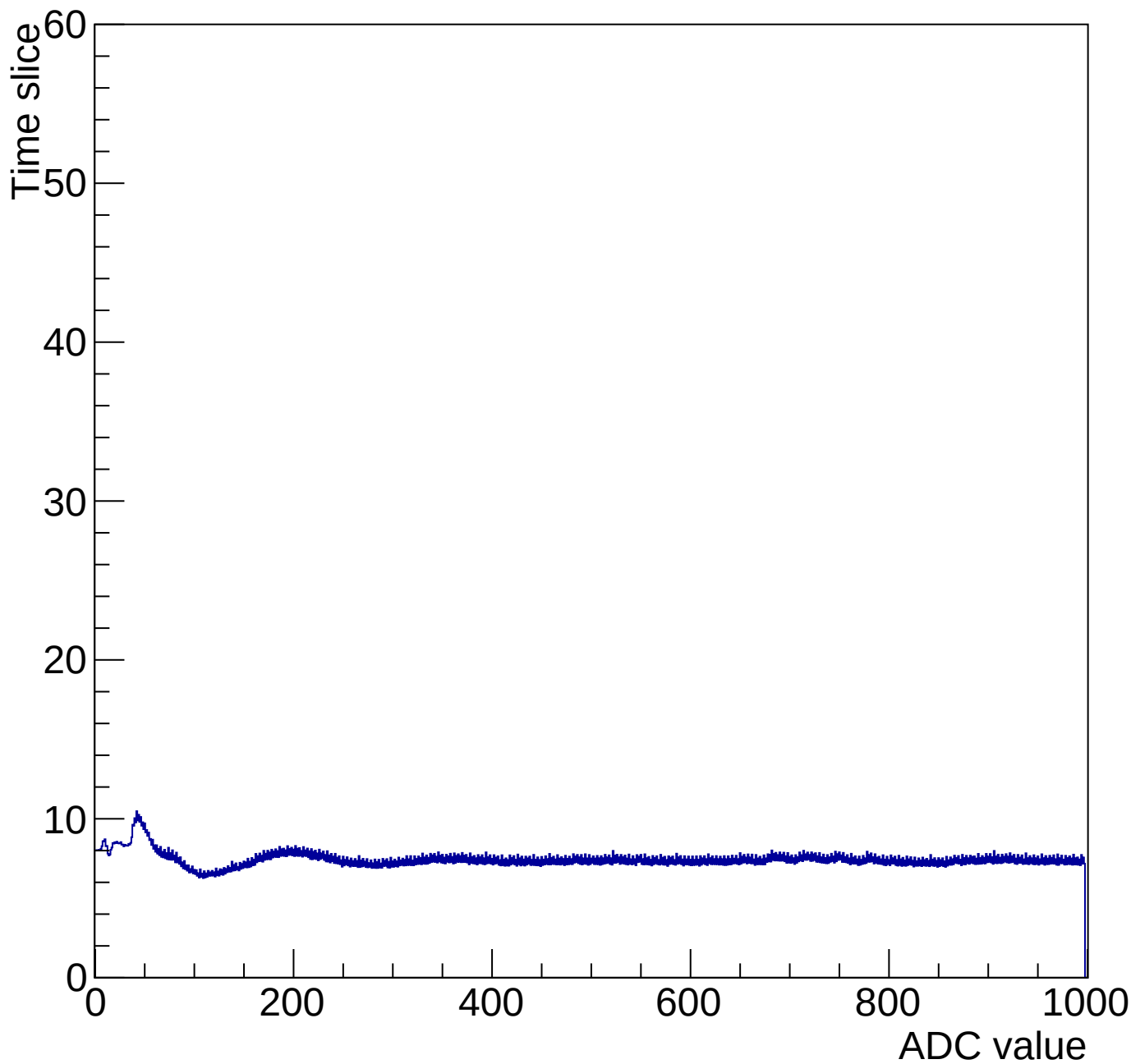
Time mcm 2005 chip 5 chan 13 1000-gain3-shaper0
