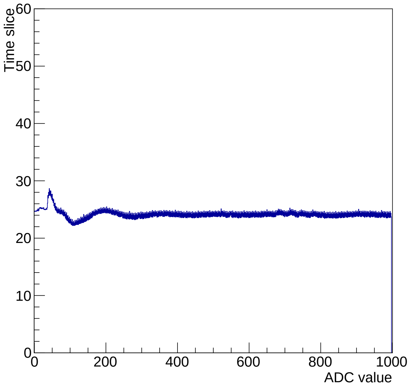
Time mcm 2005 chip 5 chan 0 1000-gain3-shaper0
