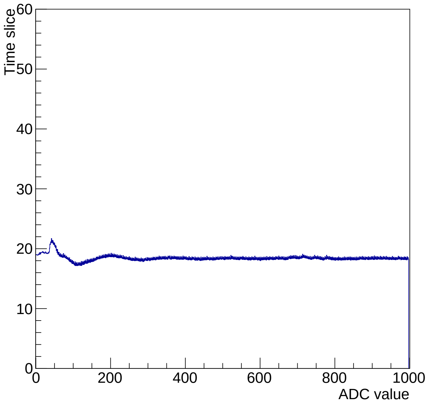
Time mcm 2005 chip 5 chan 14 1000-gain3-shaper0
