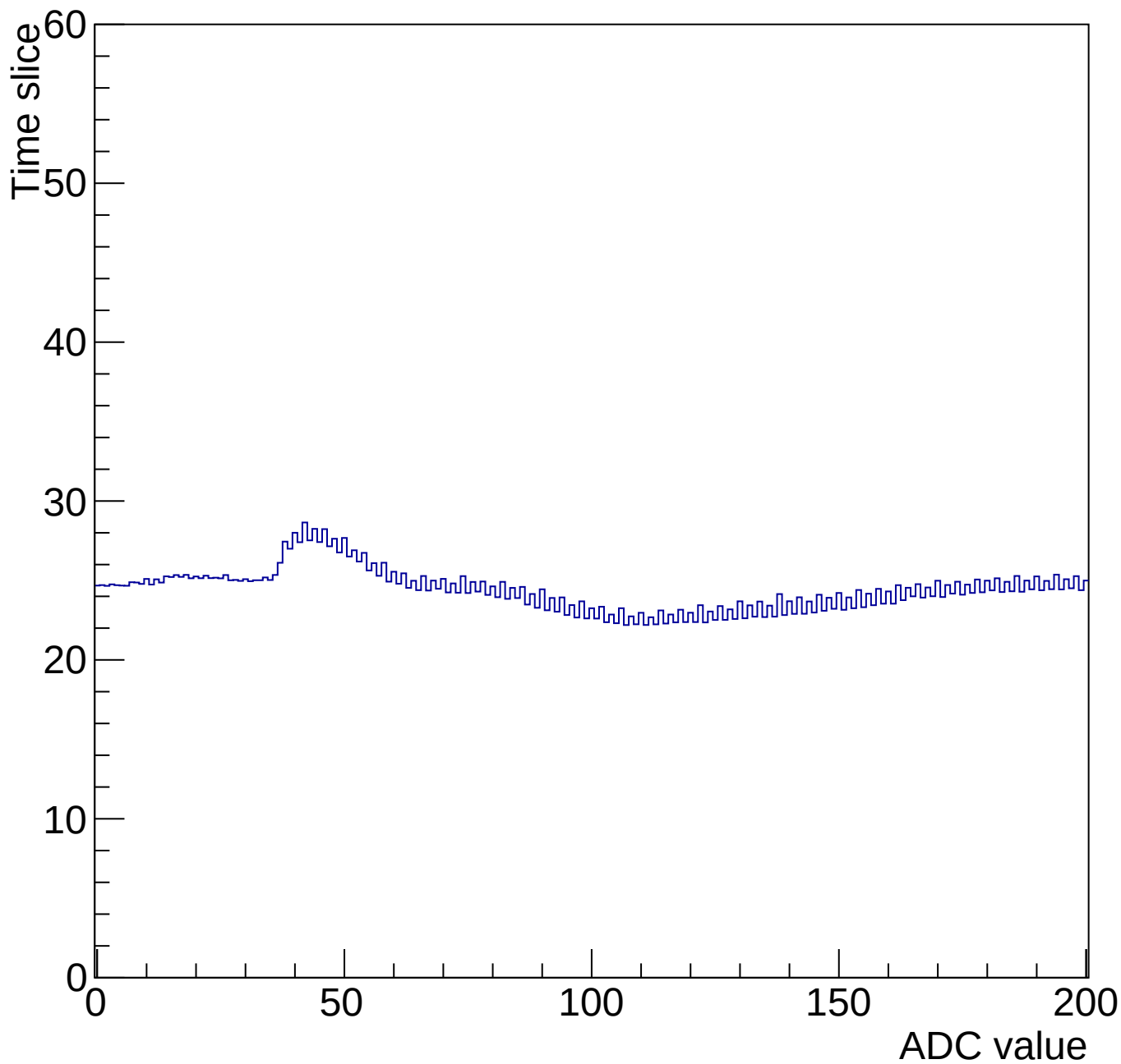
Time mcm 2005 chip 5 chan 0 200-gain3-shaper0
