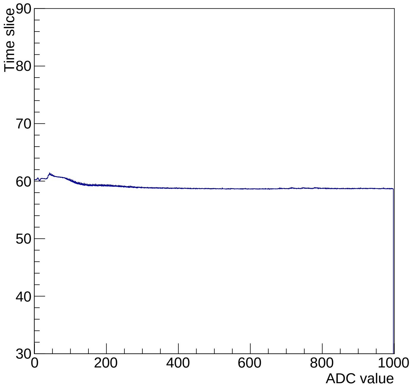
Time mcm 2005 chip 5 chan 11 1000-gain0-shaper0
