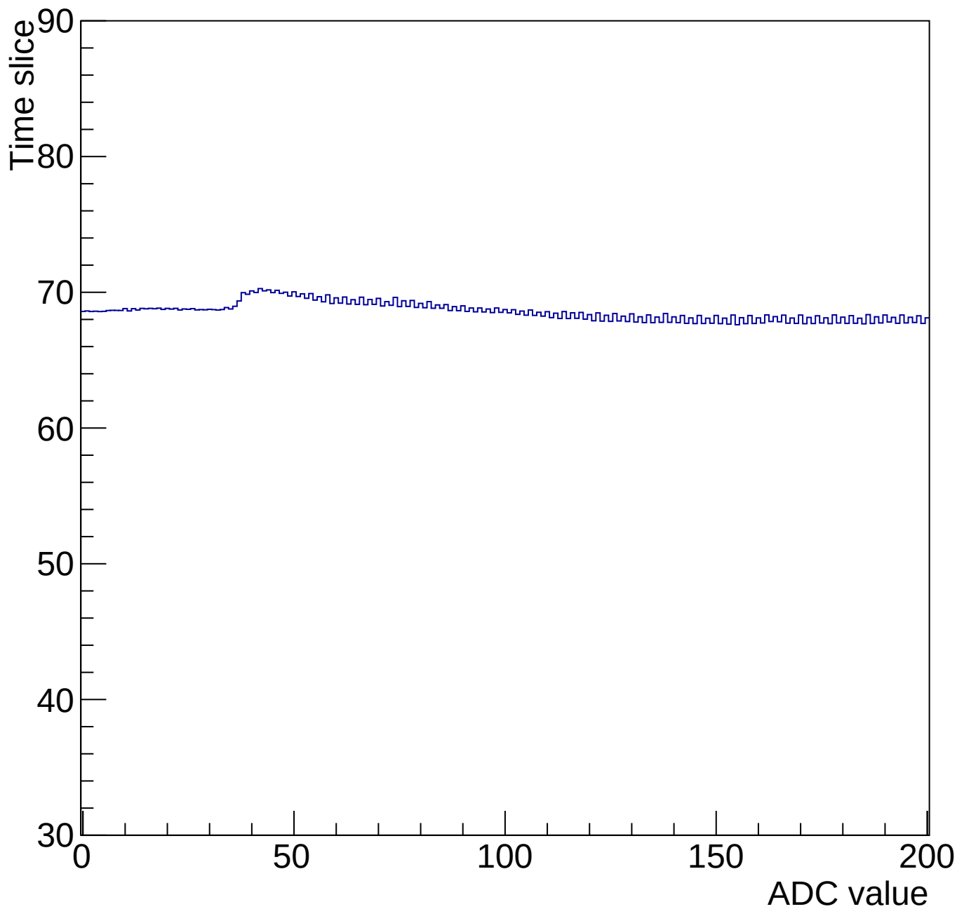
Time mcm 2005 chip 5 chan 0 200-gain0-shaper0
