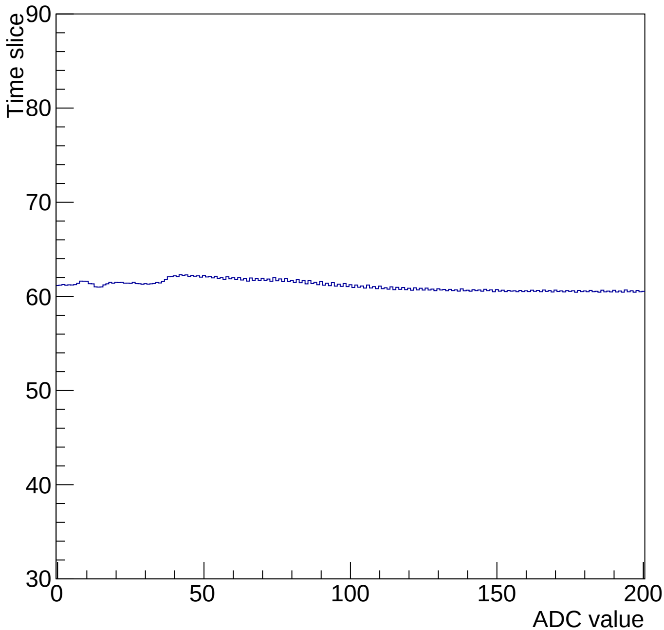
Time mcm 2005 chip 5 chan 9 200-gain0-shaper0
