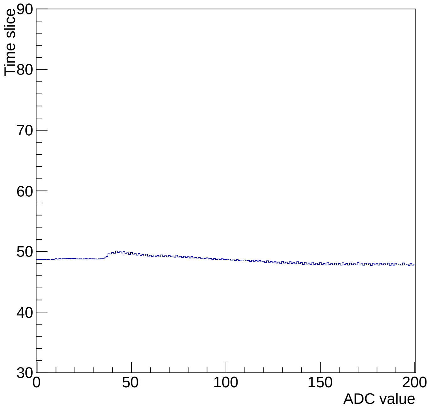
Time mcm 2005 chip 5 chan 12 200-gain0-shaper0
