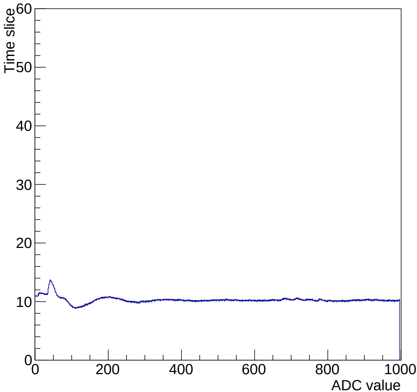
Time mcm 2006 chip 6 chan 12 1000-gain3-shaper0
