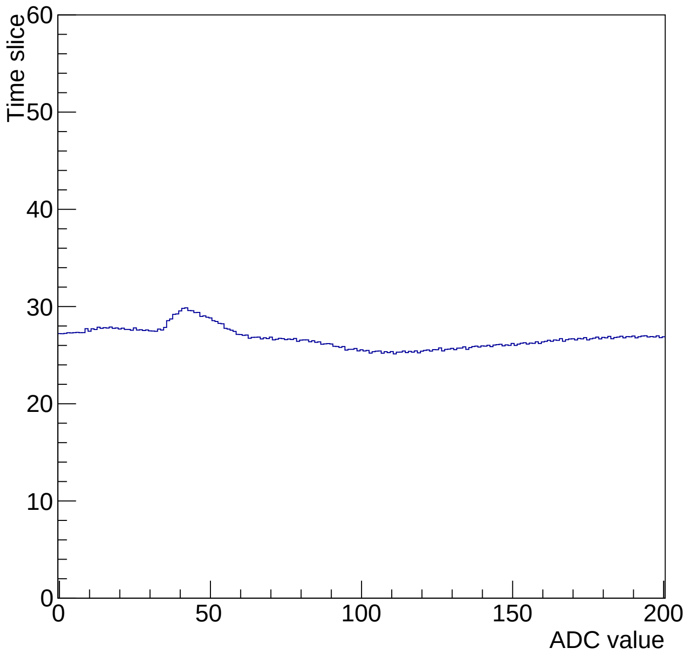
Time mcm 2006 chip 6 chan 5 200-gain3-shaper0
