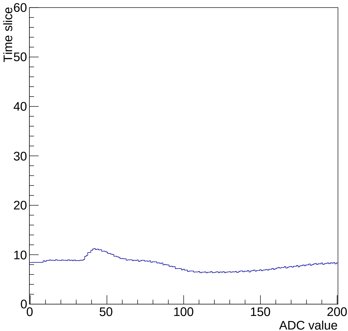
Time mcm 2006 chip 6 chan 6 200-gain3-shaper0
