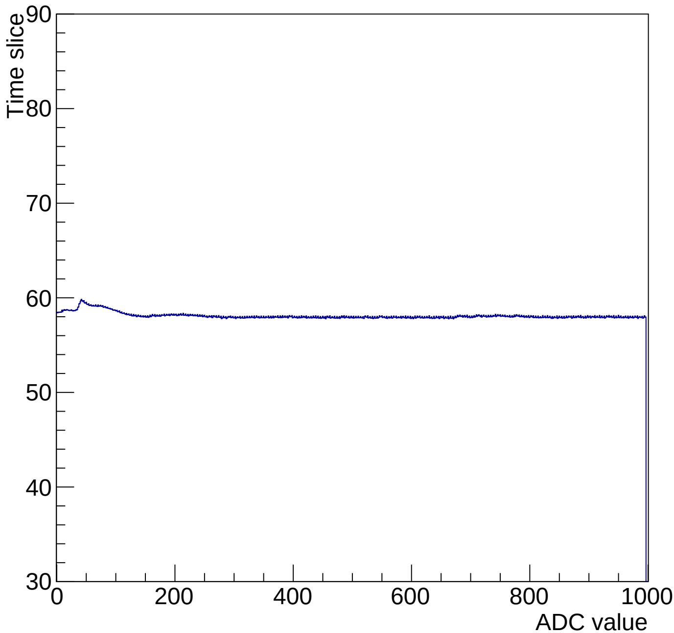
Time mcm 2006 chip 6 chan 12 1000-gain0-shaper0
