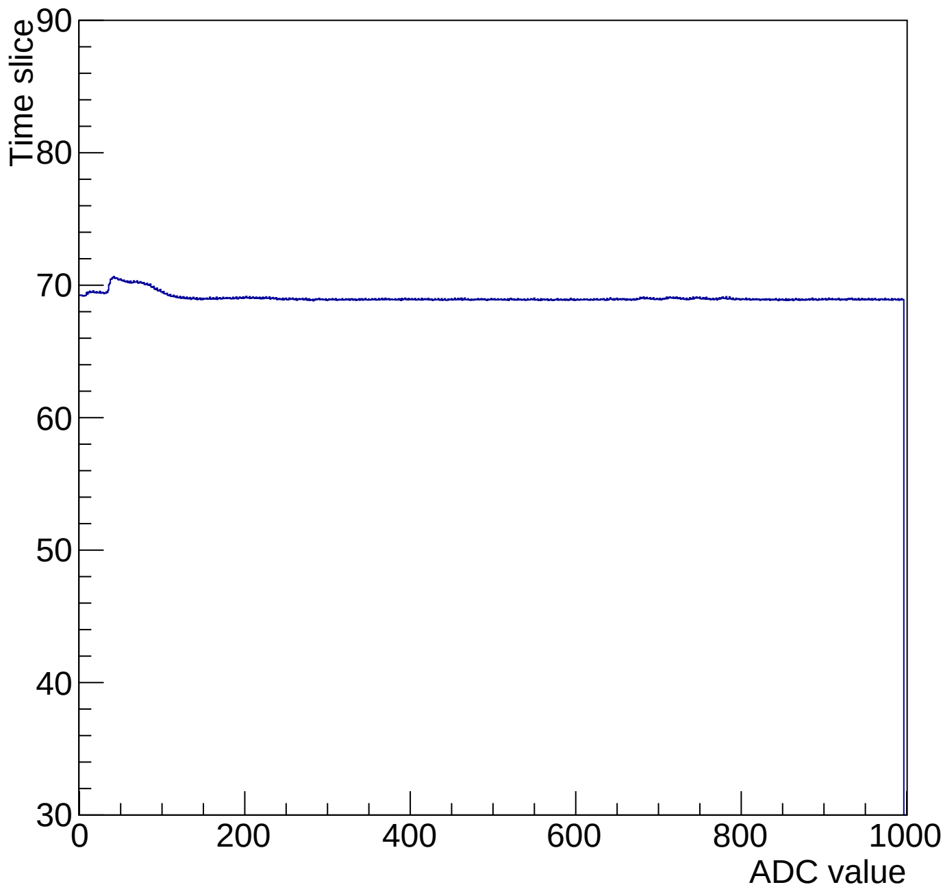
Time mcm 2006 chip 6 chan 5 1000-gain0-shaper0
