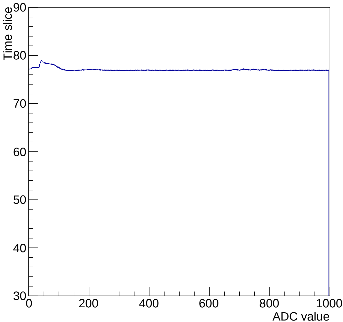
Time mcm 2006 chip 6 chan 0 1000-gain0-shaper0
