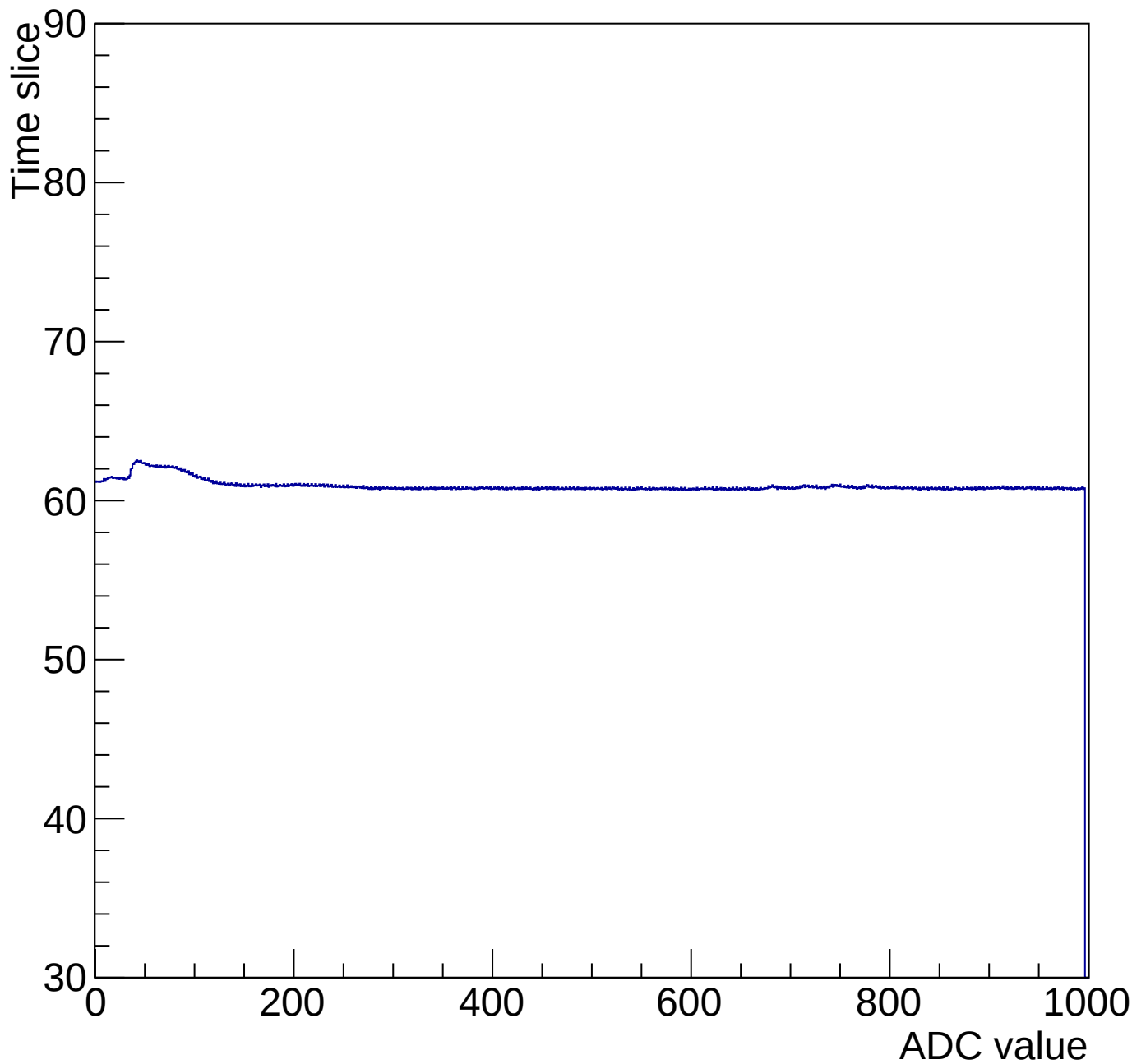
Time mcm 2006 chip 6 chan 2 1000-gain0-shaper0
