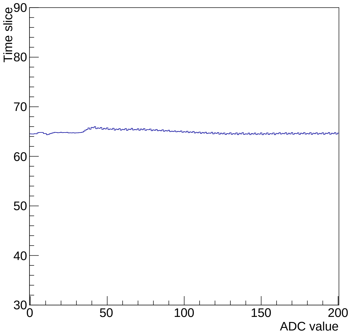
Time mcm 2007 chip 7 chan 1 200-gain0-shaper0
