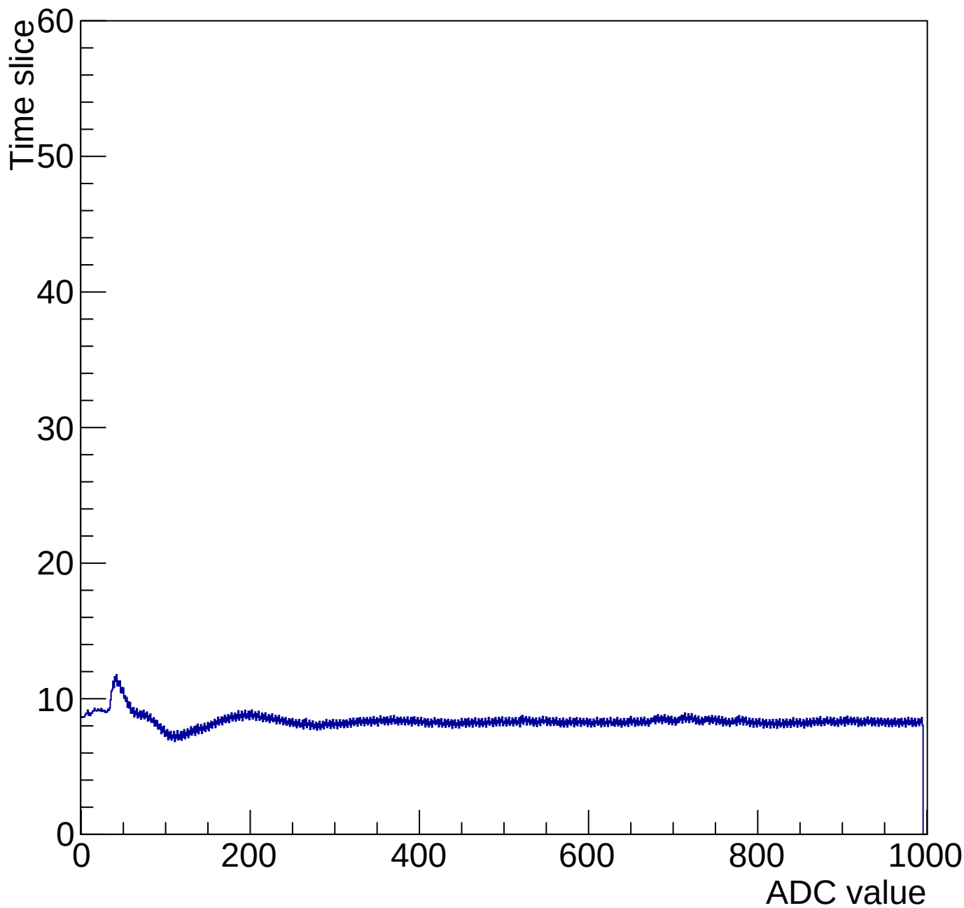
Time mcm 2007 chip 7 chan 2 1000-gain3-shaper0
