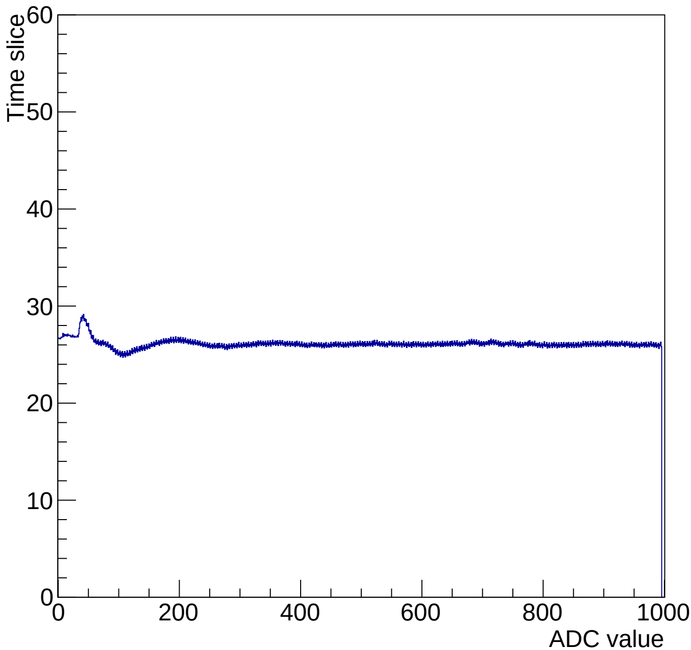
Time mcm 2007 chip 7 chan 13 1000-gain3-shaper0
